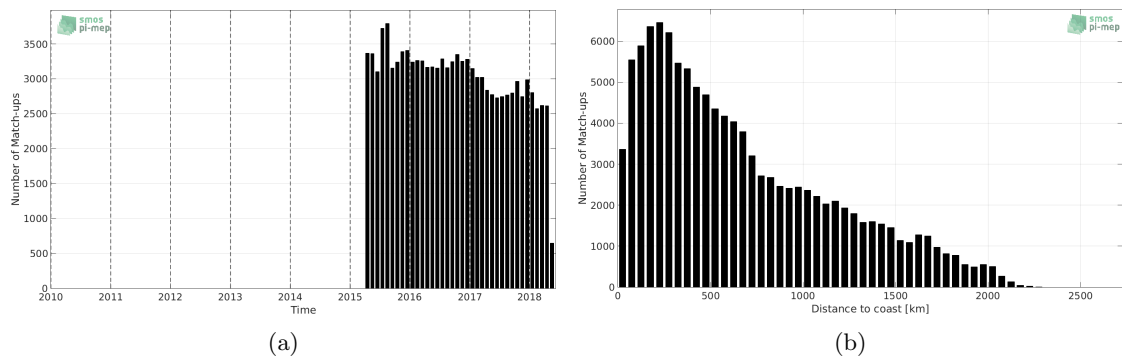
Figure 1: Number of match-ups between Argo and SMAP-L3-JPL-V4-8DAY-RUNNING-60KM SSS as a function of time (a) and as function of the distance to coast (b) over the North Pacific Ocean Pi-MEP region and for the full satellite product period.
