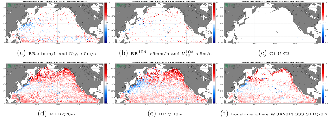
Figure 12: Temporal mean gridded over spatial boxes of size 1^\circ \times 1^\circ of \Delta\text{SSS} (SMAP-L3-JPL-V4-8DAY-RUNNING-60KM - Argo) for 6 different subdatasets corresponding to: \text{RR}>1\text{mm/h} and U_{10}<5\text{m/s} (a), \text{RR}^{10d}>5\text{mm/h} and U_{10}^{10d}<5\text{m/s} (b), C1 U C2 (c), \text{MLD}<20\text{m} (d), \text{BLT}>10\text{m} (e), Locations where WOA2013 SSS STD >0.2 (f).
