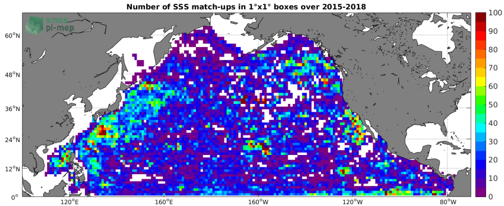
Figure 4: Number of SSS match-ups between Argo SSS and the SMAP-L3-JPL-V4-8DAY-RUNNING-60KM SSS product for the North Pacific Ocean Pi-MEP region over 1^\circ \times 1^\circ boxes and for the full satellite product period.
