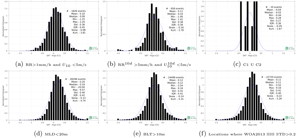
Figure 13: Normalized histogram of \Delta\text{SSS} (SMAP-L3-JPL-V4-8DAY-RUNNING-60KM - Argo) for 6 different subdatasets corresponding to: \text{RR}>1\text{mm/h} and U_{10}<5\text{m/s} (a), \text{RR}^{10d}>5\text{mm/h} and U_{10}^{10d}<5\text{m/s} (b), C1 U C2 (c), \text{MLD}<20\text{m} (d), \text{BLT}>10\text{m} (e), Locations where WOA2013 SSS STD >0.2 (f).
