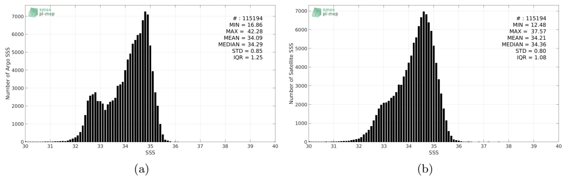
Figure 2: Histograms of SSS from Argo (a) and SMAP-L3-JPL-V4-8DAY-RUNNING-60KM (b) considering all match-up pairs per bins of 0.1 over the North Pacific Ocean Pi-MEP region and for the full satellite product period.
