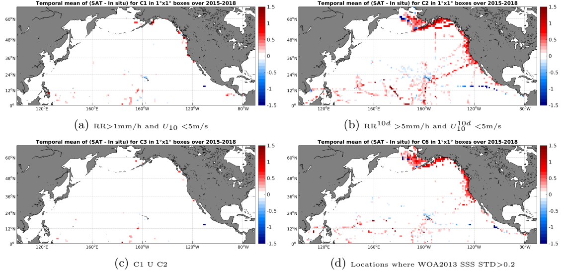
Figure 12: Temporal mean gridded over spatial boxes of size 1^\circ \times 1^\circ of \Delta SSS (SMAP-L3-JPL-V4-MONTHLY-60KM - TSG-SAMOS) for 4 different subdatasets corresponding to: RR > 1mm/h and U_{10} < 5 m/s (a), RR^{10d} > 5 mm/h and U_{10}^{10d} < 5 m/s (b), C1 U C2 (c), Locations where WOA2013 SSS STD > 0.2 (d).
