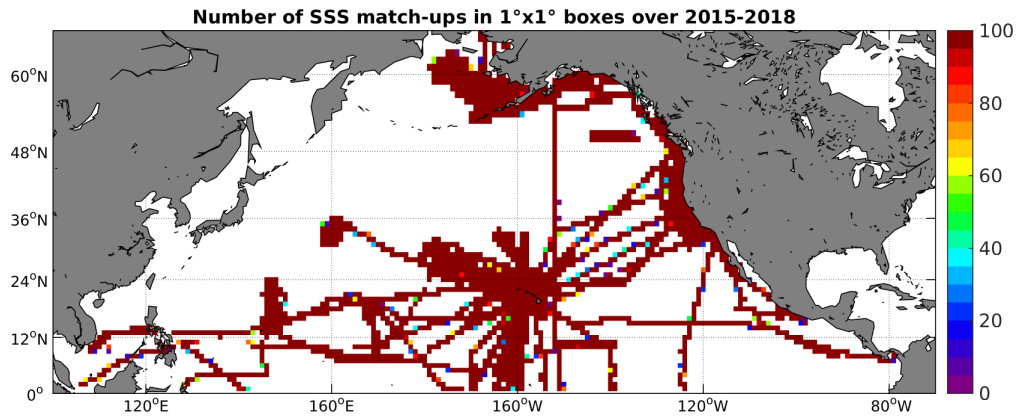
Figure 4: Number of SSS match-ups between TSG-SAMOS SSS and the SMAP-L3-JPL-V4-MONTHLY-60KM SSS product for the North Pacific Ocean Pi-MEP region over 1^\circ \times 1^\circ boxes and for the full satellite product period.
