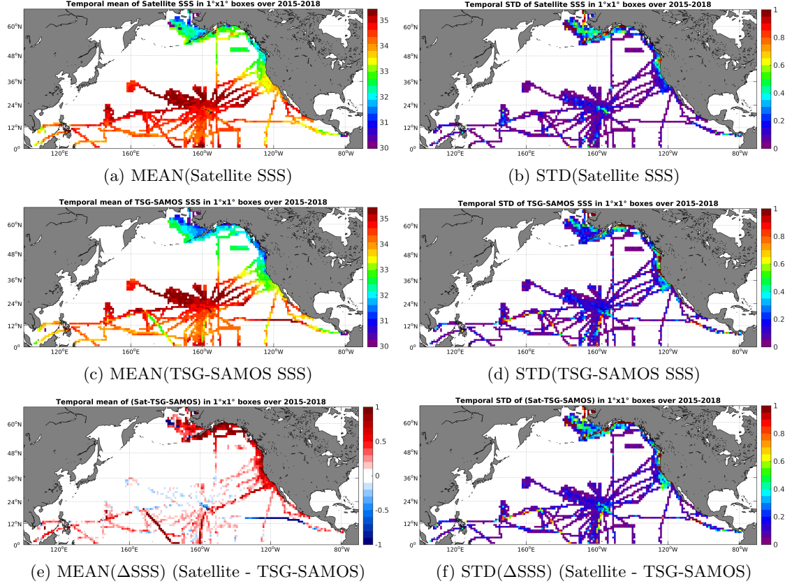
Figure 6: Temporal mean (left) and STD (right) of SSS from SMAP-L3-JPL-V4-MONTHLY-60KM (top), TSG-SAMOS (middle), and of \Delta SSS (Satellite - TSG-SAMOS). Only match-up pairs are used to generate these maps.
