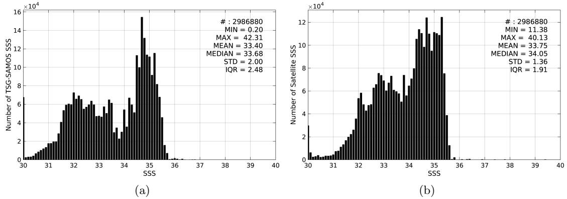
Figure 2: Histograms of SSS from TSG-SAMOS (a) and SMAP-L3-JPL-V4-MONTHLY-60KM (b) considering all match-up pairs per bins of 0.1 over the North Pacific Ocean Pi-MEP region and for the full satellite product period.
