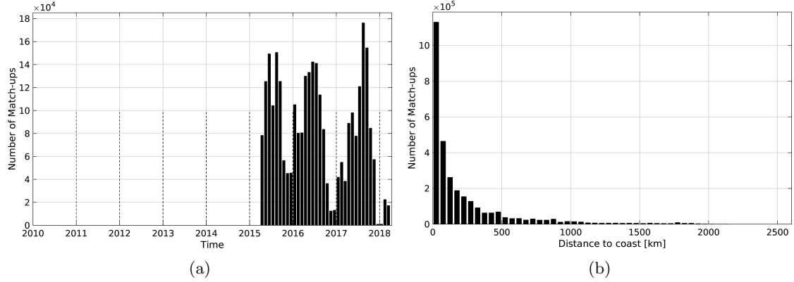
Figure 1: Number of match-ups between TSG-SAMOS and SMAP-L3-JPL-V4-MONTHLY-60KM SSS as a function of time (a) and as function of the distance to coast (b) over the North Pacific Ocean Pi-MEP region and for the full satellite product period.
