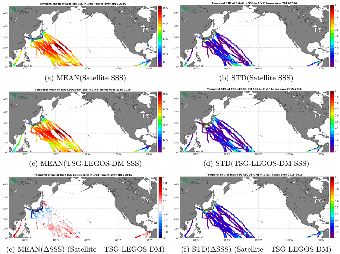
Figure 6: Temporal mean (left) and STD (right) of SSS from SMAP-L3-JPL-V4-MONTHLY-60KM (top), TSG-LEGOS-DM (middle), and of \Delta SSS (Satellite - TSG-LEGOS-DM). Only match-up pairs are used to generate these maps.
