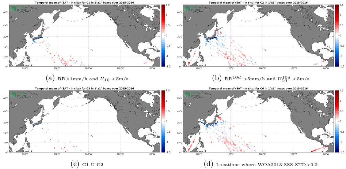
Figure 12: Temporal mean gridded over spatial boxes of size 1^\circ \times 1^\circ of \Delta SSS (SMAP-L3-JPL-V4-MONTHLY-60KM - TSG-LEGOS-DM) for 4 different subdatasets corresponding to: RR > 1mm/h and U_{10} < 5\text{m/s} (a), RR^{10d} > 5\text{mm/h} and U_{10}^{10d} < 5\text{m/s} (b), C1 U C2 (c), Locations where WOA2013 SSS STD > 0.2 (d).
