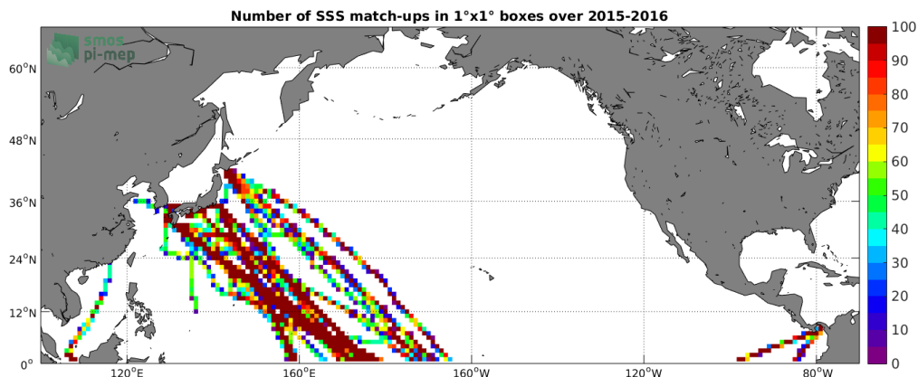
Figure 4: Number of SSS match-ups between TSG-LEGOS-DM SSS and the SMAP-L3-JPL-V4-MONTHLY-60KM SSS product for the North Pacific Ocean Pi-MEP region over 1^\circ \times 1^\circ boxes and for the full satellite product period.
