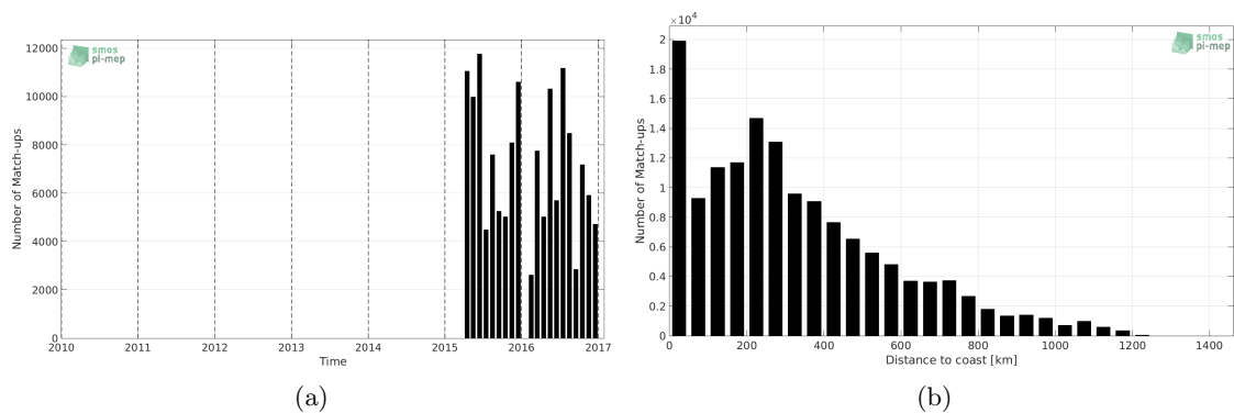
Figure 1: Number of match-ups between TSG-LEGOS-DM and SMAP-L3-JPL-V4-MONTHLY-60KM SSS as a function of time (a) and as function of the distance to coast (b) over the North Pacific Ocean Pi-MEP region and for the full satellite product period.
