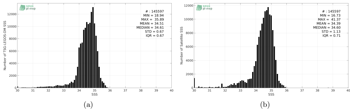
Figure 2: Histograms of SSS from TSG-LEGOS-DM (a) and SMAP-L3-JPL-V4-MONTHLY-60KM (b) considering all match-up pairs per bins of 0.1 over the North Pacific Ocean Pi-MEP region and for the full satellite product period.
