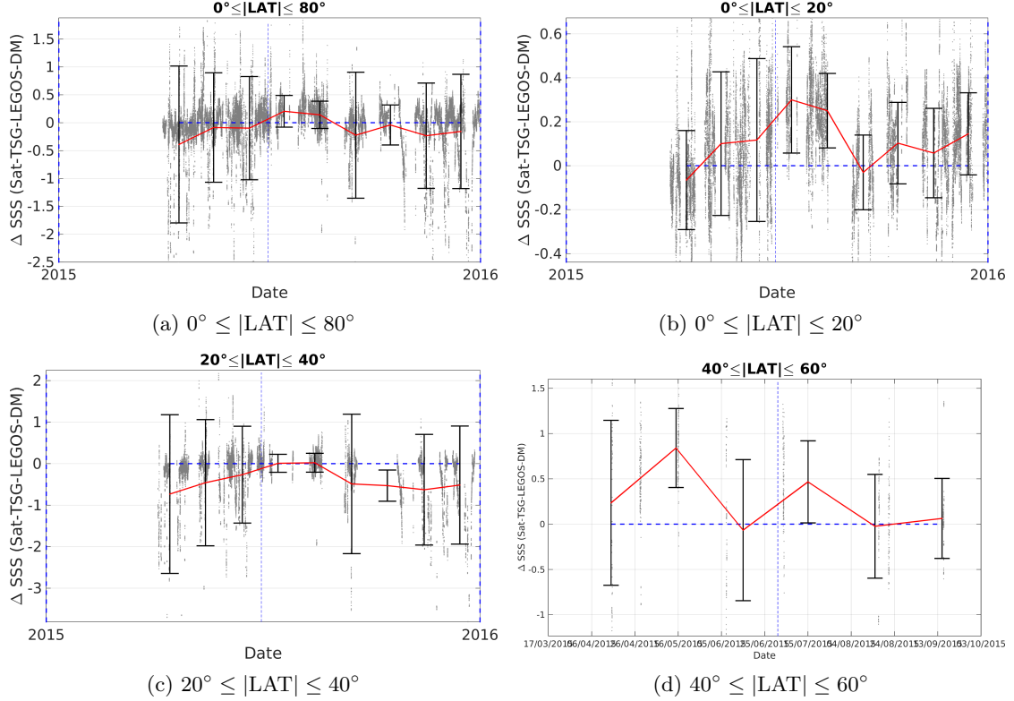
Figure 10: Monthly-averaged mean (red curves) \Delta SSS (Satellite - TSG-LEGOS-DM) and \pm 1 STD (black vertical thick bars) as function of time for all the collected Pi-MEP match-up pairs estimated over the North Pacific Ocean Pi-MEP region and for the full satellite product period are shown for different latitude bands: (a) Latitude band 80°S-80°N, (b) latitude band 20°S-20°N, (c) Mid Latitude bands 40°S-20°S and 20°N-40°N and (d) Latitude bands 60°S-40°S and 40°N-60°N.
