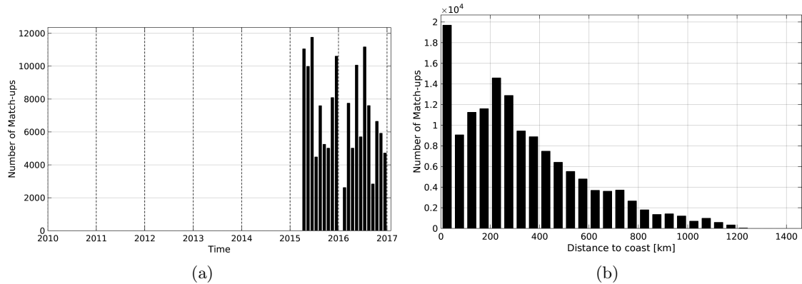
Figure 1: Number of match-ups between TSG-LEGOS-DM and SMAP-L3-JPL-V4-MONTHLY-60KM SSS as a function of time (a) and as function of the distance to coast (b) over the North Pacific Ocean Pi-MEP region and for the full satellite product period.
