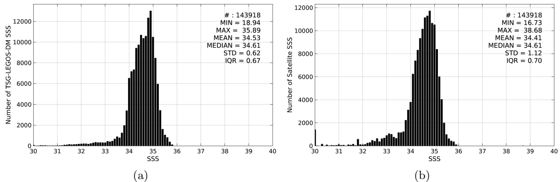
Figure 2: Histograms of SSS from TSG-LEGOS-DM (a) and SMAP-L3-JPL-V4-MONTHLY-60KM (b) considering all match-up pairs per bins of 0.1 over the North Pacific Ocean Pi-MEP region and for the full satellite product period.
