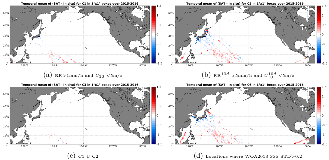
Figure 12: Temporal mean gridded over spatial boxes of size 1^\circ \times 1^\circ of \Delta SSS (SMAP-L3-JPL-V4-MONTHLY-60KM - TSG-LEGOS-DM) for 4 different subdatasets corresponding to: RR > 1\text{mm/h} and U_{10} < 5\text{m/s} (a), RR^{10d} > 5\text{mm/h} and U_{10}^{10d} < 5\text{m/s} (b), C1 U C2 (c), Locations where WOA2013 SSS STD > 0.2 (d).
