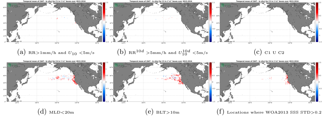
Figure 12: Temporal mean gridded over spatial boxes of size 1^\circ \times 1^\circ of \Delta\text{SSS} (SMAP-L3-JPL-V4-MONTHLY-60KM - Sea mammals) for 6 different subdatasets corresponding to: \text{RR}>1\text{mm/h} and U_{10}<5\text{m/s} (a), \text{RR}^{10d}>5\text{mm/h} and U_{10}^{10d}<5\text{m/s} (b), C1 U C2 (c), \text{MLD}<20\text{m} (d), \text{BLT}>10\text{m} (e), Locations where WOA2013 SSS STD >0.2 (f).
