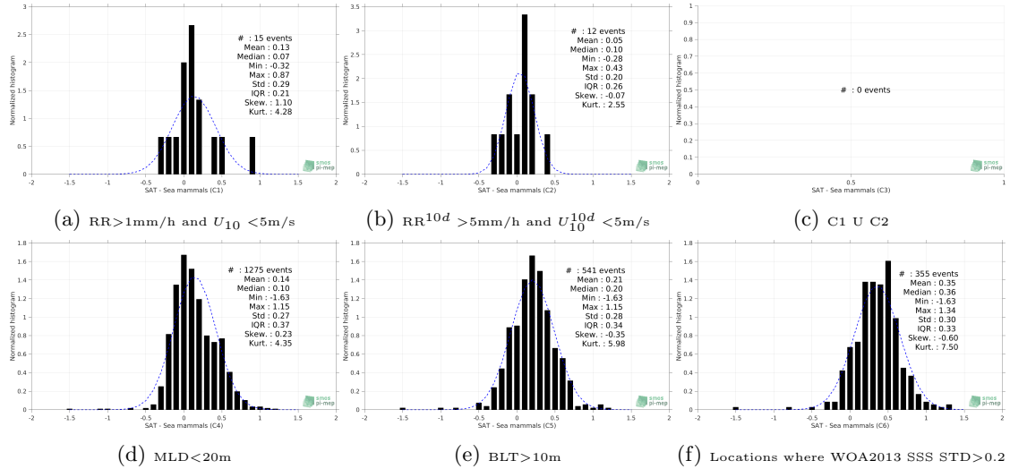
Figure 13: Normalized histogram of \Delta\text{SSS} (SMAP-L3-JPL-V4-MONTHLY-60KM - Sea mammals) for 6 different subdatasets corresponding to: \text{RR}>1\text{mm/h} and U_{10}<5\text{m/s} (a), \text{RR}^{10d}>5\text{mm/h} and U_{10}^{10d}<5\text{m/s} (b), C1 U C2 (c), \text{MLD}<20\text{m} (d), \text{BLT}>10\text{m} (e), Locations where WOA2013 SSS STD >0.2 (f).
