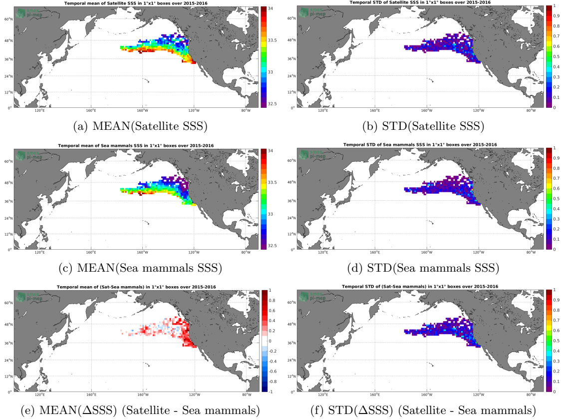
Figure 6: Temporal mean (left) and STD (right) of SSS from SMAP-L3-JPL-V4-MONTHLY-60KM (top), Sea mammals (middle), and of \Delta SSS (Satellite - Sea mammals). Only match-up pairs are used to generate these maps.
