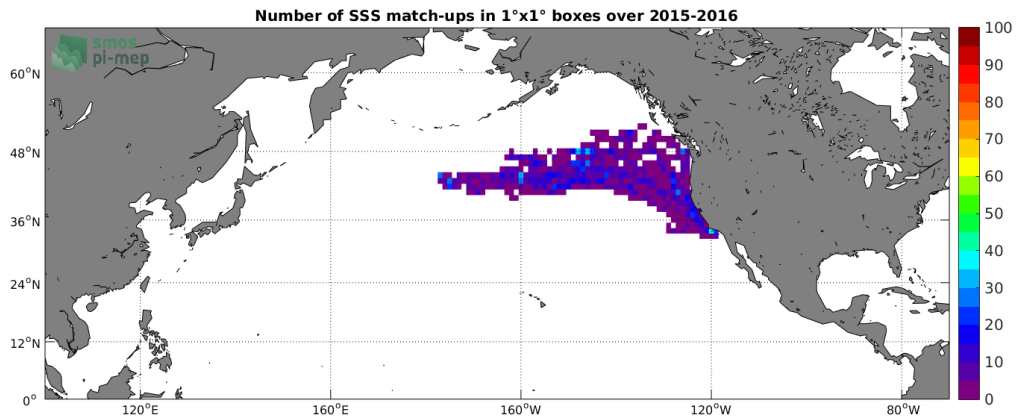
Figure 4: Number of SSS match-ups between Sea mammals SSS and the SMAP-L3-JPL-V4-MONTHLY-60KM SSS product for the North Pacific Ocean Pi-MEP region over 1^\circ \times 1^\circ boxes and for the full satellite product period.
