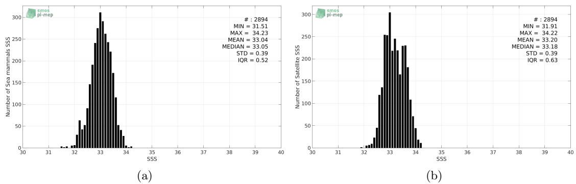
Figure 2: Histograms of SSS from Sea mammals (a) and SMAP-L3-JPL-V4-MONTHLY-60KM (b) considering all match-up pairs per bins of 0.1 over the North Pacific Ocean Pi-MEP region and for the full satellite product period.
