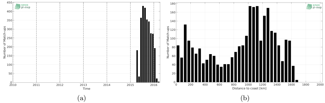
Figure 1: Number of match-ups between Sea mammals and SMAP-L3-JPL-V4-MONTHLY-60KM SSS as a function of time (a) and as function of the distance to coast (b) over the North Pacific Ocean Pi-MEP region and for the full satellite product period.
