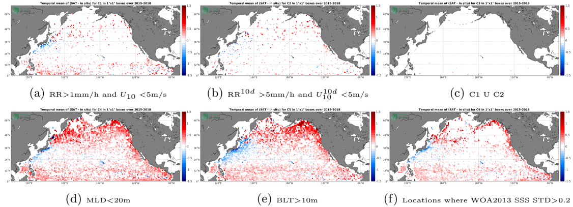
Figure 12: Temporal mean gridded over spatial boxes of size 1°x1° of \Delta SSS (SMAP-L3-JPL-V4-MONTHLY-60KM - Argo) for 6 different subdatasets corresponding to:RR>1mm/h and U_{10} < 5m/s (a), RR^{10d} > 5mm/h and U_{10}^{10d} < 5m/s (b), C1 U C2 (c),MLD<20m (d),BLT>10m (e),Locations where WOA2013 SSS STD>0.2 (f).
