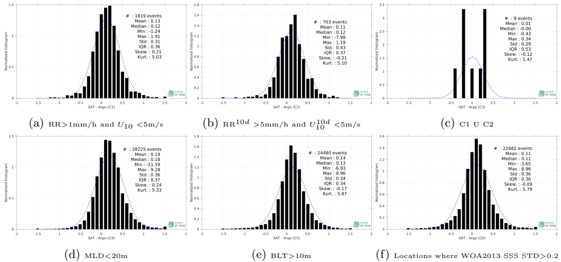
Figure 13: Normalized histogram of \Delta SSS (SMAP-L3-JPL-V4-MONTHLY-60KM - Argo) for 6 different subdatasets corresponding to: RR>1mm/h and U_{10} < 5m/s (a), RR^{10d} > 5mm/h and U_{10}^{10d} < 5m/s (b), C1 U C2 (c),MLD<20m (d),BLT>10m (e),Locations where WOA2013 SSS STD>0.2 (f).
