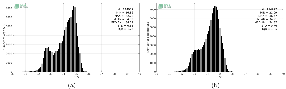
Figure 2: Histograms of SSS from Argo (a) and SMAP-L3-JPL-V4-MONTHLY-60KM (b) considering all match-up pairs per bins of 0.1 over the North Pacific Ocean Pi-MEP region and for the full satellite product period.
