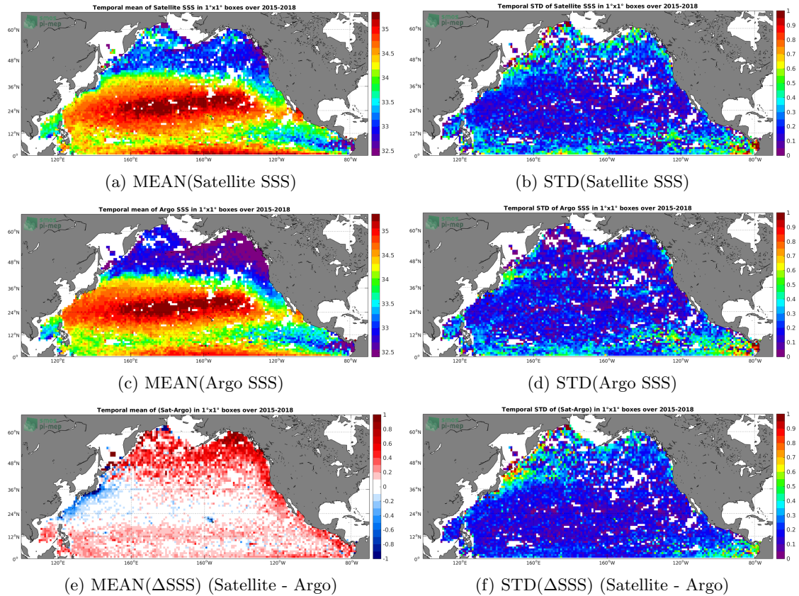
Figure 6: Temporal mean (left) and STD (right) of SSS from SMAP-L3-JPL-V4-MONTHLY-60KM (top), Argo (middle), and of \Delta SSS (Satellite - Argo). Only match-up pairs are used to generate these maps.
