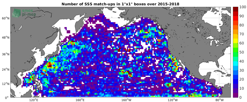
Figure 4: Number of SSS match-ups between Argo SSS and the SMAP-L3-JPL-V4-MONTHLY-60KM SSS product for the North Pacific Ocean Pi-MEP region over 1°x1° boxes and for the full satellite product period.
