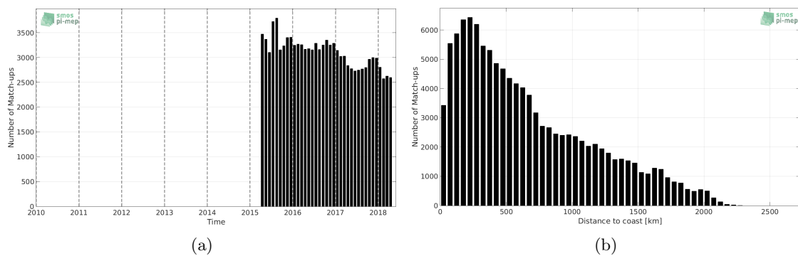
Figure 1: Number of match-ups between Argo and SMAP-L3-JPL-V4-MONTHLY-60KM SSS as a function of time (a) and as function of the distance to coast (b) over the North Pacific Ocean Pi-MEP region and for the full satellite product period.
