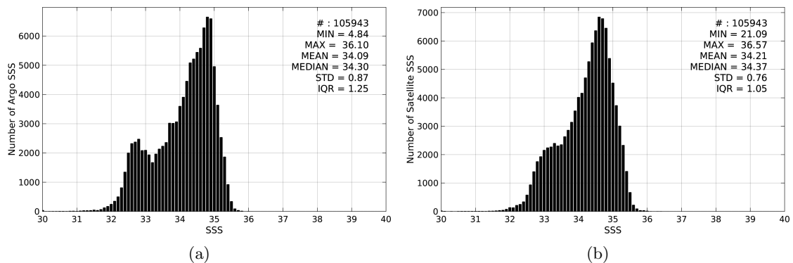
Figure 2: Histograms of SSS from Argo (a) and SMAP-L3-JPL-V4-MONTHLY-60KM (b) considering all match-up pairs per bins of 0.1 over the North Pacific Ocean Pi-MEP region and for the full satellite product period.
