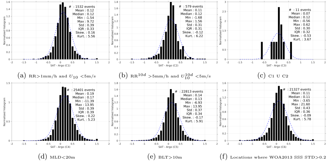
Figure 13: Normalized histogram of \Delta\text{SSS} (SMAP-L3-JPL-V4-MONTHLY-60KM - Argo) for 6 different subdatasets corresponding to: RR>1mm/h and U_{10} < 5\text{m/s} (a), RR^{10d} > 5\text{mm/h} and U_{10}^{10d} < 5\text{m/s} (b), C1 U C2 (c),MLD<20m (d),BLT>10m (e),Locations where WOA2013 SSS STD>0.2 (f).
