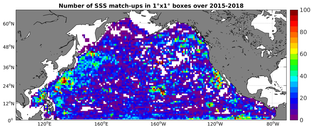
Figure 4: Number of SSS match-ups between Argo SSS and the SMAP-L3-JPL-V4-MONTHLY-60KM SSS product for the North Pacific Ocean Pi-MEP region over 1^\circ \times 1^\circ boxes and for the full satellite product period.
