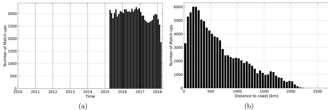
Figure 1: Number of match-ups between Argo and SMAP-L3-JPL-V4-MONTHLY-60KM SSS as a function of time (a) and as function of the distance to coast (b) over the North Pacific Ocean Pi-MEP region and for the full satellite product period.
