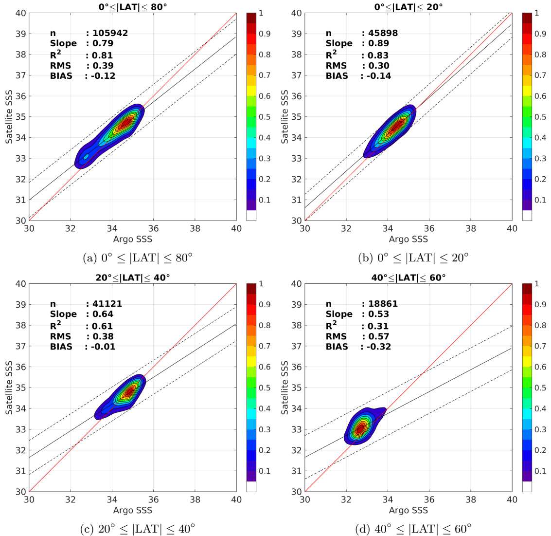
Figure 9: Contour maps of the concentration of SMAP-L3-JPL-V4-MONTHLY-60KM SSS (y-axis) versus Argo SSS (x-axis) at match-up pairs for different latitude bands. For each plot, the red line shows x=y . The black thin and dashed lines indicate a linear fit through the data cloud and the \pm 95\% confidence levels, respectively. The number match-up pairs n , the slope and R^2 coefficient of the linear fit, the root mean square (RMS) and the mean bias between satellite and in situ data are indicated for each latitude band in each plots.
