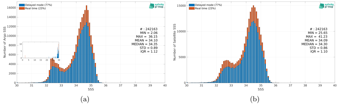
Figure 2: Histograms of SSS from Argo (a) and SMAP SSS L2-AVERAGED v5 (RSS) (b) considering all match-up pairs per bins of 0.1 over the North Pacific Ocean Pi-MEP region and for the full satellite product period.
