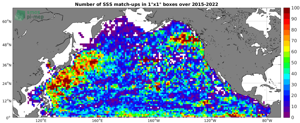
Figure 4: Number of SSS match-ups between Argo SSS and the SMAP SSS L2-AVERAGED v5 (RSS) SSS product for the North Pacific Ocean Pi-MEP region over 1^\circ \times 1^\circ boxes and for the full satellite product period.
