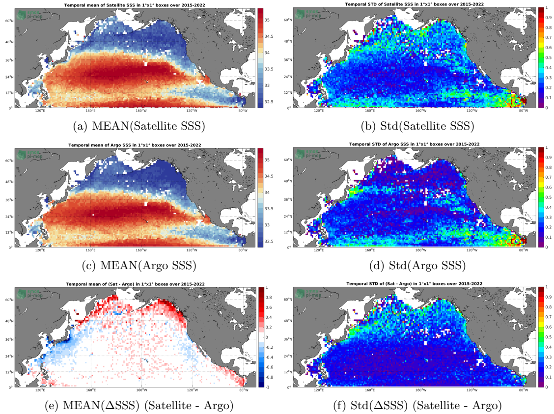
Figure 6: Temporal mean (left) and Std (right) of SSS from SMAP SSS L2-AVERAGED v5 (RSS) (top), Argo (middle), and of \Delta SSS (Satellite - Argo). Only match-up pairs are used to generate these maps.
