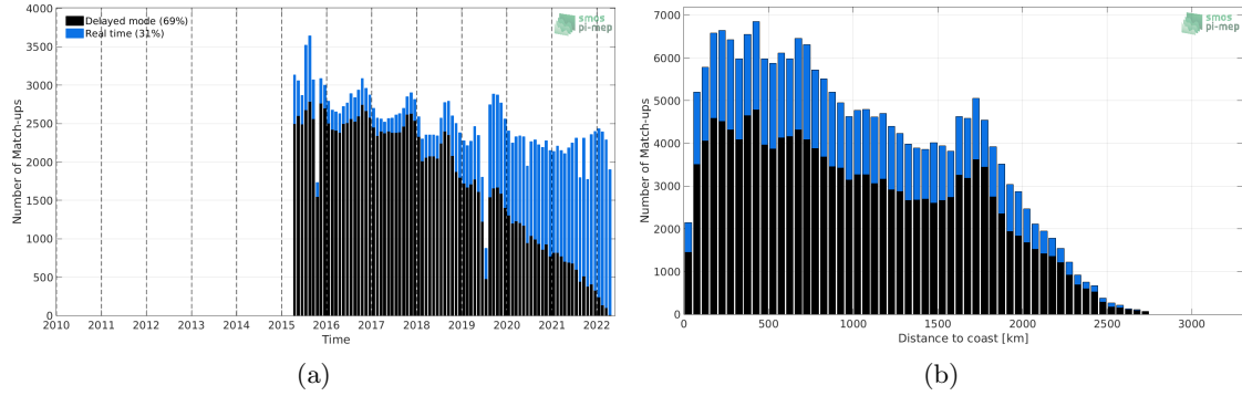
Figure 1: Number of match-ups between Argo and SMAP SSS L2-AVERAGED v5 (RSS) SSS as a function of time (a) and as function of the distance to coast (b) over the North Pacific Ocean Pi-MEP region and for the full satellite product period.
