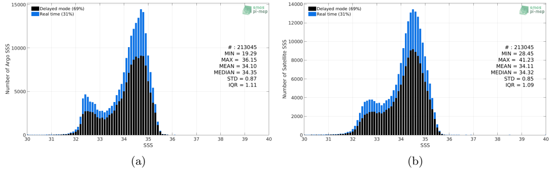
Figure 2: Histograms of SSS from Argo (a) and SMAP SSS L2-AVERAGED v5 (RSS) (b) considering all match-up pairs per bins of 0.1 over the North Pacific Ocean Pi-MEP region and for the full satellite product period.
