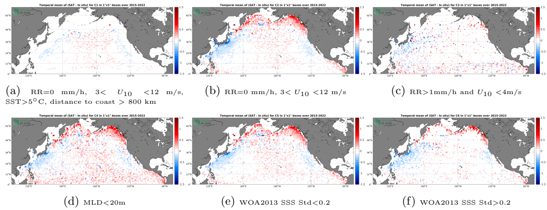
Figure 12: Temporal mean gridded over spatial boxes of size 1^\circ \times 1^\circ of \Delta SSS (SMAP SSS L2-AVERAGED v5 (RSS) - Argo) for 6 different subdatasets corresponding to:RR=0 mm/h, 3 < U_{10} < 12 m/s, SST >5^\circ C, distance to coast > 800 km (a), RR=0 mm/h, 3 < U_{10} < 12 m/s (b), RR >1 mm/h and U_{10} < 4 m/s (c),MLD <20 m (d),WOA2013 SSS Std <0.2 (e),WOA2013 SSS Std >0.2 (f).
