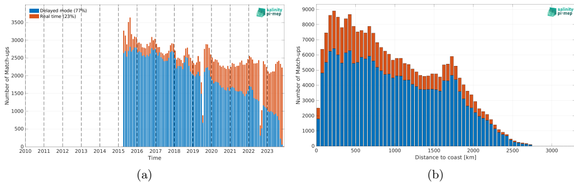
Figure 1: Number of match-ups between Argo and SMAP SSS L2-AVERAGED v5.0 (JPL) SSS as a function of time (a) and as function of the distance to coast (b) over the North Pacific Ocean Pi-MEP region and for the full satellite product period.
