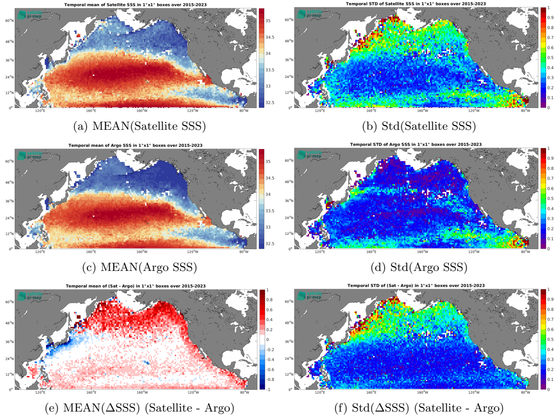
Figure 6: Temporal mean (left) and Std (right) of SSS from SMAP SSS L2-AVERAGED v5.0 (JPL) (top), Argo (middle), and of \Delta\text{SSS} (Satellite - Argo). Only match-up pairs are used to generate these maps.
