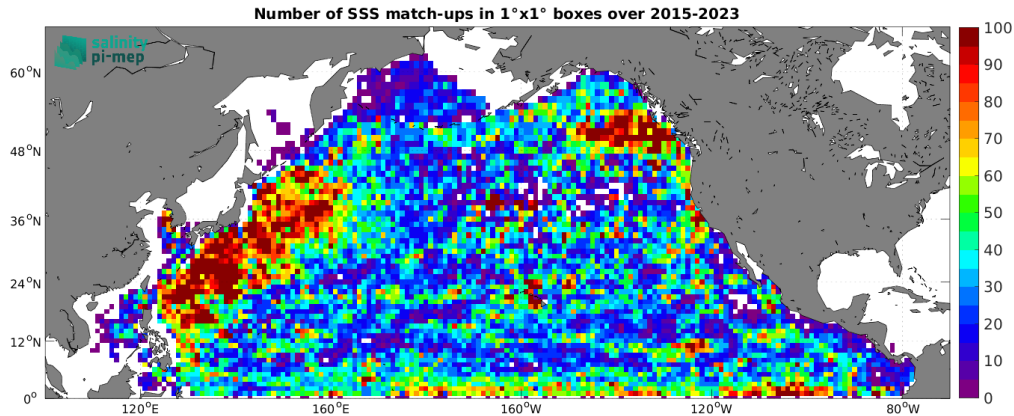
Figure 4: Number of SSS match-ups between Argo SSS and the SMAP SSS L2-AVERAGED v5.0 (JPL) SSS product for the North Pacific Ocean Pi-MEP region over 1^\circ \times 1^\circ boxes and for the full satellite product period.
