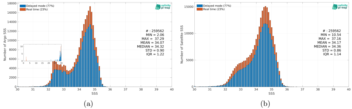
Figure 2: Histograms of SSS from Argo (a) and SMAP SSS L2-AVERAGED v5.0 (JPL) (b) considering all match-up pairs per bins of 0.1 over the North Pacific Ocean Pi-MEP region and for the full satellite product period.
