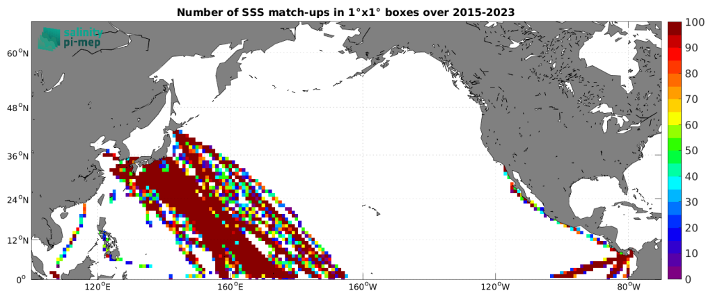
Figure 5: Number of SSS match-ups between TSG (LEGOS-DM) SSS and the SMAP SSS L2 v6 (RSS) SSS product for the North Pacific Ocean Pi-MEP region over 1^\circ \times 1^\circ boxes and for the full satellite product period.
