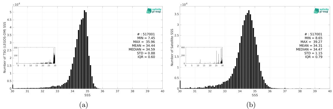
Figure 3: Histograms of SSS from TSG (LEGOS-DM) (a) and SMAP SSS L2 v6 (RSS) (b) considering all match-up pairs per bins of 0.1 over the North Pacific Ocean Pi-MEP region and for the full satellite product period.
