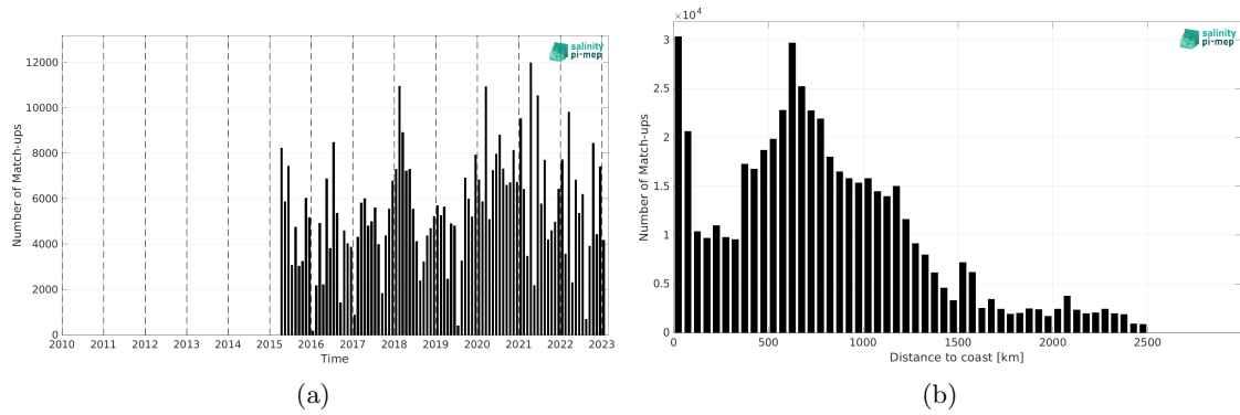
Figure 2: Number of match-ups between TSG (LEGOS-DM) and SMAP SSS L2 v6 (RSS) SSS as a function of time (a) and as function of the distance to coast (b) over the North Pacific Ocean Pi-MEP region and for the full satellite product period.
