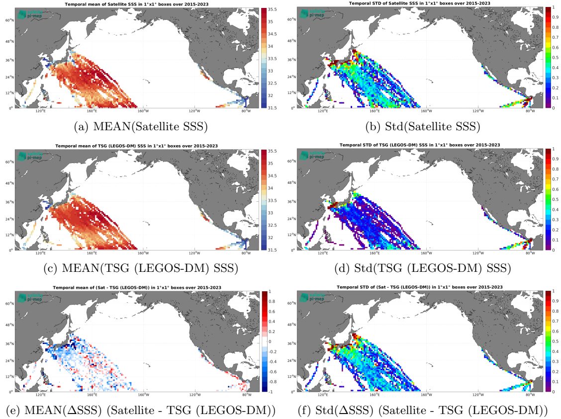
Figure 7: Temporal mean (left) and Std (right) of SSS from SMAP SSS L2 v6 (RSS) (top), TSG (LEGOS-DM) (middle), and of \Delta SSS (Satellite - TSG (LEGOS-DM)). Only match-up pairs are used to generate these maps.
