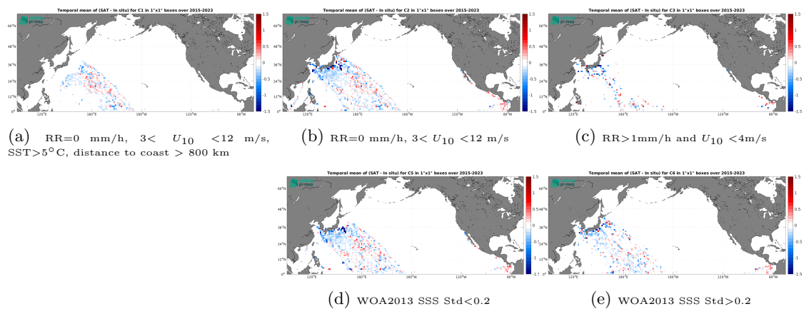
Figure 14: Temporal mean gridded over spatial boxes of size 1^\circ \times 1^\circ of \Delta SSS (SMAP SSS L2 v6 (RSS) - TSG (LEGOS-DM)) for 5 different subdatasets corresponding to: RR=0 mm/h, 3 < U_{10} < 12 m/s, SST > 5^\circ\text{C} , distance to coast > 800 km (a), RR=0 mm/h, 3 < U_{10} < 12 m/s (b), RR > 1 mm/h and U_{10} < 4 m/s (c), WOA2013 SSS Std < 0.2 (d), WOA2013 SSS Std > 0.2 (e).
