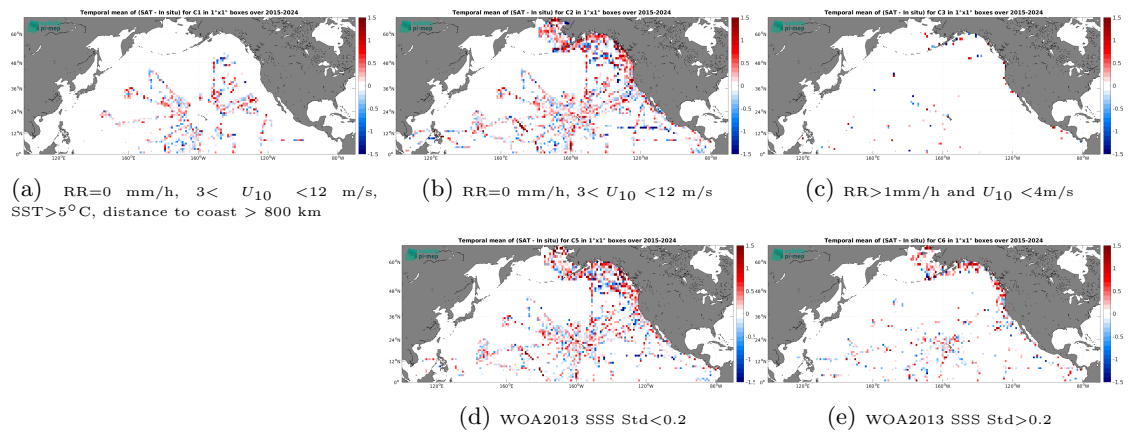
Figure 14: Temporal mean gridded over spatial boxes of size 1^\circ \times 1^\circ of \Delta SSS (SMAP SSS L2 v6 - 40 km (RSS) - TSG (SAMOS)) for 5 different subdatasets corresponding to:RR=0 mm/h, 3 < U_{10} < 12 m/s, SST > 5^\circ C , distance to coast > 800 km (a), RR=0 mm/h, 3 < U_{10} < 12 m/s (b), RR>1mm/h and U_{10} < 4 m/s (c), WOA2013 SSS Std<0.2 (d), WOA2013 SSS Std>0.2 (e).
