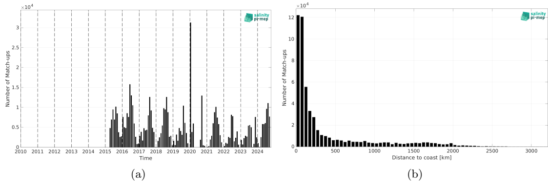
Figure 2: Number of match-ups between TSG (SAMOS) and SMAP SSS L2 v6 - 40 km (RSS) SSS as a function of time (a) and as function of the distance to coast (b) over the North Pacific Ocean Pi-MEP region and for the full satellite product period.
