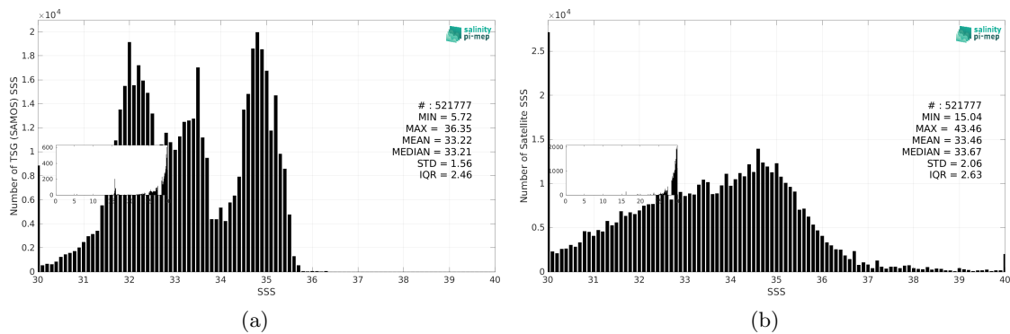
Figure 3: Histograms of SSS from TSG (SAMOS) (a) and SMAP SSS L2 v6 - 40 km (RSS) (b) considering all match-up pairs per bins of 0.1 over the North Pacific Ocean Pi-MEP region and for the full satellite product period.
