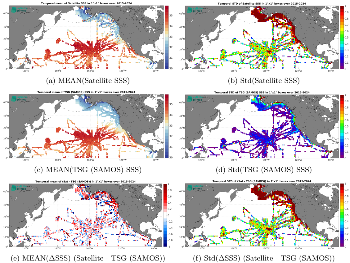
Figure 7: Temporal mean (left) and Std (right) of SSS from SMAP SSS L2 v6 - 40 km (RSS) (top), TSG (SAMOS) (middle), and of \Delta SSS (Satellite - TSG (SAMOS)). Only match-up pairs are used to generate these maps.
