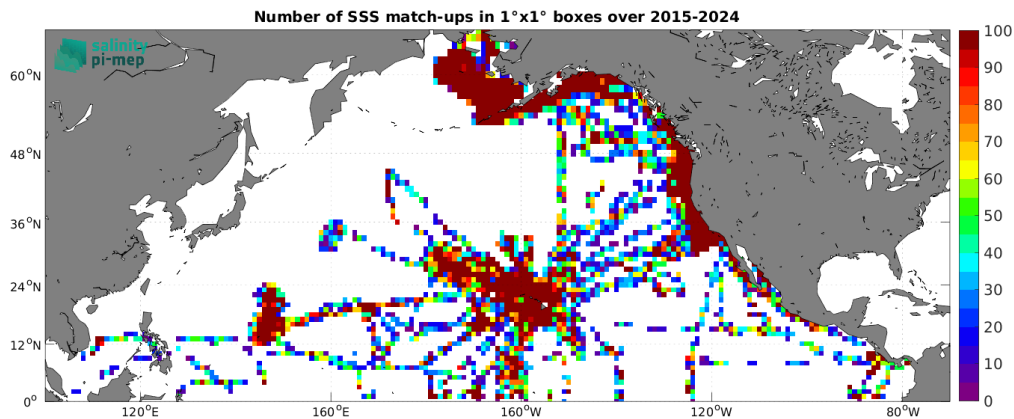
Figure 5: Number of SSS match-ups between TSG (SAMOS) SSS and the SMAP SSS L2 v6 - 40 km (RSS) SSS product for the North Pacific Ocean Pi-MEP region over 1^\circ \times 1^\circ boxes and for the full satellite product period.
