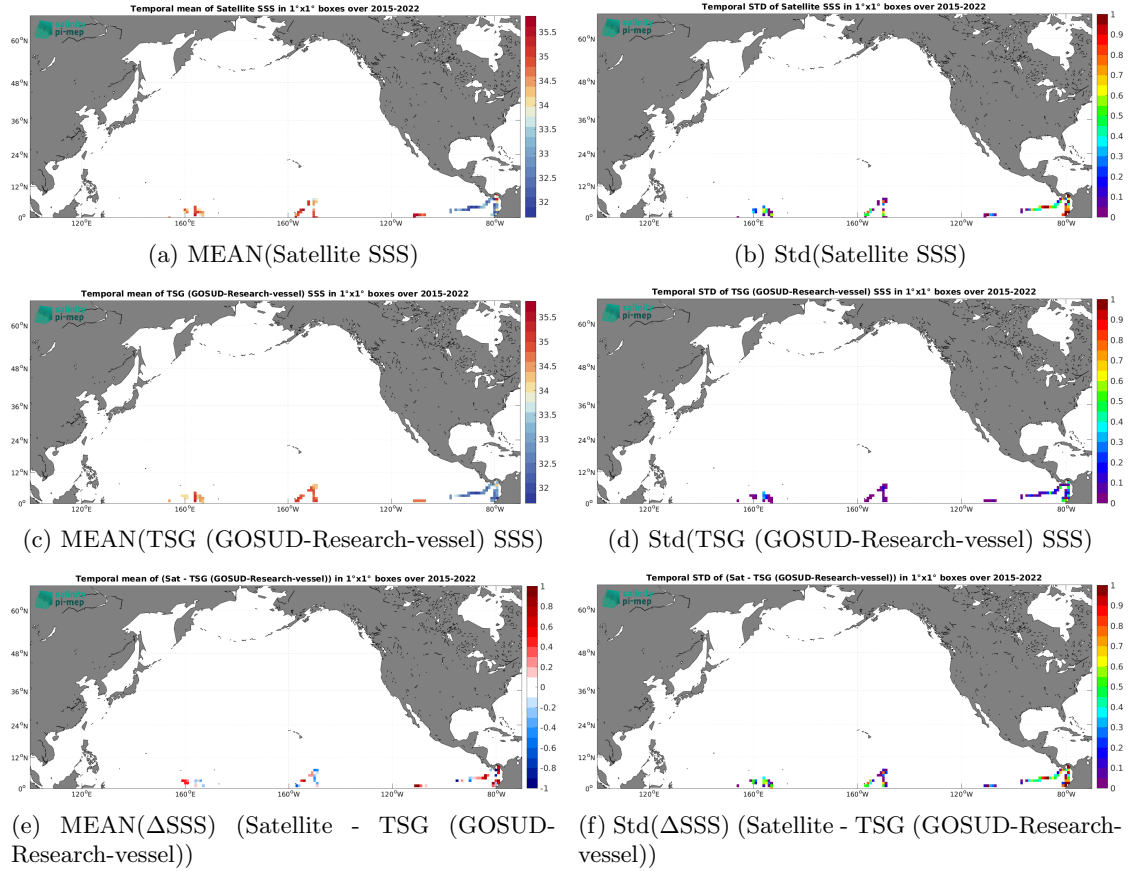
Figure 7: Temporal mean (left) and Std (right) of SSS from SMAP SSS L2 v6 - 40 km (RSS) (top), TSG (GOSUD-Research-vessel) (middle), and of \Delta SSS (Satellite - TSG (GOSUD-Research-vessel)). Only match-up pairs are used to generate these maps.
