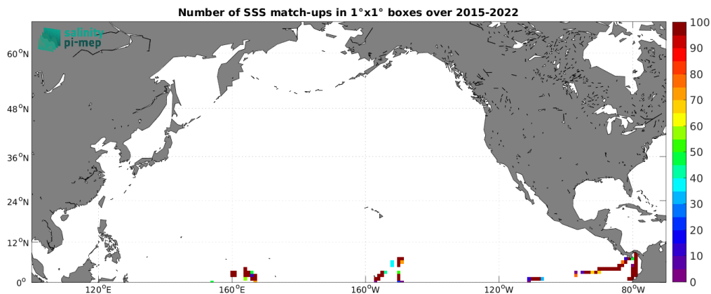
Figure 5: Number of SSS match-ups between TSG (GOSUD-Research-vessel) SSS and the SMAP SSS L2 v6 - 40 km (RSS) SSS product for the North Pacific Ocean Pi-MEP region over 1^\circ \times 1^\circ boxes and for the full satellite product period.
