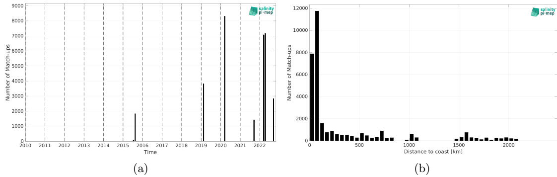
Figure 2: Number of match-ups between TSG (GOSUD-Research-vessel) and SMAP SSS L2 v6 - 40 km (RSS) SSS as a function of time (a) and as function of the distance to coast (b) over the North Pacific Ocean Pi-MEP region and for the full satellite product period.
