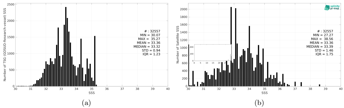
Figure 3: Histograms of SSS from TSG (GOSUD-Research-vessel) (a) and SMAP SSS L2 v6 - 40 km (RSS) (b) considering all match-up pairs per bins of 0.1 over the North Pacific Ocean Pi-MEP region and for the full satellite product period.
