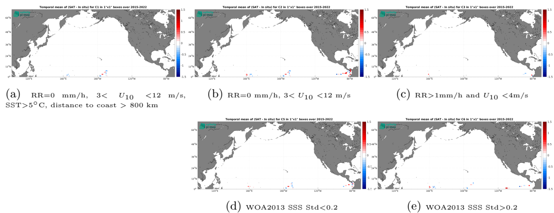
Figure 14: Temporal mean gridded over spatial boxes of size 1^\circ \times 1^\circ of \Delta SSS (SMAP SSS L2 v6 - 40 km (RSS) - TSG (GOSUD-Research-vessel)) for 5 different subdatasets corresponding to:RR=0 mm/h, 3 < U_{10} < 12 m/s, SST >5^\circ C, distance to coast > 800 km (a), RR=0 mm/h, 3 < U_{10} < 12 m/s (b), RR >1 mm/h and U_{10} < 4 m/s (c), WOA2013 SSS Std <0.2 (d), WOA2013 SSS Std >0.2 (e).
