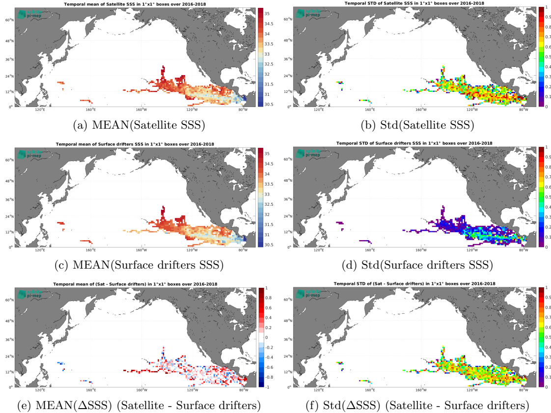
Figure 6: Temporal mean (left) and Std (right) of SSS from SMAP SSS L2 v6 - 40 km (RSS) (top), Surface drifters (middle), and of \Delta SSS (Satellite - Surface drifters). Only match-up pairs are used to generate these maps.
