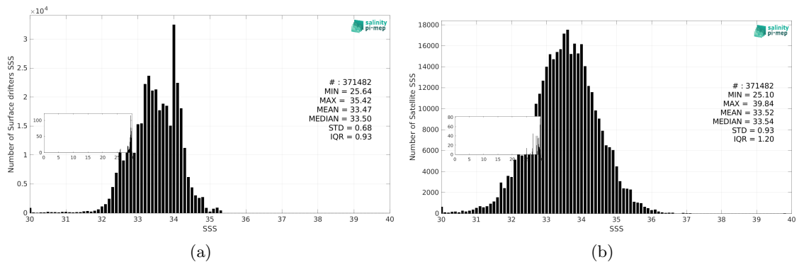
Figure 3: Histograms of SSS from Surface drifters (a) and SMAP SSS L2 v6 - 40 km (RSS) (b) considering all match-up pairs per bins of 0.1 over the North Pacific Ocean Pi-MEP region and for the full satellite product period.
