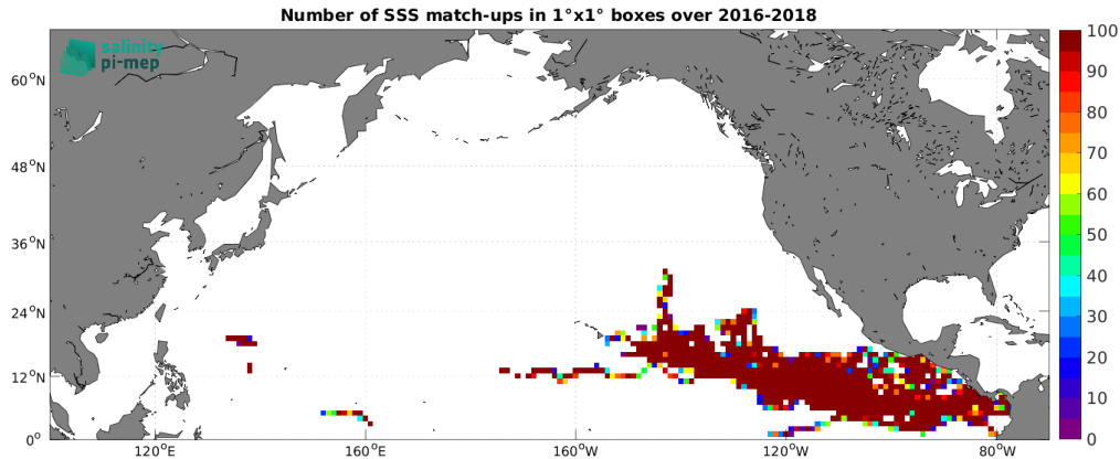
Figure 4: Number of SSS match-ups between Surface drifters SSS and the SMAP SSS L2 v6 - 40 km (RSS) SSS product for the North Pacific Ocean Pi-MEP region over 1^\circ \times 1^\circ boxes and for the full satellite product period.
