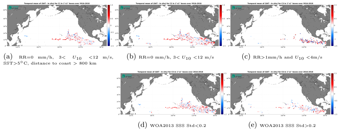
Figure 13: Temporal mean gridded over spatial boxes of size 1^\circ \times 1^\circ of \Delta SSS (SMAP SSS L2 v6 - 40 km (RSS) - Surface drifters) for 5 different subdatasets corresponding to:RR=0 mm/h, 3 < U_{10} < 12 m/s, SST >5^\circ\text{C} , distance to coast > 800 km (a), RR=0 mm/h, 3 < U_{10} < 12 m/s (b), RR >1 mm/h and U_{10} < 4 m/s (c), WOA2013 SSS Std <0.2 (d), WOA2013 SSS Std >0.2 (e).
