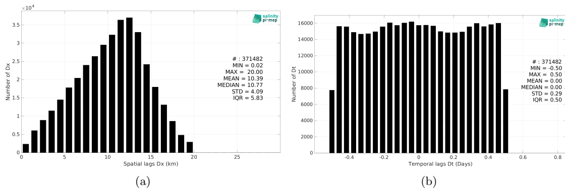
Figure 5: Histograms of the spatial (a) and temporal (b) lags between the location/time of the Surface drifters measurement and the date of the corresponding SMAP SSS L2 v6 - 40 km (RSS) SSS pixel.
