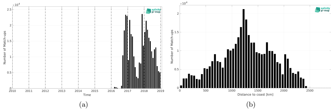
Figure 2: Number of match-ups between Surface drifters and SMAP SSS L2 v6 - 40 km (RSS) SSS as a function of time (a) and as function of the distance to coast (b) over the North Pacific Ocean Pi-MEP region and for the full satellite product period.
