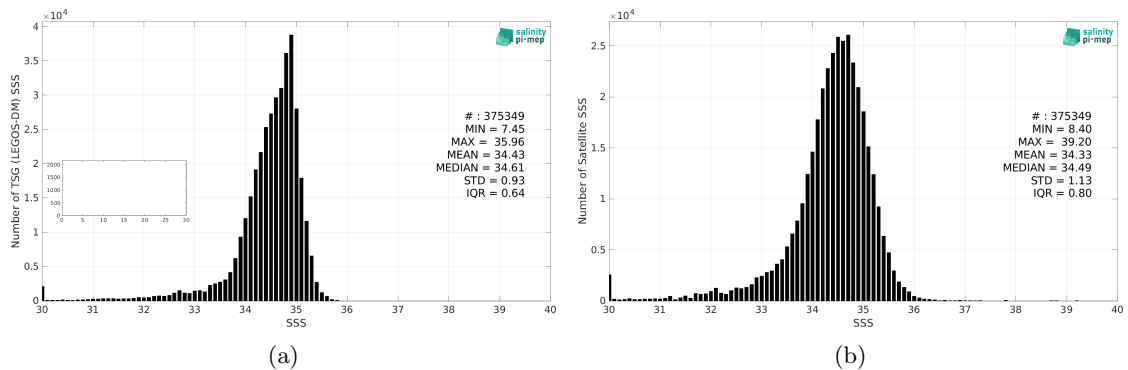
Figure 2: Histograms of SSS from TSG (LEGOS-DM) (a) and SMAP SSS L2 v5 (RSS) (b) considering all match-up pairs per bins of 0.1 over the North Pacific Ocean Pi-MEP region and for the full satellite product period.
