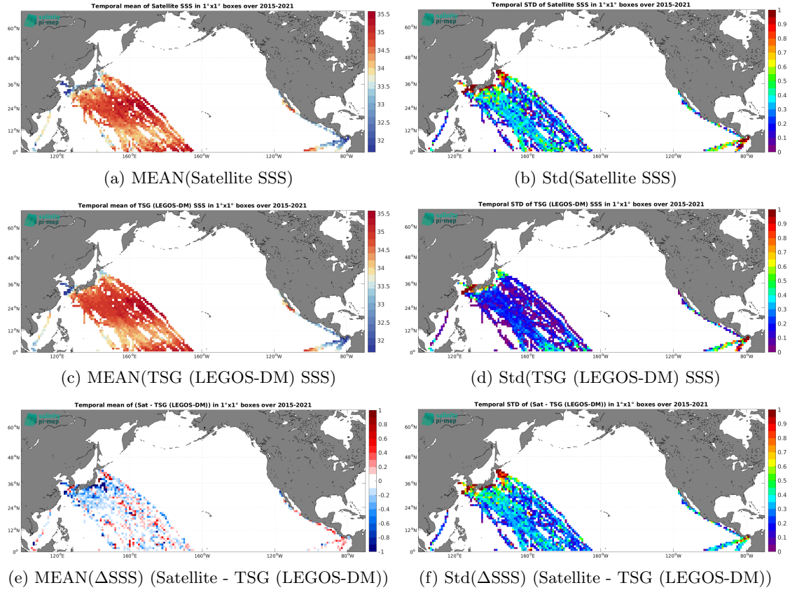
Figure 6: Temporal mean (left) and Std (right) of SSS from SMAP SSS L2 v5 (RSS) (top), TSG (LEGOS-DM) (middle), and of \Delta SSS (Satellite - TSG (LEGOS-DM)). Only match-up pairs are used to generate these maps.
