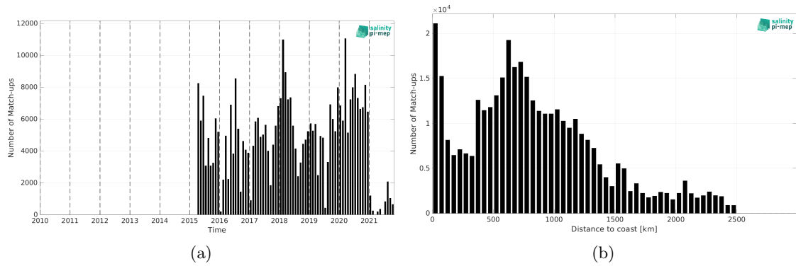
Figure 1: Number of match-ups between TSG (LEGOS-DM) and SMAP SSS L2 v5 (RSS) SSS as a function of time (a) and as function of the distance to coast (b) over the North Pacific Ocean Pi-MEP region and for the full satellite product period.
