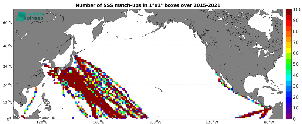
Figure 4: Number of SSS match-ups between TSG (LEGOS-DM) SSS and the SMAP SSS L2 v5 (RSS) SSS product for the North Pacific Ocean Pi-MEP region over 1^\circ \times 1^\circ boxes and for the full satellite product period.
