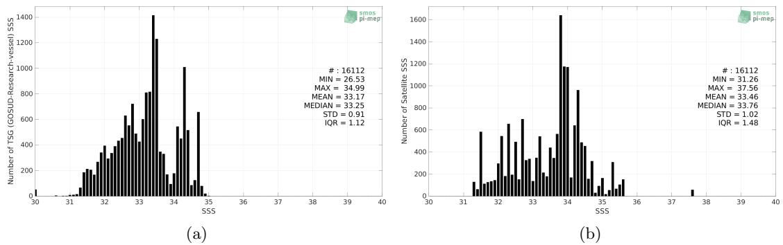
Figure 2: Histograms of SSS from TSG (GOSUD-Research-vessel) (a) and SMAP SSS L2 v5 (RSS) (b) considering all match-up pairs per bins of 0.1 over the North Pacific Ocean Pi-MEP region and for the full satellite product period.
