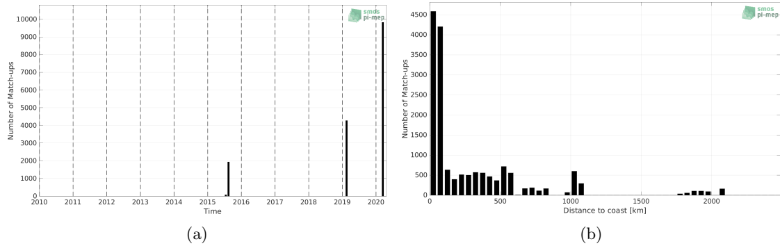
Figure 1: Number of match-ups between TSG (GOSUD-Research-vessel) and SMAP SSS L2 v5 (RSS) SSS as a function of time (a) and as function of the distance to coast (b) over the North Pacific Ocean Pi-MEP region and for the full satellite product period.
