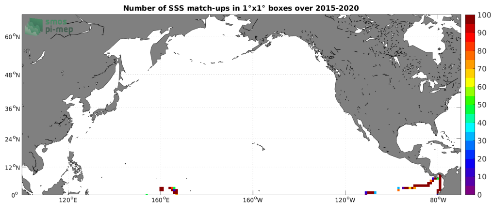
Figure 4: Number of SSS match-ups between TSG (GOSUD-Research-vessel) SSS and the SMAP SSS L2 v5 (RSS) SSS product for the North Pacific Ocean Pi-MEP region over 1^\circ \times 1^\circ boxes and for the full satellite product period.
