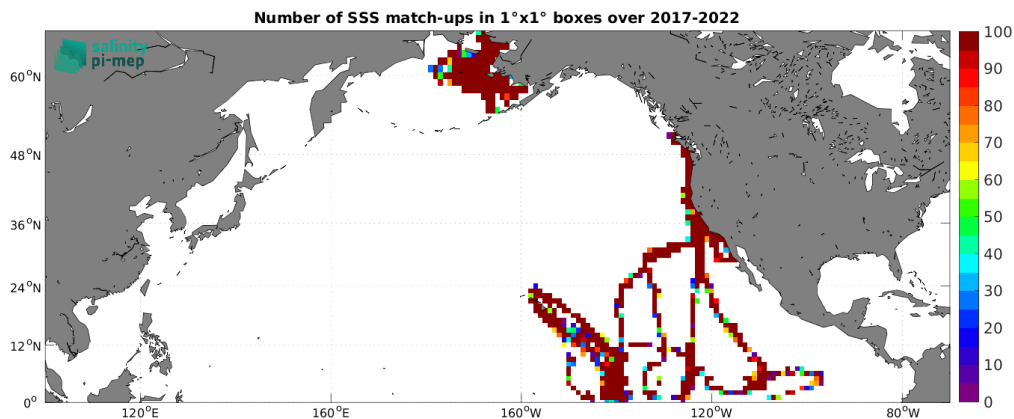
Figure 4: Number of SSS match-ups between Saildrone SSS and the SMAP SSS L2 v5 (RSS) SSS product for the North Pacific Ocean Pi-MEP region over 1^\circ \times 1^\circ boxes and for the full satellite product period.
