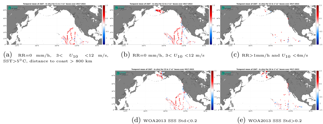
Figure 12: Temporal mean gridded over spatial boxes of size 1^\circ \times 1^\circ of \Delta SSS (SMAP SSS L2 v5 (RSS) - Saildrone) for 5 different subdatasets corresponding to:RR=0 mm/h, 3 < U_{10} < 12 m/s, SST >5^\circ\text{C} , distance to coast > 800 km (a), RR=0 mm/h, 3 < U_{10} < 12 m/s (b), RR >1 mm/h and U_{10} < 4 m/s (c), WOA2013 SSS Std <0.2 (d), WOA2013 SSS Std >0.2 (e).
