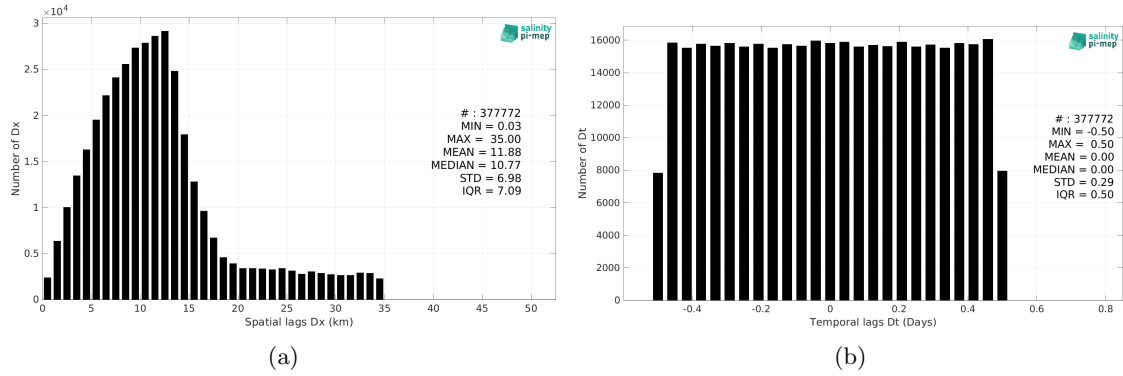
Figure 5: Histograms of the spatial (a) and temporal (b) lags between the location/time of the Saildrone measurement and the date of the corresponding SMAP SSS L2 v5 (RSS) SSS pixel.
