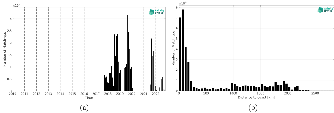
Figure 1: Number of match-ups between Saildrone and SMAP SSS L2 v5 (RSS) SSS as a function of time (a) and as function of the distance to coast (b) over the North Pacific Ocean Pi-MEP region and for the full satellite product period.
