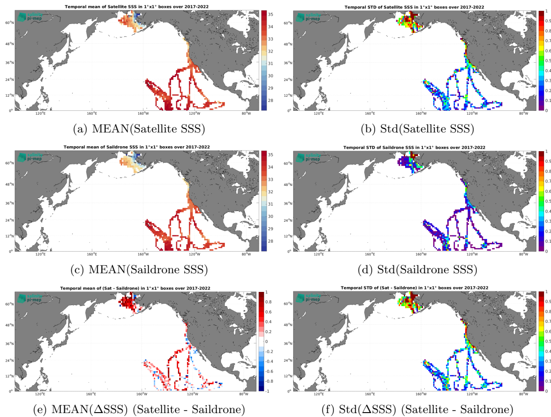
Figure 6: Temporal mean (left) and Std (right) of SSS from SMAP SSS L2 v5 (RSS) (top), Saildrone (middle), and of \Delta SSS (Satellite - Saildrone). Only match-up pairs are used to generate these maps.
