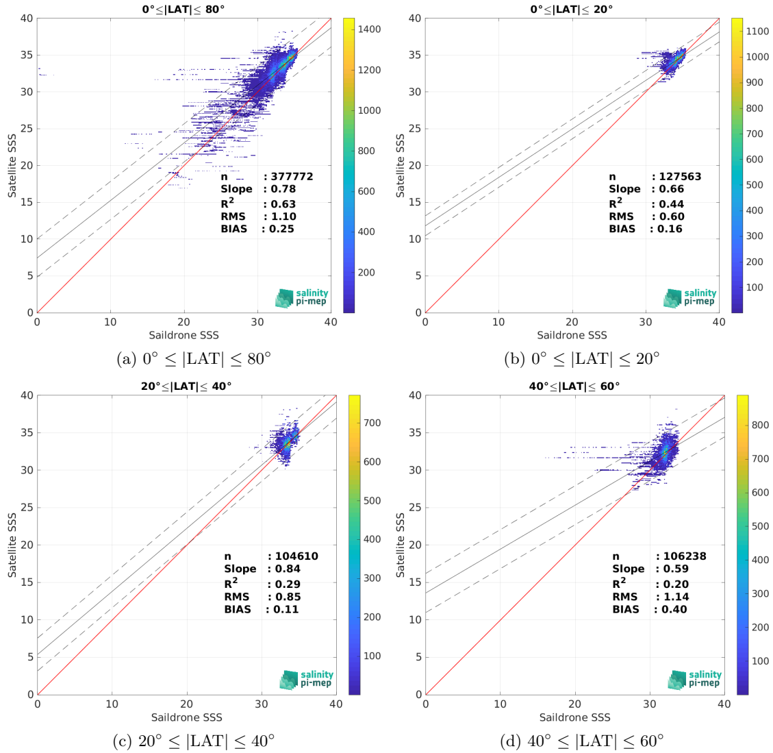
Figure 9: Contour maps of the concentration of SMAP SSS L2 v5 (RSS) SSS (y-axis) versus Saildrone SSS (x-axis) at match-up pairs for different latitude bands. For each plot, the red line shows x=y . The black thin and dashed lines indicate a linear fit through the data cloud and the \pm 95\% confidence levels, respectively. The number match-up pairs n , the slope and R^2 coefficient of the linear fit, the root mean square (RMS) and the mean bias between satellite and in situ data are indicated for each latitude band in each plots.
