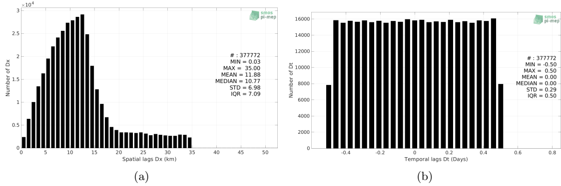
Figure 5: Histograms of the spatial (a) and temporal (b) lags between the location/time of the Sairdrone measurement and the date of the corresponding SMAP SSS L2 v5 (RSS) SSS pixel.
