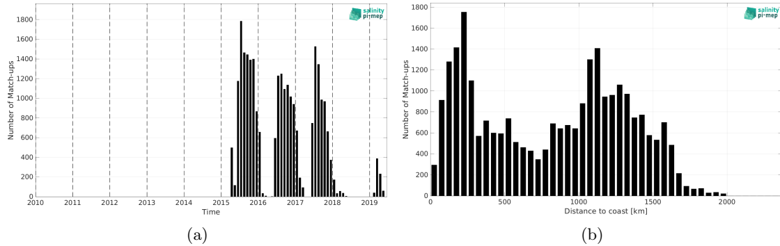
Figure 1: Number of match-ups between Marine mammals and SMAP SSS L2 v5 (RSS) SSS as a function of time (a) and as function of the distance to coast (b) over the North Pacific Ocean Pi-MEP region and for the full satellite product period.
