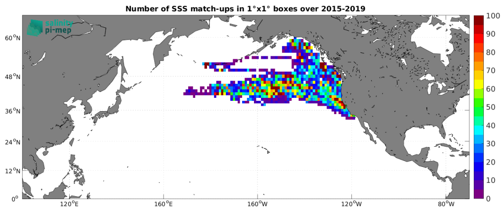
Figure 4: Number of SSS match-ups between Marine mammals SSS and the SMAP SSS L2 v5 (RSS) SSS product for the North Pacific Ocean Pi-MEP region over 1^\circ \times 1^\circ boxes and for the full satellite product period.
