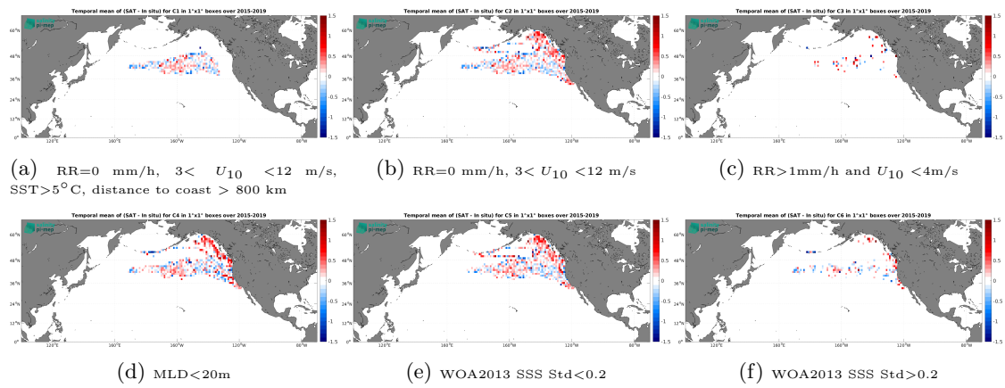
Figure 12: Temporal mean gridded over spatial boxes of size 1^\circ \times 1^\circ of \Delta SSS (SMAP SSS L2 v5 (RSS) - Marine mammals) for 6 different subdatasets corresponding to:RR=0 mm/h, 3 < U_{10} < 12 m/s, SST >5^\circ C, distance to coast > 800 km (a), RR=0 mm/h, 3 < U_{10} < 12 m/s (b), RR >1 mm/h and U_{10} < 4 m/s (c),MLD <20 m (d),WOA2013 SSS Std <0.2 (e),WOA2013 SSS Std >0.2 (f).
