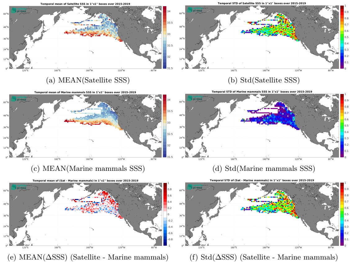
Figure 6: Temporal mean (left) and Std (right) of SSS from SMAP SSS L2 v5 (RSS) (top), Marine mammals (middle), and of \Delta SSS (Satellite - Marine mammals). Only match-up pairs are used to generate these maps.
