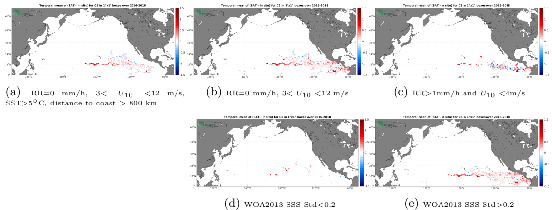
Figure 11: Temporal mean gridded over spatial boxes of size 1^\circ \times 1^\circ of \Delta SSS (SMAP SSS L2 v5 (RSS) - Surface drifters) for 5 different subdatasets corresponding to:RR=0 mm/h, 3 < U_{10} < 12 m/s, SST >5^\circ\text{C} , distance to coast > 800 km (a), RR=0 mm/h, 3 < U_{10} < 12 m/s (b), RR >1 mm/h and U_{10} < 4 m/s (c), WOA2013 SSS Std <0.2 (d), WOA2013 SSS Std >0.2 (e).
