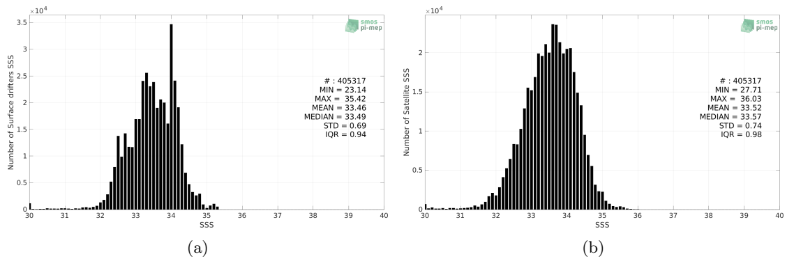
Figure 2: Histograms of SSS from Surface drifters (a) and SMAP SSS L2 v5 (RSS) (b) considering all match-up pairs per bins of 0.1 over the North Pacific Ocean Pi-MEP region and for the full satellite product period.
