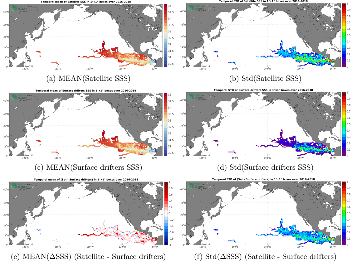
Figure 5: Temporal mean (left) and Std (right) of SSS from SMAP SSS L2 v5 (RSS) (top), Surface drifters (middle), and of \Delta SSS (Satellite - Surface drifters). Only match-up pairs are used to generate these maps.
