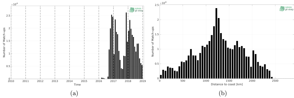
Figure 1: Number of match-ups between Surface drifters and SMAP SSS L2 v5 (RSS) SSS as a function of time (a) and as function of the distance to coast (b) over the North Pacific Ocean Pi-MEP region and for the full satellite product period.
