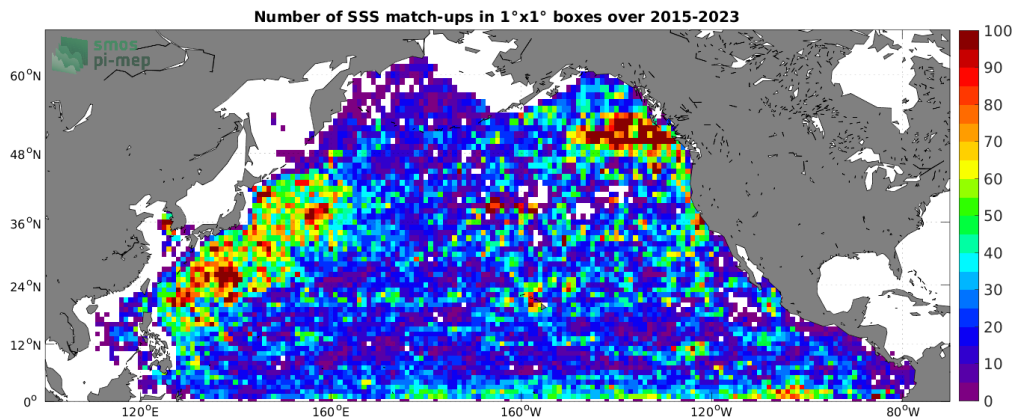
Figure 4: Number of SSS match-ups between Argo SSS and the SMAP SSS L2 v5 (RSS) SSS product for the North Pacific Ocean Pi-MEP region over 1^\circ \times 1^\circ boxes and for the full satellite product period.
