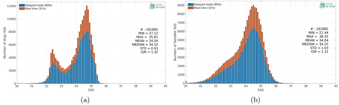
Figure 2: Histograms of SSS from Argo (a) and SMAP SSS L2 v5 (RSS) (b) considering all match-up pairs per bins of 0.1 over the North Pacific Ocean Pi-MEP region and for the full satellite product period.
