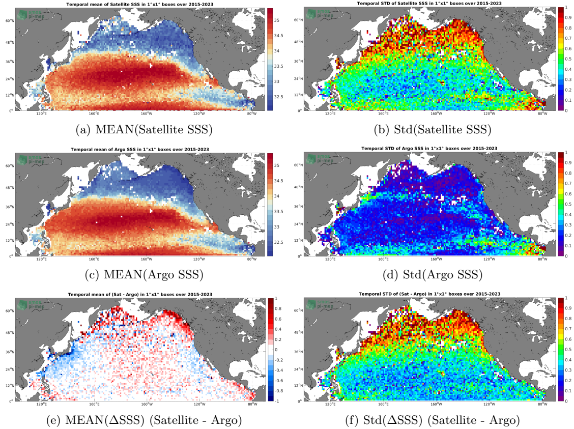
Figure 6: Temporal mean (left) and Std (right) of SSS from SMAP SSS L2 v5 (RSS) (top), Argo (middle), and of \Delta SSS (Satellite - Argo). Only match-up pairs are used to generate these maps.
