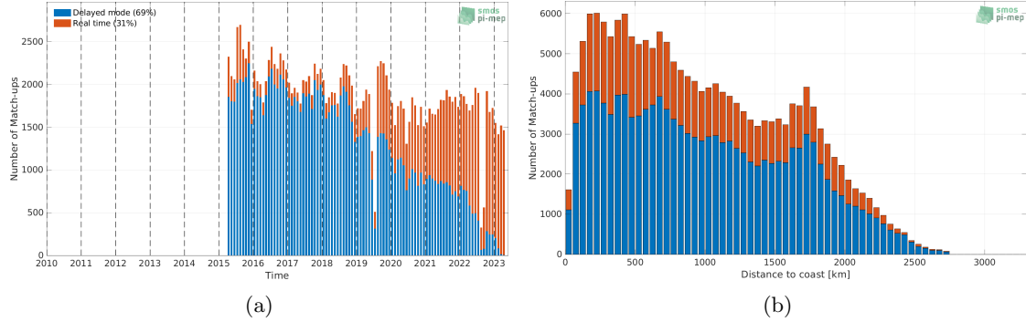
Figure 1: Number of match-ups between Argo and SMAP SSS L2 v5 (RSS) SSS as a function of time (a) and as function of the distance to coast (b) over the North Pacific Ocean Pi-MEP region and for the full satellite product period.
