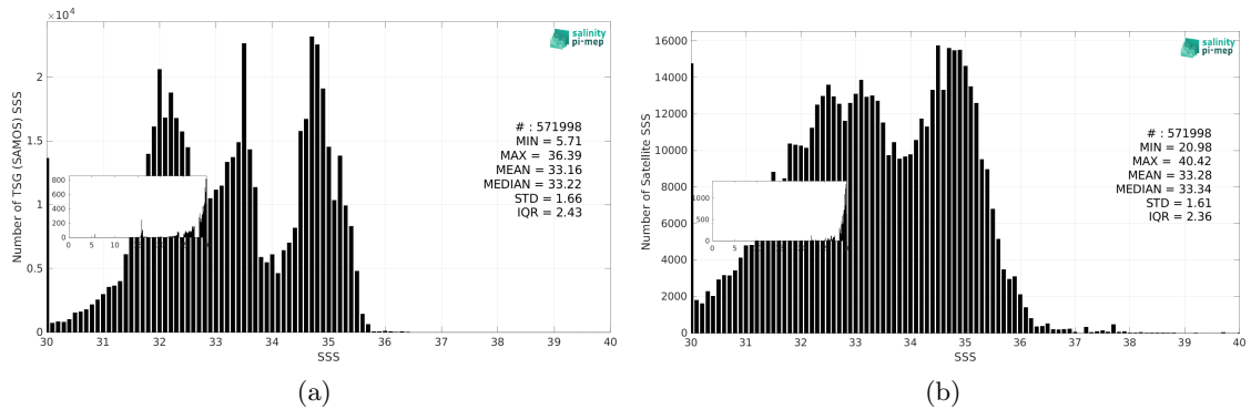
Figure 3: Histograms of SSS from TSG (SAMOS) (a) and SMAP SSS L2 v5.3 (RSS) (b) considering all match-up pairs per bins of 0.1 over the North Pacific Ocean Pi-MEP region and for the full satellite product period.
