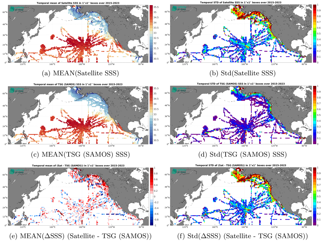
Figure 7: Temporal mean (left) and Std (right) of SSS from SMAP SSS L2 v5.3 (RSS) (top), TSG (SAMOS) (middle), and of \Delta SSS (Satellite - TSG (SAMOS)). Only match-up pairs are used to generate these maps.
