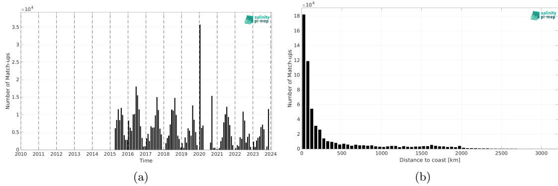
Figure 2: Number of match-ups between TSG (SAMOS) and SMAP SSS L2 v5.3 (RSS) SSS as a function of time (a) and as function of the distance to coast (b) over the North Pacific Ocean Pi-MEP region and for the full satellite product period.
