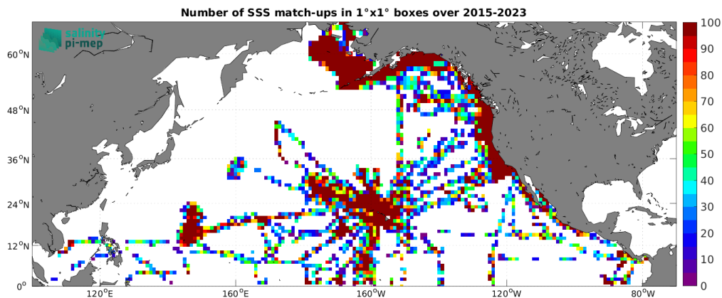
Figure 5: Number of SSS match-ups between TSG (SAMOS) SSS and the SMAP SSS L2 v5.3 (RSS) SSS product for the North Pacific Ocean Pi-MEP region over 1^\circ \times 1^\circ boxes and for the full satellite product period.
