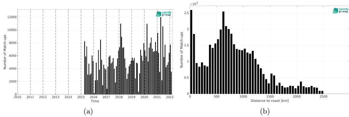
Figure 2: Number of match-ups between TSG (LEGOS-DM) and SMAP SSS L2 v5.3 (RSS) SSS as a function of time (a) and as function of the distance to coast (b) over the North Pacific Ocean Pi-MEP region and for the full satellite product period.
