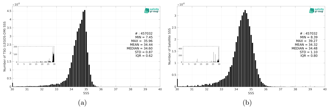
Figure 3: Histograms of SSS from TSG (LEGOS-DM) (a) and SMAP SSS L2 v5.3 (RSS) (b) considering all match-up pairs per bins of 0.1 over the North Pacific Ocean Pi-MEP region and for the full satellite product period.
