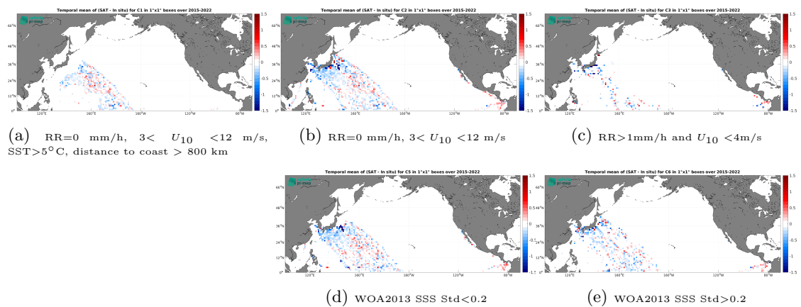
Figure 14: Temporal mean gridded over spatial boxes of size 1^\circ \times 1^\circ of \Delta SSS (SMAP SSS L2 v5.3 (RSS) - TSG (LEGOS-DM)) for 5 different subdatasets corresponding to:RR=0 mm/h, 3 < U_{10} < 12 m/s, SST > 5^\circ C , distance to coast > 800 km (a), RR=0 mm/h, 3 < U_{10} < 12 m/s (b), RR>1mm/h and U_{10} < 4 m/s (c), WOA2013 SSS Std<0.2 (d), WOA2013 SSS Std>0.2 (e).
