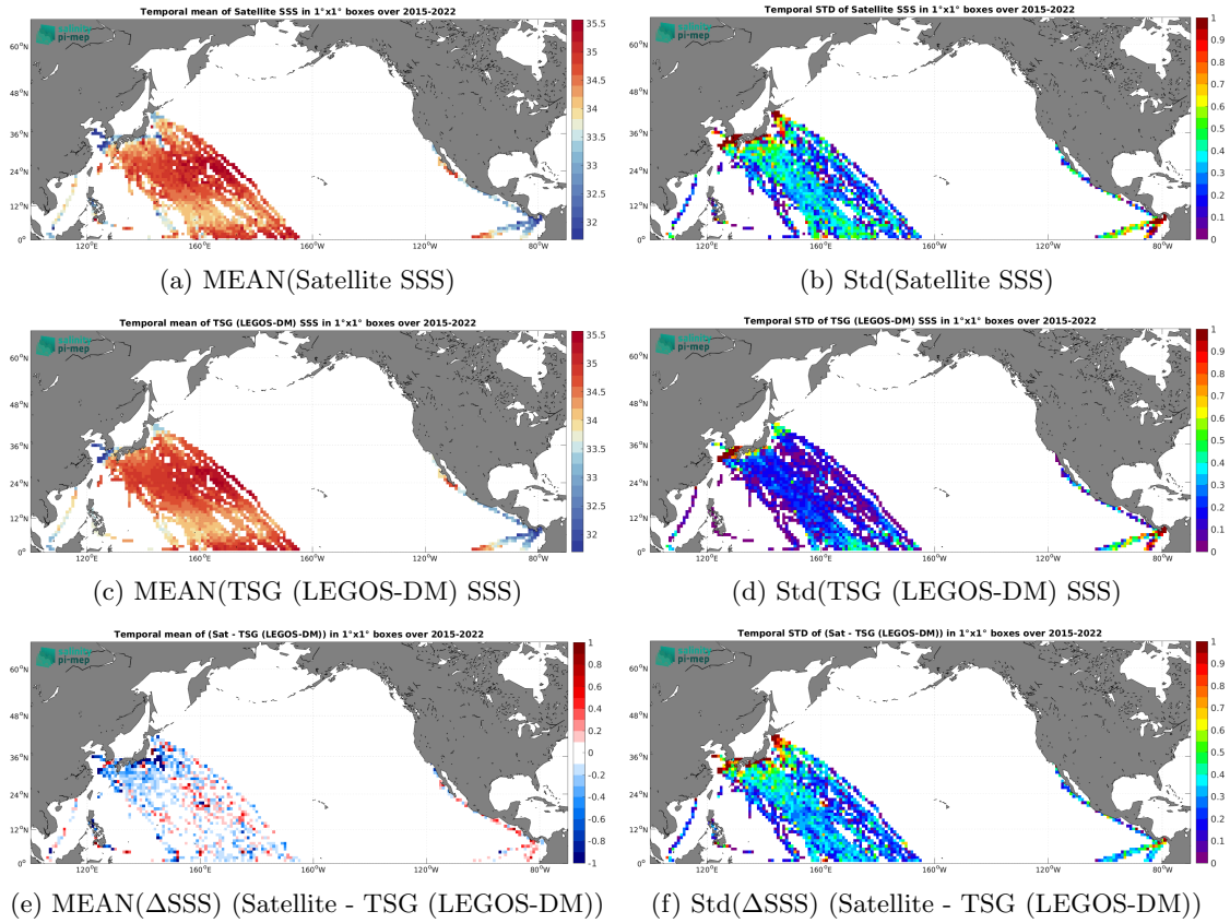
Figure 7: Temporal mean (left) and Std (right) of SSS from SMAP SSS L2 v5.3 (RSS) (top), TSG (LEGOS-DM) (middle), and of \Delta SSS (Satellite - TSG (LEGOS-DM)). Only match-up pairs are used to generate these maps.
