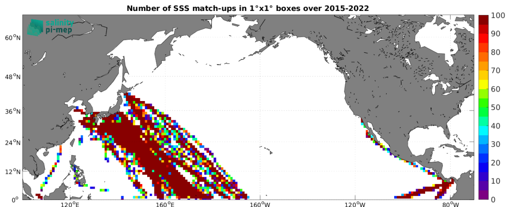
Figure 5: Number of SSS match-ups between TSG (LEGOS-DM) SSS and the SMAP SSS L2 v5.3 (RSS) SSS product for the North Pacific Ocean Pi-MEP region over 1^\circ \times 1^\circ boxes and for the full satellite product period.
