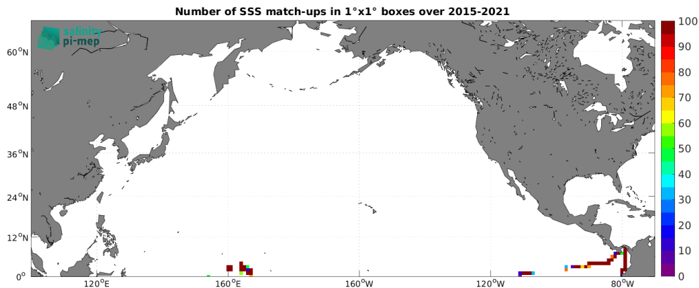
Figure 5: Number of SSS match-ups between TSG (GOSUD-Research-vessel) SSS and the SMAP SSS L2 v5.3 (RSS) SSS product for the North Pacific Ocean Pi-MEP region over 1^\circ \times 1^\circ boxes and for the full satellite product period.
