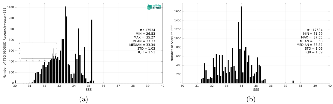
Figure 3: Histograms of SSS from TSG (GOSUD-Research-vessel) (a) and SMAP SSS L2 v5.3 (RSS) (b) considering all match-up pairs per bins of 0.1 over the North Pacific Ocean Pi-MEP region and for the full satellite product period.
