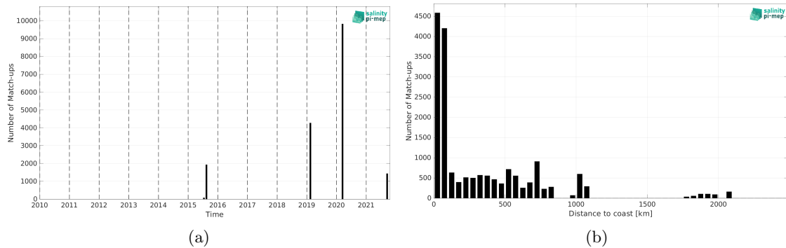
Figure 2: Number of match-ups between TSG (GOSUD-Research-vessel) and SMAP SSS L2 v5.3 (RSS) SSS as a function of time (a) and as function of the distance to coast (b) over the North Pacific Ocean Pi-MEP region and for the full satellite product period.
