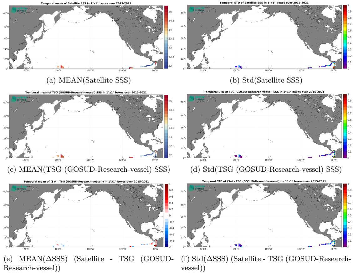
Figure 7: Temporal mean (left) and Std (right) of SSS from SMAP SSS L2 v5.3 (RSS) (top), TSG (GOSUD-Research-vessel) (middle), and of \Delta SSS (Satellite - TSG (GOSUD-Research-vessel)). Only match-up pairs are used to generate these maps.
