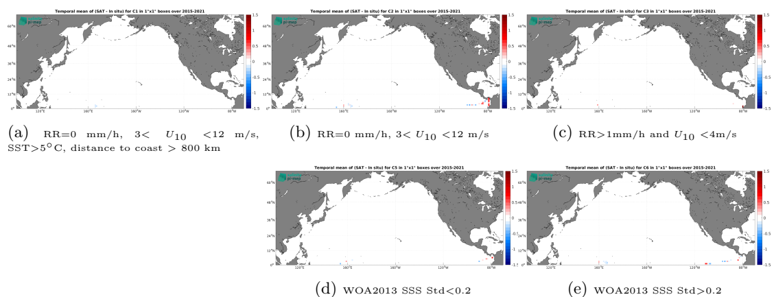
Figure 14: Temporal mean gridded over spatial boxes of size 1^\circ \times 1^\circ of \Delta\text{SSS} (SMAP SSS L2 v5.3 (RSS) - TSG (GOSUD-Research-vessel)) for 5 different subdatasets corresponding to: RR=0 mm/h, 3 < U_{10} < 12 m/s, SST > 5°C, distance to coast > 800 km (a), RR=0 mm/h, 3 < U_{10} < 12 m/s (b), RR > 1mm/h and U_{10} < 4 m/s (c), WOA2013 SSS Std < 0.2 (d), WOA2013 SSS Std > 0.2 (e).
