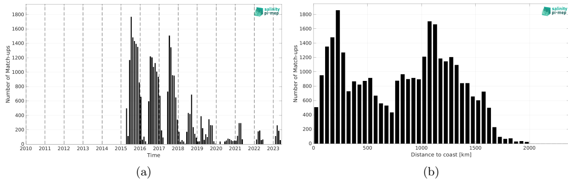
Figure 2: Number of match-ups between Marine mammals and SMAP SSS L2 v5.3 (RSS) SSS as a function of time (a) and as function of the distance to coast (b) over the North Pacific Ocean Pi-MEP region and for the full satellite product period.
