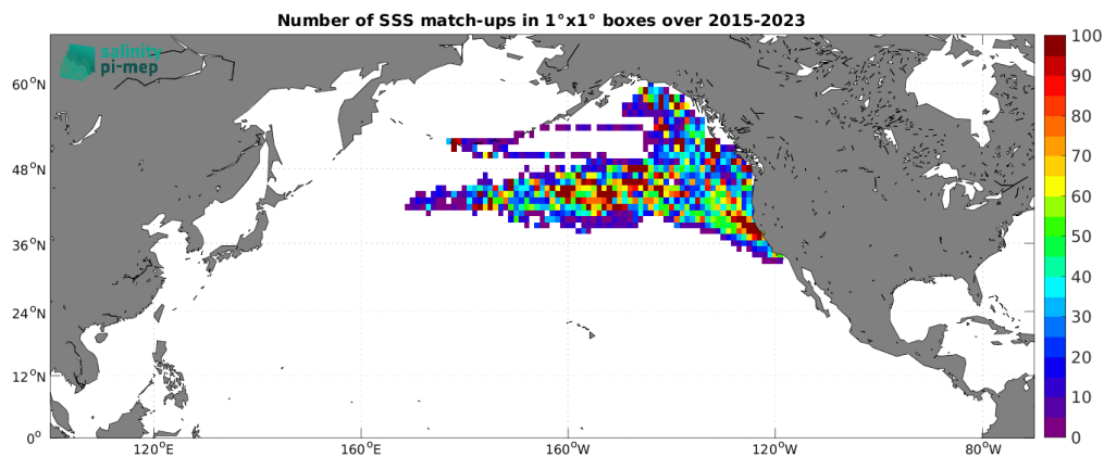
Figure 5: Number of SSS match-ups between Marine mammals SSS and the SMAP SSS L2 v5.3 (RSS) SSS product for the North Pacific Ocean Pi-MEP region over 1^\circ \times 1^\circ boxes and for the full satellite product period.
