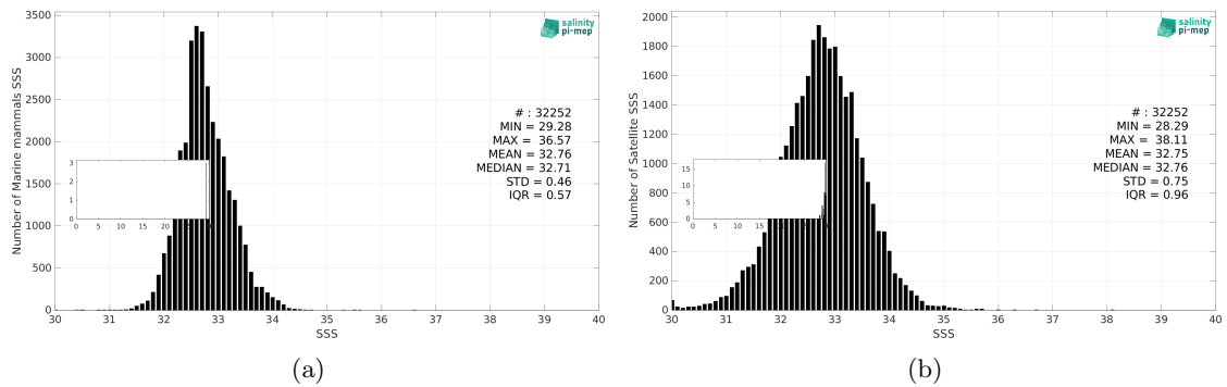
Figure 3: Histograms of SSS from Marine mammals (a) and SMAP SSS L2 v5.3 (RSS) (b) considering all match-up pairs per bins of 0.1 over the North Pacific Ocean Pi-MEP region and for the full satellite product period.
