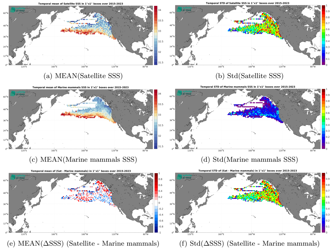
Figure 7: Temporal mean (left) and Std (right) of SSS from SMAP SSS L2 v5.3 (RSS) (top), Marine mammals (middle), and of \Delta SSS (Satellite - Marine mammals). Only match-up pairs are used to generate these maps.
