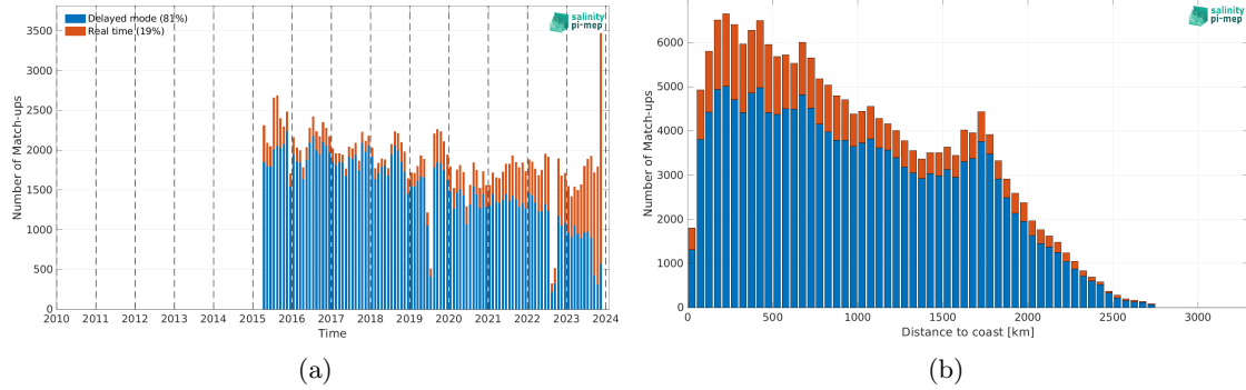
Figure 2: Number of match-ups between Argo and SMAP SSS L2 v5.3 (RSS) SSS as a function of time (a) and as function of the distance to coast (b) over the North Pacific Ocean Pi-MEP region and for the full satellite product period.
