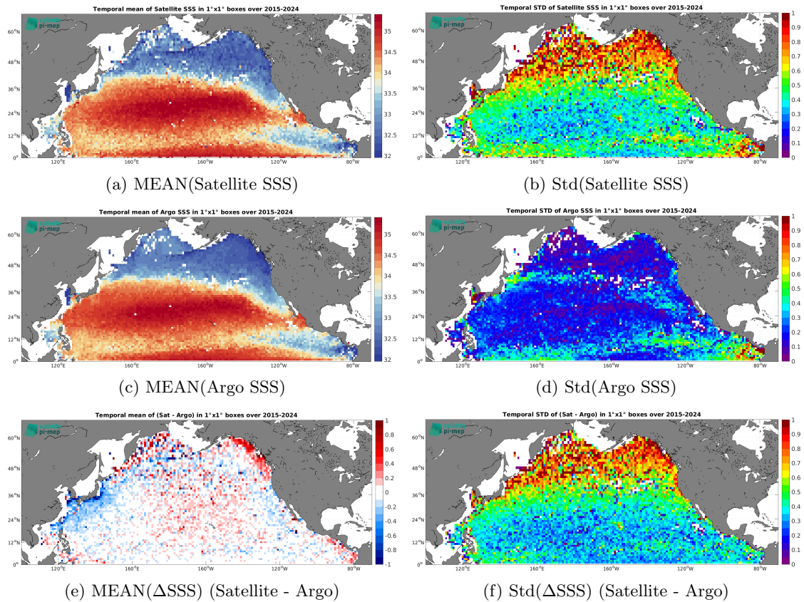
Figure 7: Temporal mean (left) and Std (right) of SSS from SMAP SSS L2 v5.3 (RSS) (top), Argo (middle), and of \Delta SSS (Satellite - Argo). Only match-up pairs are used to generate these maps.
