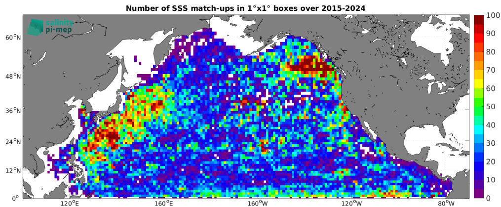
Figure 5: Number of SSS match-ups between Argo SSS and the SMAP SSS L2 v5.3 (RSS) SSS product for the North Pacific Ocean Pi-MEP region over 1^\circ \times 1^\circ boxes and for the full satellite product period.
