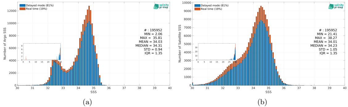
Figure 3: Histograms of SSS from Argo (a) and SMAP SSS L2 v5.3 (RSS) (b) considering all match-up pairs per bins of 0.1 over the North Pacific Ocean Pi-MEP region and for the full satellite product period.
