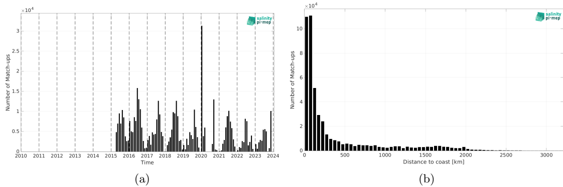
Figure 2: Number of match-ups between TSG (SAMOS) and SMAP SSS L2 v5.3 - 40 km (RSS) SSS as a function of time (a) and as function of the distance to coast (b) over the North Pacific Ocean Pi-MEP region and for the full satellite product period.
