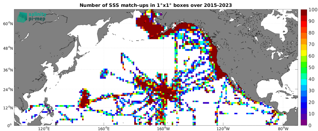
Figure 5: Number of SSS match-ups between TSG (SAMOS) SSS and the SMAP SSS L2 v5.3 - 40 km (RSS) SSS product for the North Pacific Ocean Pi-MEP region over 1^\circ \times 1^\circ boxes and for the full satellite product period.
