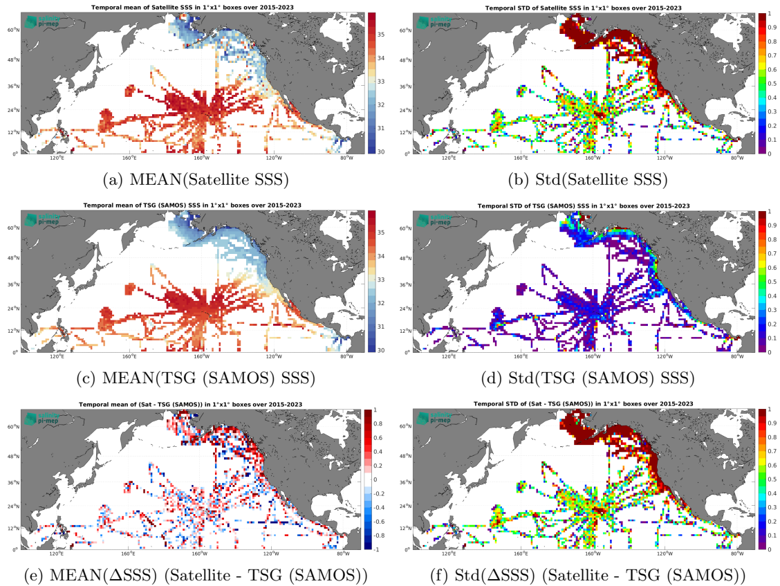
Figure 7: Temporal mean (left) and Std (right) of SSS from SMAP SSS L2 v5.3 - 40 km (RSS) (top), TSG (SAMOS) (middle), and of \Delta SSS (Satellite - TSG (SAMOS)). Only match-up pairs are used to generate these maps.
