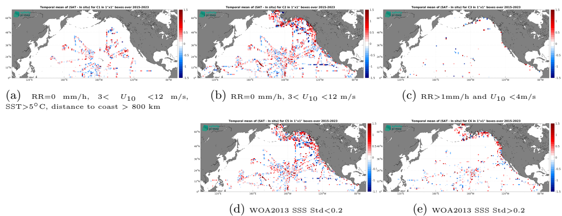
Figure 14: Temporal mean gridded over spatial boxes of size 1^\circ \times 1^\circ of \Delta SSS (SMAP SSS L2 v5.3 - 40 km (RSS) - TSG (SAMOS)) for 5 different subdatasets corresponding to:RR=0 mm/h, 3 < U_{10} < 12 m/s, SST>5°C, distance to coast > 800 km (a), RR=0 mm/h, 3 < U_{10} < 12 m/s (b), RR>1mm/h and U_{10} < 4 m/s (c), WOA2013 SSS Std<0.2 (d), WOA2013 SSS Std>0.2 (e).
