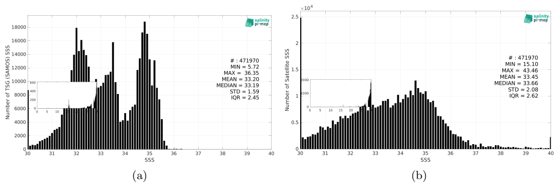
Figure 3: Histograms of SSS from TSG (SAMOS) (a) and SMAP SSS L2 v5.3 - 40 km (RSS) (b) considering all match-up pairs per bins of 0.1 over the North Pacific Ocean Pi-MEP region and for the full satellite product period.
