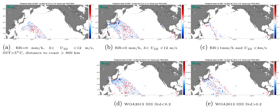
Figure 14: Temporal mean gridded over spatial boxes of size 1^\circ \times 1^\circ of \Delta\text{SSS} (SMAP SSS L2 v5.3 - 40 km (RSS) - TSG (LEGOS-DM)) for 5 different subdatasets corresponding to:RR=0 mm/h, 3 < U_{10} < 12 m/s, SST > 5°C, distance to coast > 800 km (a), RR=0 mm/h, 3 < U_{10} < 12 m/s (b), RR > 1mm/h and U_{10} < 4 m/s (c), WOA2013 SSS Std < 0.2 (d), WOA2013 SSS Std > 0.2 (e).
