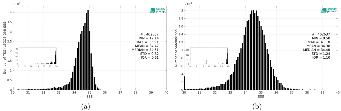
Figure 3: Histograms of SSS from TSG (LEGOS-DM) (a) and SMAP SSS L2 v5.3 - 40 km (RSS) (b) considering all match-up pairs per bins of 0.1 over the North Pacific Ocean Pi-MEP region and for the full satellite product period.
