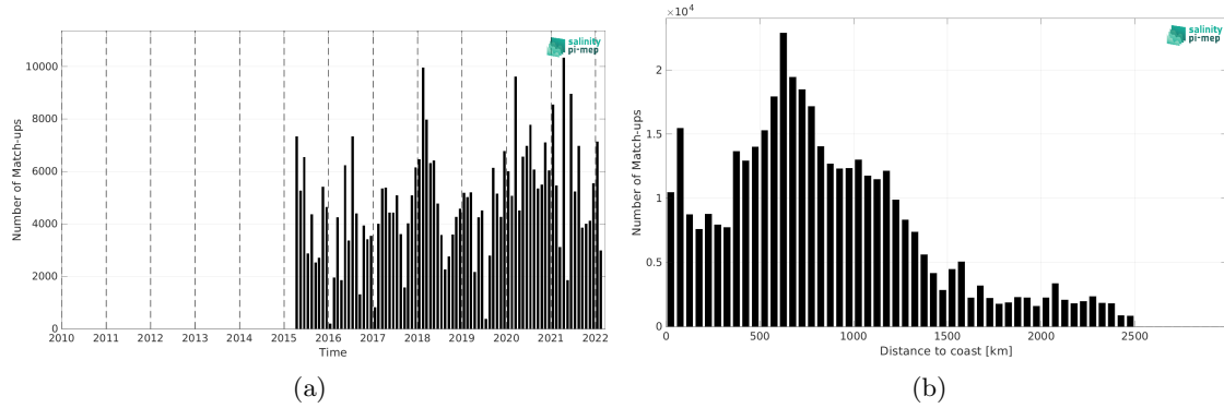
Figure 2: Number of match-ups between TSG (LEGOS-DM) and SMAP SSS L2 v5.3 - 40 km (RSS) SSS as a function of time (a) and as function of the distance to coast (b) over the North Pacific Ocean Pi-MEP region and for the full satellite product period.
