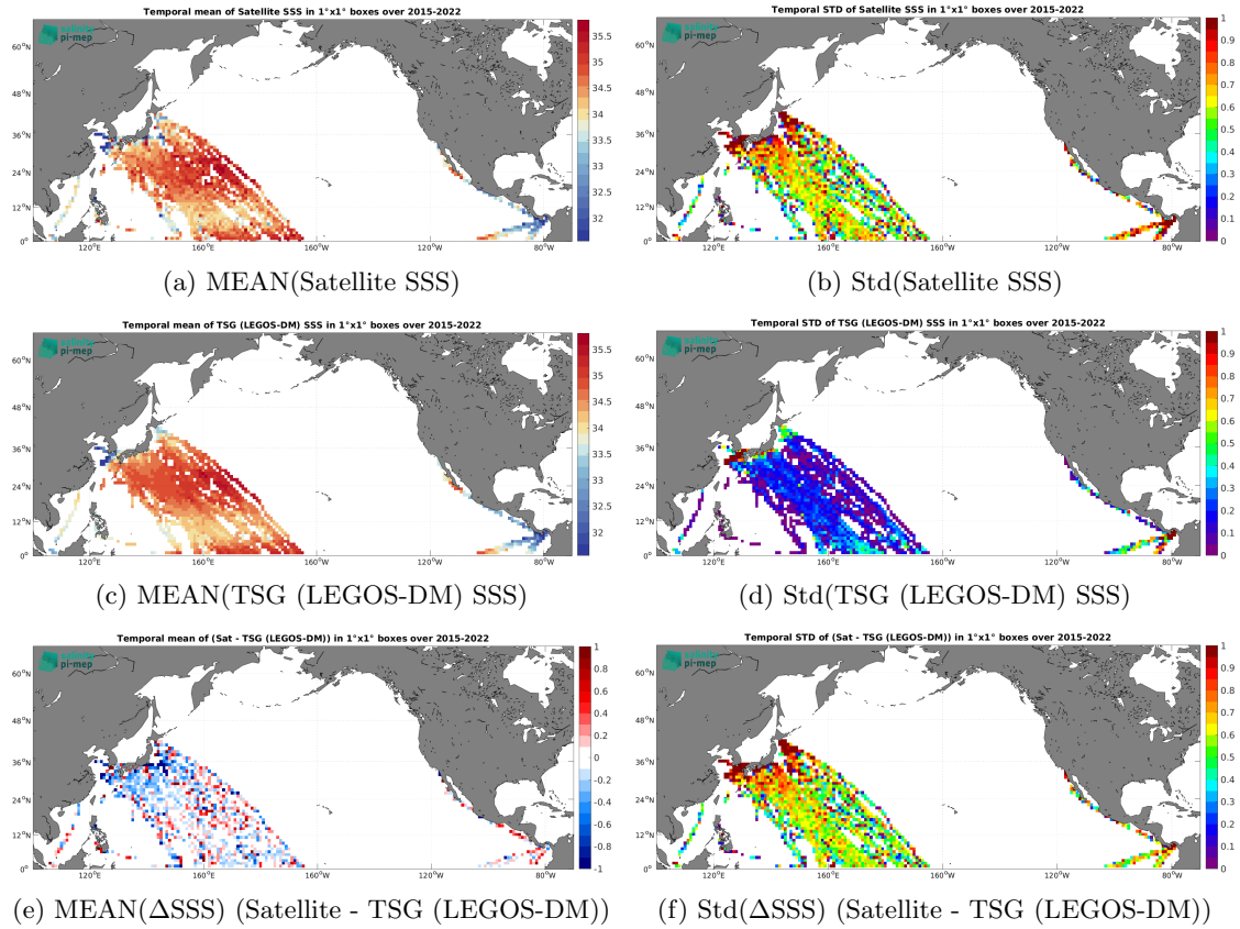
Figure 7: Temporal mean (left) and Std (right) of SSS from SMAP SSS L2 v5.3 - 40 km (RSS) (top), TSG (LEGOS-DM) (middle), and of \Delta SSS (Satellite - TSG (LEGOS-DM)). Only match-up pairs are used to generate these maps.
