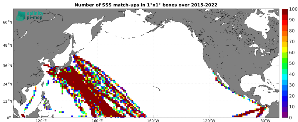
Figure 5: Number of SSS match-ups between TSG (LEGOS-DM) SSS and the SMAP SSS L2 v5.3 - 40 km (RSS) SSS product for the North Pacific Ocean Pi-MEP region over 1^\circ \times 1^\circ boxes and for the full satellite product period.
