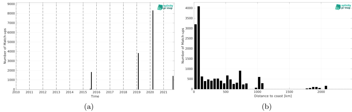
Figure 2: Number of match-ups between TSG (GOSUD-Research-vessel) and SMAP SSS L2 v5.3 - 40 km (RSS) SSS as a function of time (a) and as function of the distance to coast (b) over the North Pacific Ocean Pi-MEP region and for the full satellite product period.
