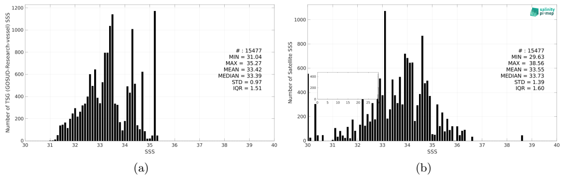
Figure 3: Histograms of SSS from TSG (GOSUD-Research-vessel) (a) and SMAP SSS L2 v5.3 - 40 km (RSS) (b) considering all match-up pairs per bins of 0.1 over the North Pacific Ocean Pi-MEP region and for the full satellite product period.
