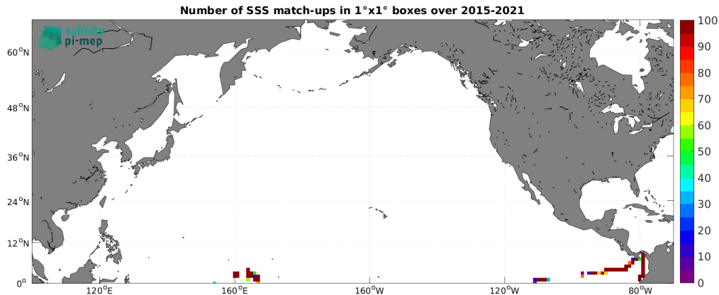
Figure 5: Number of SSS match-ups between TSG (GOSUD-Research-vessel) SSS and the SMAP SSS L2 v5.3 - 40 km (RSS) SSS product for the North Pacific Ocean Pi-MEP region over 1^\circ \times 1^\circ boxes and for the full satellite product period.
