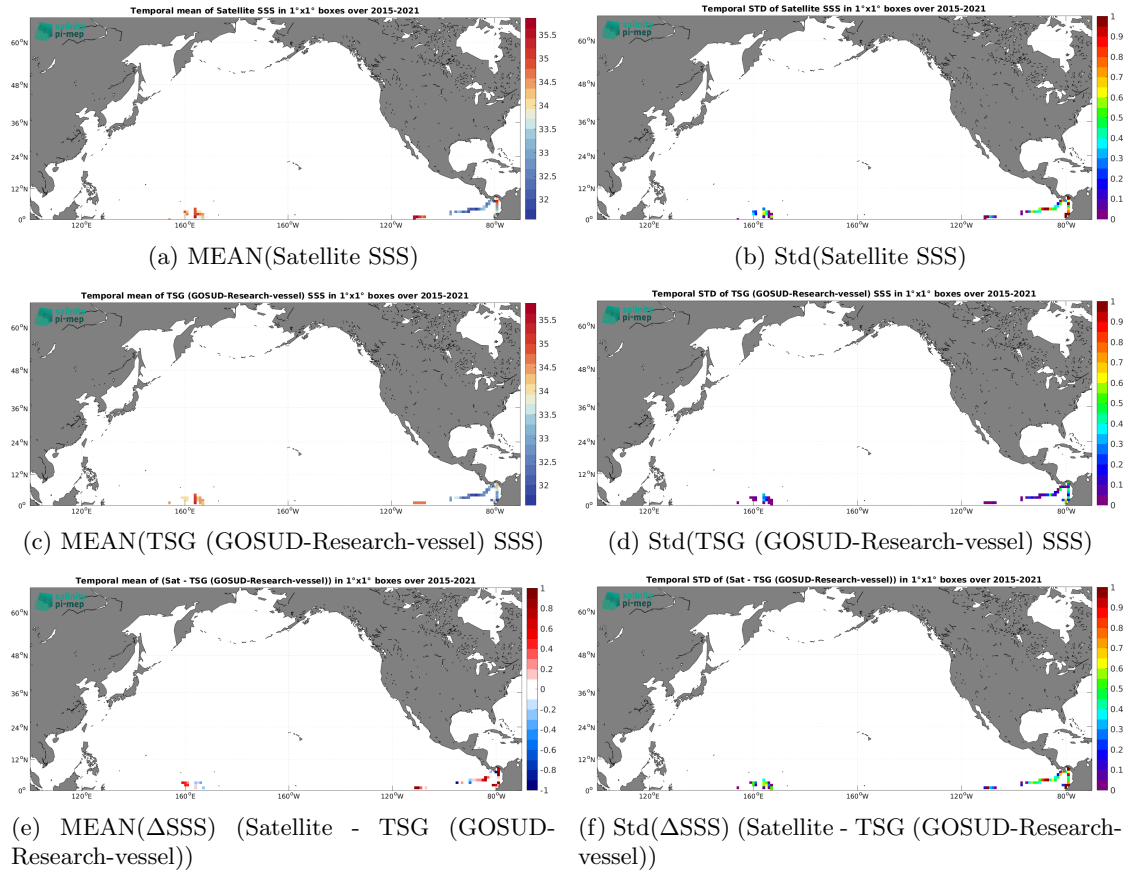
Figure 7: Temporal mean (left) and Std (right) of SSS from SMAP SSS L2 v5.3 - 40 km (RSS) (top), TSG (GOSUD-Research-vessel) (middle), and of \Delta SSS (Satellite - TSG (GOSUD-Research-vessel)). Only match-up pairs are used to generate these maps.
