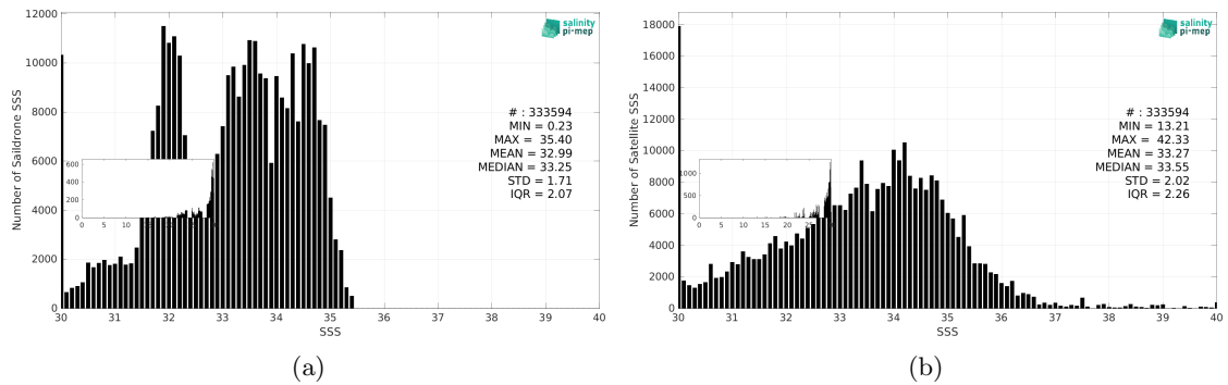
Figure 3: Histograms of SSS from Sailldrone (a) and SMAP SSS L2 v5.3 - 40 km (RSS) (b) considering all match-up pairs per bins of 0.1 over the North Pacific Ocean Pi-MEP region and for the full satellite product period.
