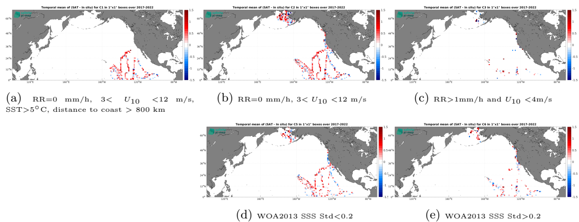
Figure 14: Temporal mean gridded over spatial boxes of size 1^\circ \times 1^\circ of \Delta SSS (SMAP SSS L2 v5.3 - 40 km (RSS) - Saildrone) for 5 different subdatasets corresponding to:RR=0 mm/h, 3 < U_{10} < 12 m/s, SST >5^\circ\text{C} , distance to coast > 800 km (a), RR=0 mm/h, 3 < U_{10} < 12 m/s (b), RR >1 mm/h and U_{10} < 4 m/s (c), WOA2013 SSS Std <0.2 (d), WOA2013 SSS Std >0.2 (e).
