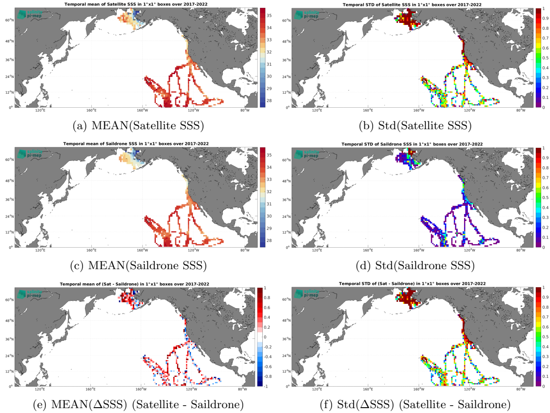
Figure 7: Temporal mean (left) and Std (right) of SSS from SMAP SSS L2 v5.3 - 40 km (RSS) (top), Saildrone (middle), and of \Delta SSS (Satellite - Saildrone). Only match-up pairs are used to generate these maps.
