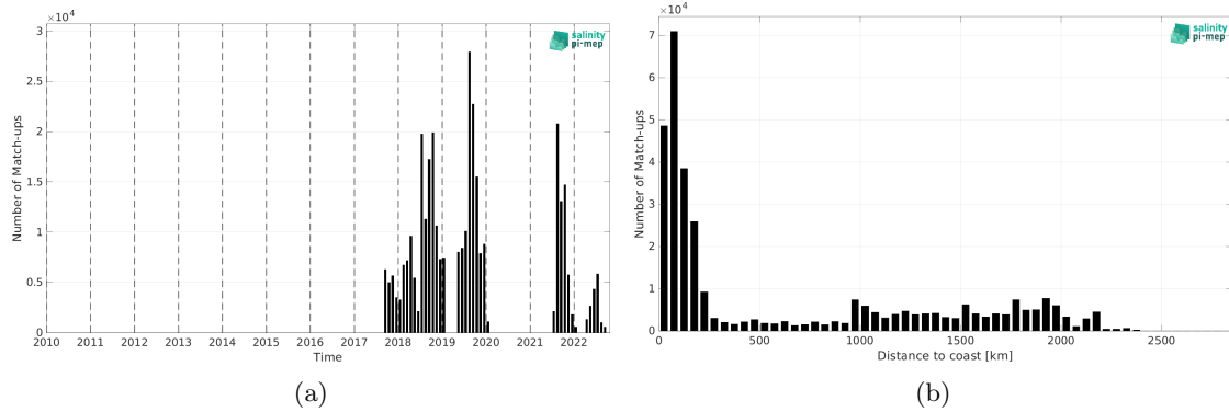
Figure 2: Number of match-ups between Sailldrone and SMAP SSS L2 v5.3 - 40 km (RSS) SSS as a function of time (a) and as function of the distance to coast (b) over the North Pacific Ocean Pi-MEP region and for the full satellite product period.
