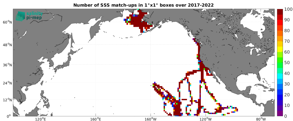
Figure 5: Number of SSS match-ups between Saildrone SSS and the SMAP SSS L2 v5.3 - 40 km (RSS) SSS product for the North Pacific Ocean Pi-MEP region over 1^\circ \times 1^\circ boxes and for the full satellite product period.
