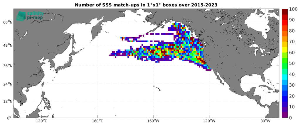
Figure 5: Number of SSS match-ups between Marine mammals SSS and the SMAP SSS L2 v5.3 - 40 km (RSS) SSS product for the North Pacific Ocean Pi-MEP region over 1^\circ \times 1^\circ boxes and for the full satellite product period.
