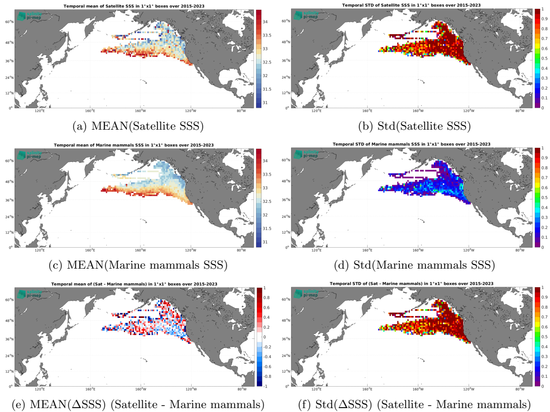
Figure 7: Temporal mean (left) and Std (right) of SSS from SMAP SSS L2 v5.3 - 40 km (RSS) (top), Marine mammals in situ dataset (middle), and of \Delta SSS (Satellite - Marine mammals). Only match-up pairs are used to generate these maps.
