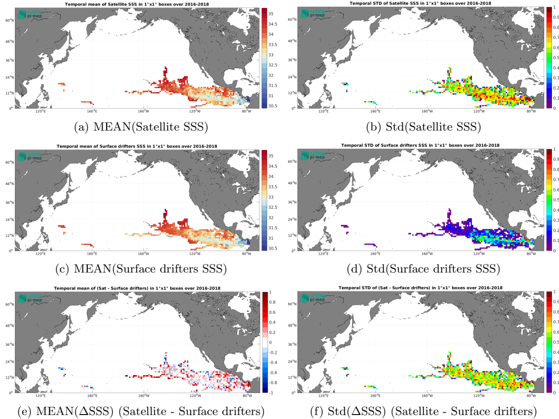
Figure 6: Temporal mean (left) and Std (right) of SSS from SMAP SSS L2 v5.3 - 40 km (RSS) (top), Surface drifters (middle), and of \Delta SSS (Satellite - Surface drifters). Only match-up pairs are used to generate these maps.
