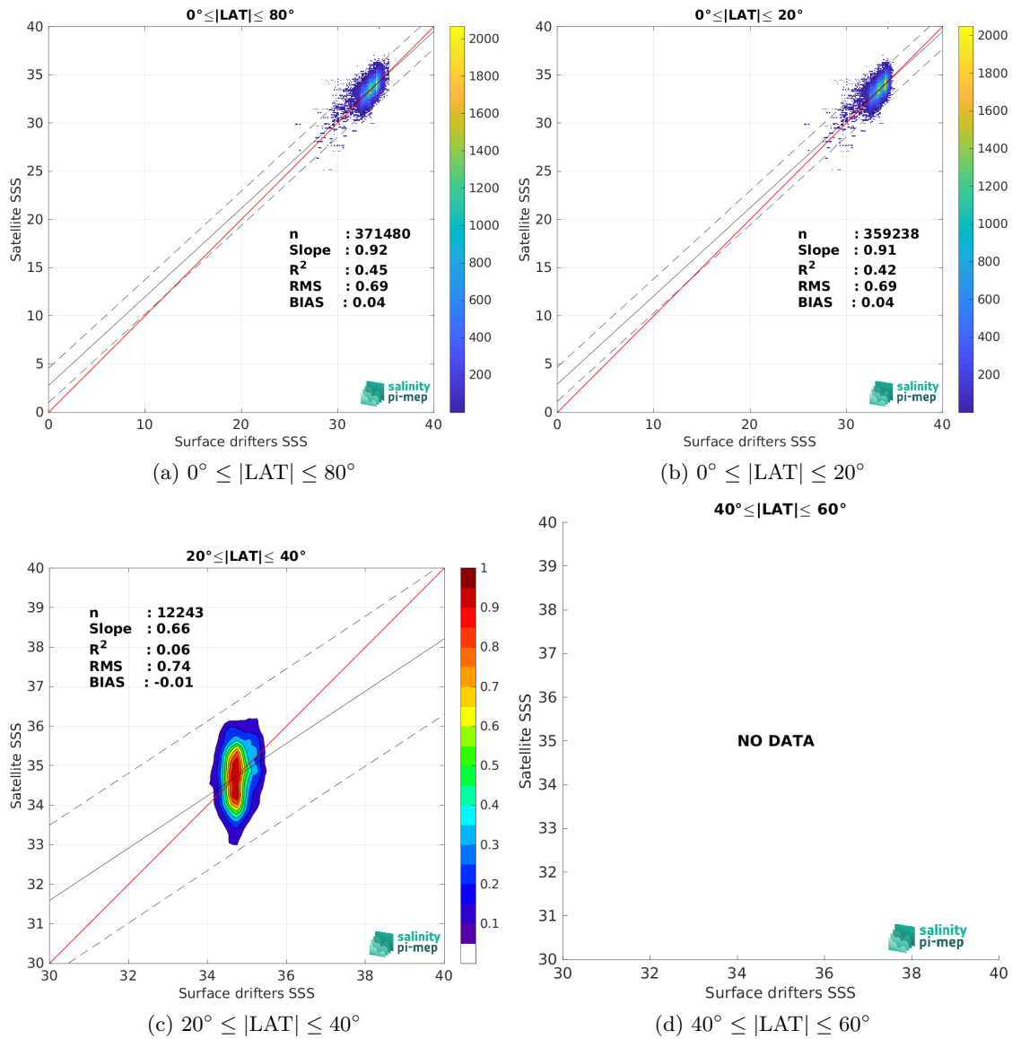
Figure 9: Contour maps of the concentration of SMAP SSS L2 v5.3 - 40 km (RSS) SSS (y-axis) versus Surface drifters SSS (x-axis) at match-up pairs for different latitude bands. For each plot, the red line shows x=y . The black thin and dashed lines indicate a linear fit through the data cloud and the \pm 95\% confidence levels, respectively. The number match-up pairs n , the slope and R^2 coefficient of the linear fit, the root mean square (RMS) and the mean bias between satellite and in situ data are indicated for each latitude band in each plots.
