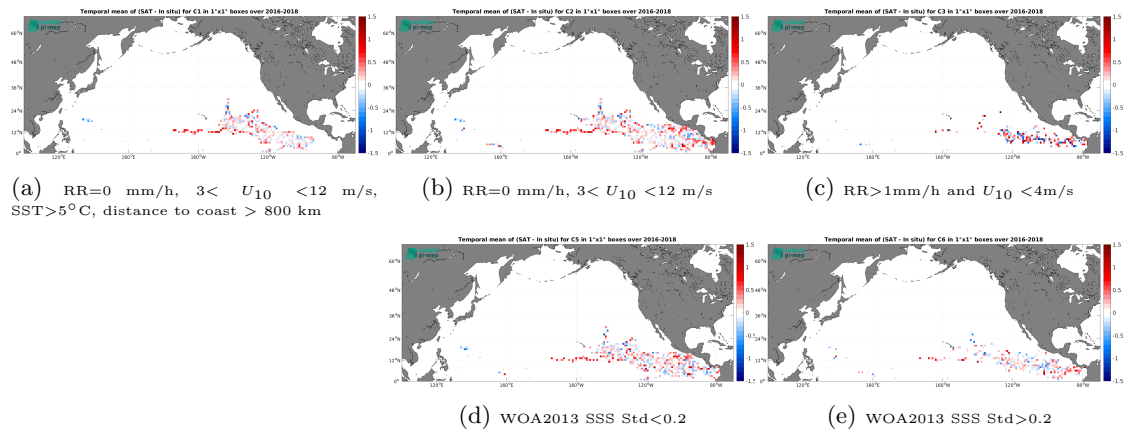
Figure 13: Temporal mean gridded over spatial boxes of size 1^\circ \times 1^\circ of \Delta SSS (SMAP SSS L2 v5.3 - 40 km (RSS) - Surface drifters) for 5 different subdatasets corresponding to:RR=0 mm/h, 3 < U_{10} < 12 m/s, SST >5^\circ\text{C} , distance to coast > 800 km (a), RR=0 mm/h, 3 < U_{10} < 12 m/s (b), RR >1 mm/h and U_{10} < 4 m/s (c), WOA2013 SSS Std <0.2 (d), WOA2013 SSS Std >0.2 (e).
