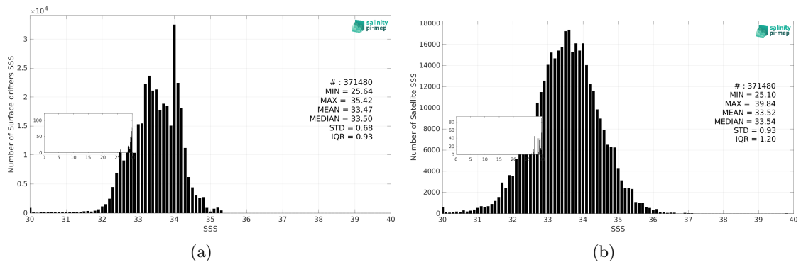
Figure 3: Histograms of SSS from Surface drifters (a) and SMAP SSS L2 v5.3 - 40 km (RSS) (b) considering all match-up pairs per bins of 0.1 over the North Pacific Ocean Pi-MEP region and for the full satellite product period.
