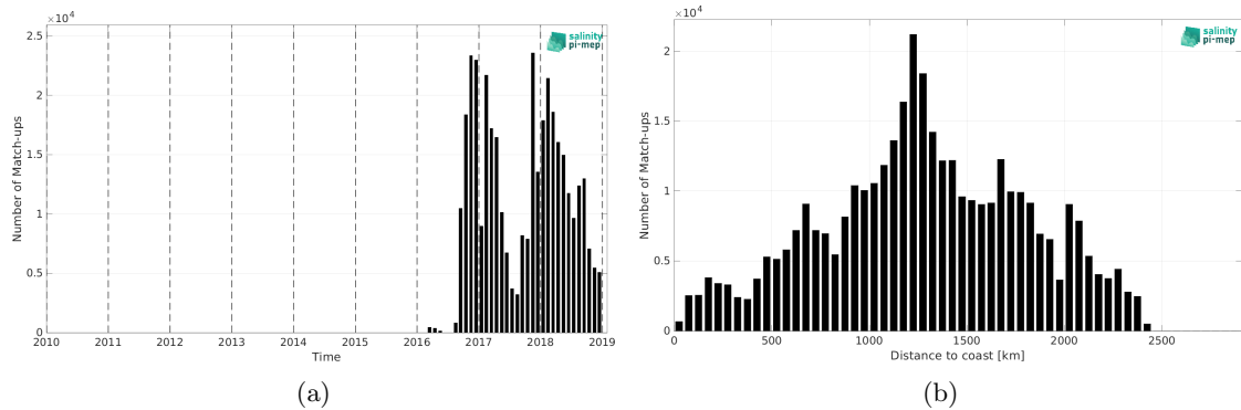
Figure 2: Number of match-ups between Surface drifters and SMAP SSS L2 v5.3 - 40 km (RSS) SSS as a function of time (a) and as function of the distance to coast (b) over the North Pacific Ocean Pi-MEP region and for the full satellite product period.
