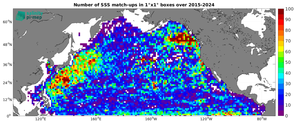
Figure 5: Number of SSS match-ups between Argo SSS and the SMAP SSS L2 v5.3 - 40 km (RSS) SSS product for the North Pacific Ocean Pi-MEP region over 1^\circ \times 1^\circ boxes and for the full satellite product period.
