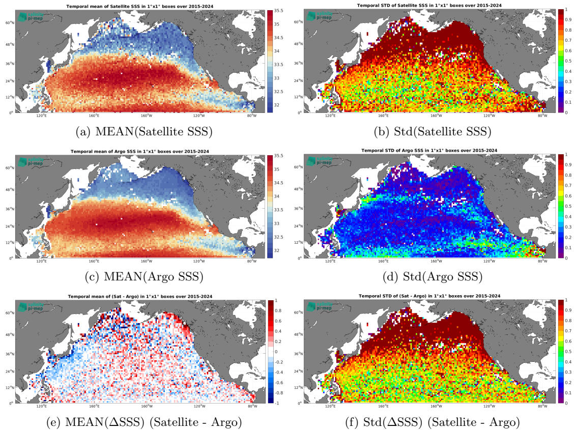
Figure 7: Temporal mean (left) and Std (right) of SSS from SMAP SSS L2 v5.3 - 40 km (RSS) (top), Argo (middle), and of \Delta SSS (Satellite - Argo). Only match-up pairs are used to generate these maps.
