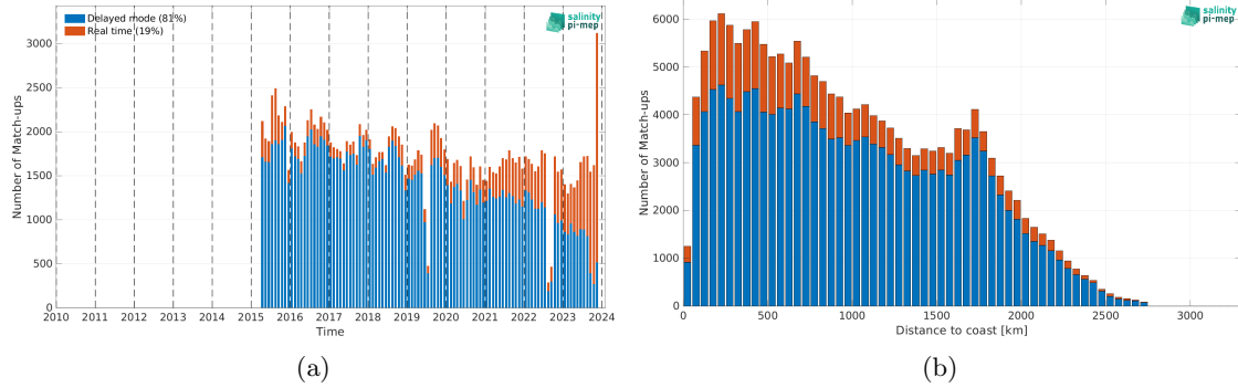
Figure 2: Number of match-ups between Argo and SMAP SSS L2 v5.3 - 40 km (RSS) SSS as a function of time (a) and as function of the distance to coast (b) over the North Pacific Ocean Pi-MEP region and for the full satellite product period.
