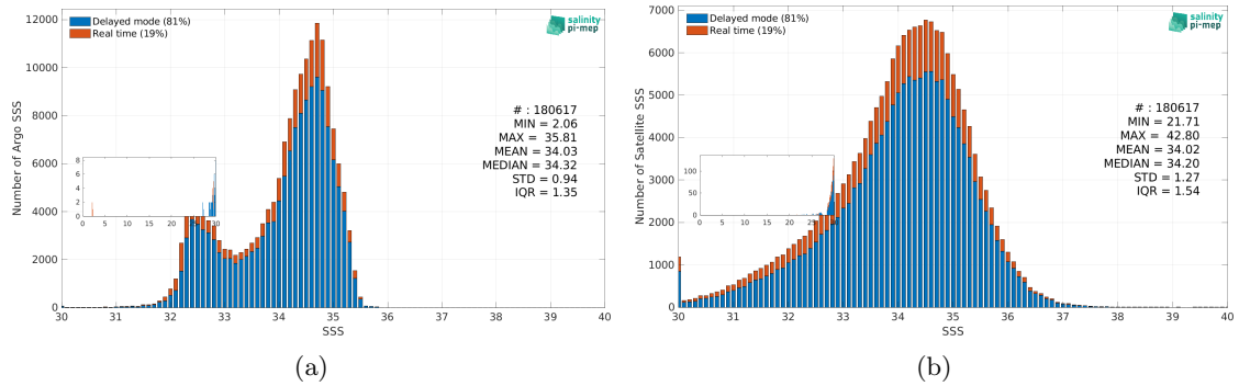
Figure 3: Histograms of SSS from Argo (a) and SMAP SSS L2 v5.3 - 40 km (RSS) (b) considering all match-up pairs per bins of 0.1 over the North Pacific Ocean Pi-MEP region and for the full satellite product period.
