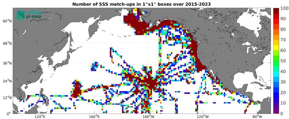
Figure 4: Number of SSS match-ups between TSG (SAMOS) SSS and the SMAP SSS L2 v5 - 40 km (RSS) SSS product for the North Pacific Ocean Pi-MEP region over 1^\circ \times 1^\circ boxes and for the full satellite product period.
