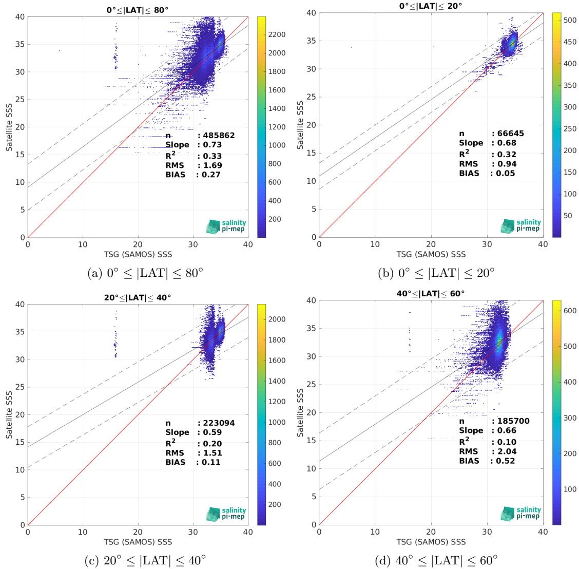
Figure 9: Contour maps of the concentration of SMAP SSS L2 v5 - 40 km (RSS) SSS (y-axis) versus TSG (SAMOS) SSS (x-axis) at match-up pairs for different latitude bands. For each plot, the red line shows x=y . The black thin and dashed lines indicate a linear fit through the data cloud and the \pm 95\% confidence levels, respectively. The number match-up pairs n , the slope and R^2 coefficient of the linear fit, the root mean square (RMS) and the mean bias between satellite and in situ data are indicated for each latitude band in each plots.
