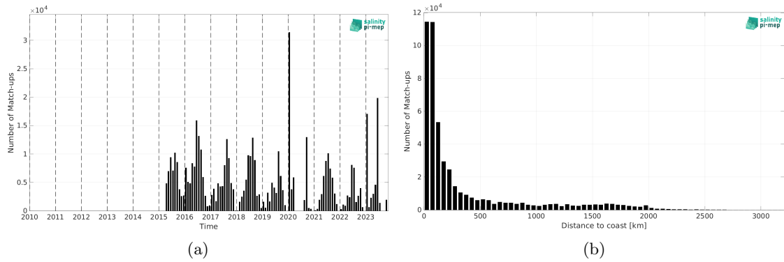
Figure 1: Number of match-ups between TSG (SAMOS) and SMAP SSS L2 v5 - 40 km (RSS) SSS as a function of time (a) and as function of the distance to coast (b) over the North Pacific Ocean Pi-MEP region and for the full satellite product period.
