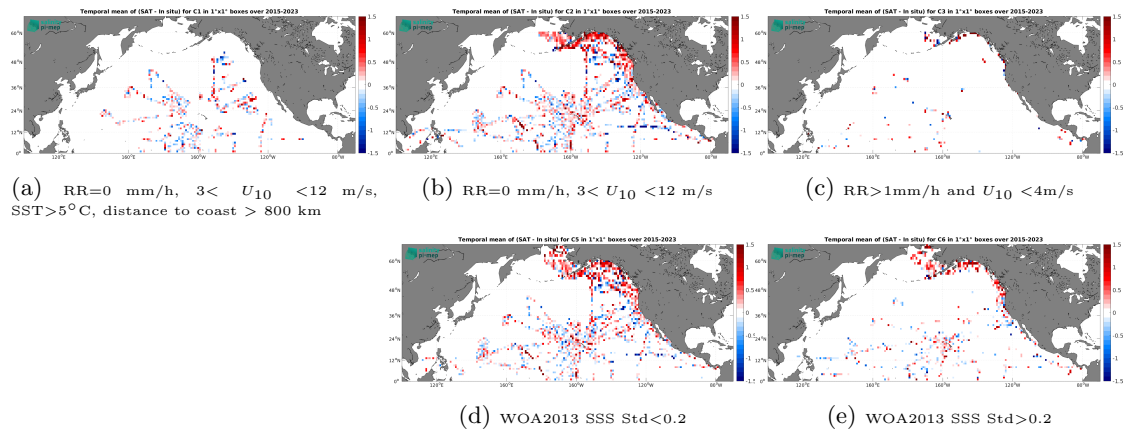
Figure 12: Temporal mean gridded over spatial boxes of size 1^\circ \times 1^\circ of \Delta SSS (SMAP SSS L2 v5 - 40 km (RSS) - TSG (SAMOS)) for 5 different subdatasets corresponding to:RR=0 mm/h, 3 < U_{10} < 12 m/s, SST > 5^\circ C , distance to coast > 800 km (a), RR=0 mm/h, 3 < U_{10} < 12 m/s (b), RR>1mm/h and U_{10} < 4 m/s (c), WOA2013 SSS Std<0.2 (d), WOA2013 SSS Std>0.2 (e).
