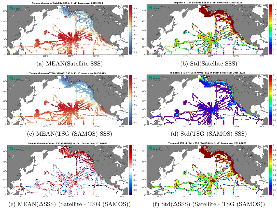
Figure 6: Temporal mean (left) and Std (right) of SSS from SMAP SSS L2 v5 - 40 km (RSS) (top), TSG (SAMOS) (middle), and of \Delta SSS (Satellite - TSG (SAMOS)). Only match-up pairs are used to generate these maps.
