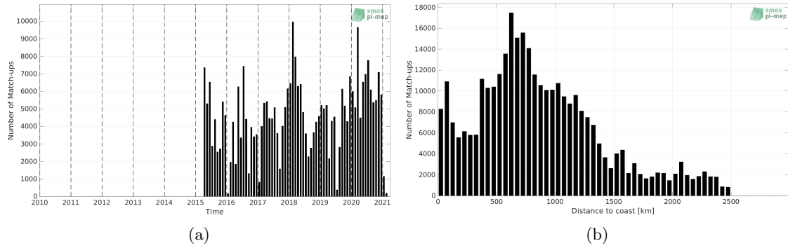
Figure 1: Number of match-ups between TSG (LEGOS-DM) and SMAP SSS L2 v5 - 40 km (RSS) SSS as a function of time (a) and as function of the distance to coast (b) over the North Pacific Ocean Pi-MEP region and for the full satellite product period.
