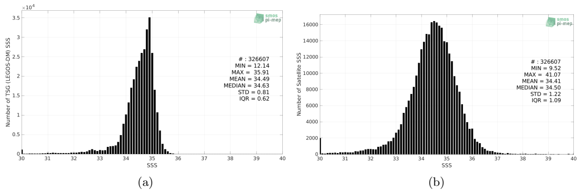
Figure 2: Histograms of SSS from TSG (LEGOS-DM) (a) and SMAP SSS L2 v5 - 40 km (RSS) (b) considering all match-up pairs per bins of 0.1 over the North Pacific Ocean Pi-MEP region and for the full satellite product period.
