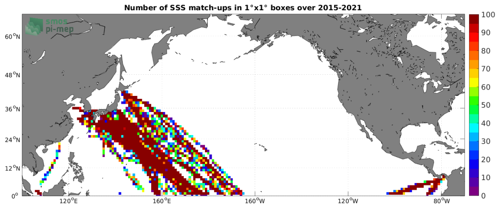
Figure 4: Number of SSS match-ups between TSG (LEGOS-DM) SSS and the SMAP SSS L2 v5 - 40 km (RSS) SSS product for the North Pacific Ocean Pi-MEP region over 1^\circ \times 1^\circ boxes and for the full satellite product period.
