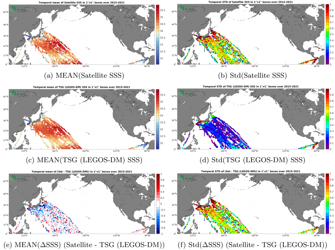
Figure 6: Temporal mean (left) and Std (right) of SSS from SMAP SSS L2 v5 - 40 km (RSS) (top), TSG (LEGOS-DM) (middle), and of \Delta SSS (Satellite - TSG (LEGOS-DM)). Only match-up pairs are used to generate these maps.
