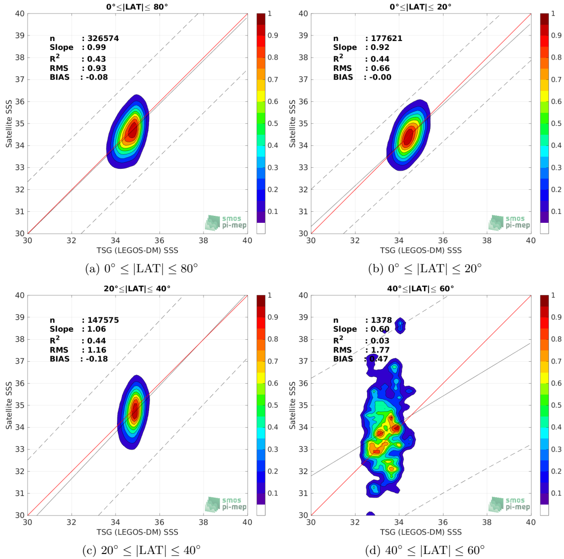
Figure 9: Contour maps of the concentration of SMAP SSS L2 v5 - 40 km (RSS) SSS (y-axis) versus TSG (LEGOS-DM) SSS (x-axis) at match-up pairs for different latitude bands. For each plot, the red line shows x=y . The black thin and dashed lines indicate a linear fit through the data cloud and the \pm 95\% confidence levels, respectively. The number match-up pairs n , the slope and R^2 coefficient of the linear fit, the root mean square (RMS) and the mean bias between satellite and in situ data are indicated for each latitude band in each plots.
