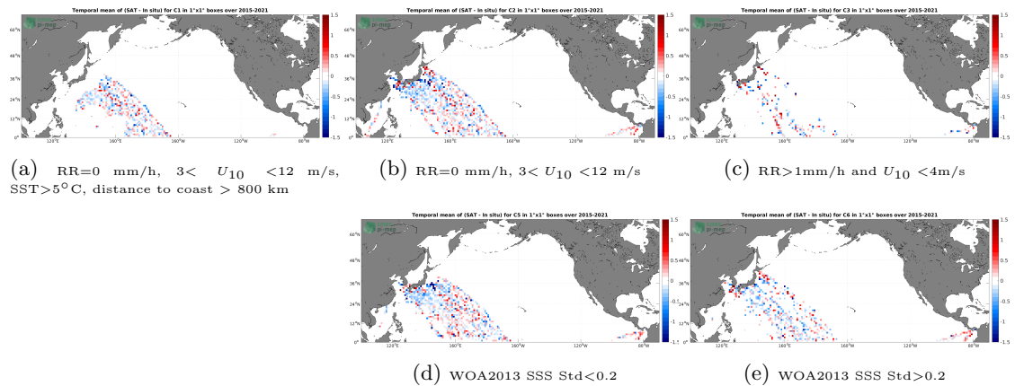
Figure 12: Temporal mean gridded over spatial boxes of size 1^\circ \times 1^\circ of \Delta SSS (SMAP SSS L2 v5 - 40 km (RSS) - TSG (LEGOS-DM)) for 5 different subdatasets corresponding to:RR=0 mm/h, 3 < U_{10} < 12 m/s, SST >5^\circ\text{C} , distance to coast > 800 km (a), RR=0 mm/h, 3 < U_{10} < 12 m/s (b), RR >1 mm/h and U_{10} < 4 m/s (c), WOA2013 SSS Std <0.2 (d), WOA2013 SSS Std >0.2 (e).
