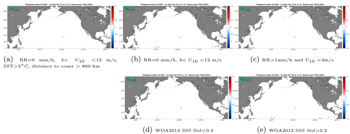
Figure 12: Temporal mean gridded over spatial boxes of size 1^\circ \times 1^\circ of \Delta\text{SSS} (SMAP SSS L2 v5 - 40 km (RSS) - TSG (GOSUD-Research-vessel)) for 5 different subdatasets corresponding to:RR=0 mm/h, 3 < U_{10} < 12 m/s, SST>5°C, distance to coast > 800 km (a), RR=0 mm/h, 3 < U_{10} < 12 m/s (b), RR>1mm/h and U_{10} < 4 m/s (c), WOA2013 SSS Std<0.2 (d), WOA2013 SSS Std>0.2 (e).
