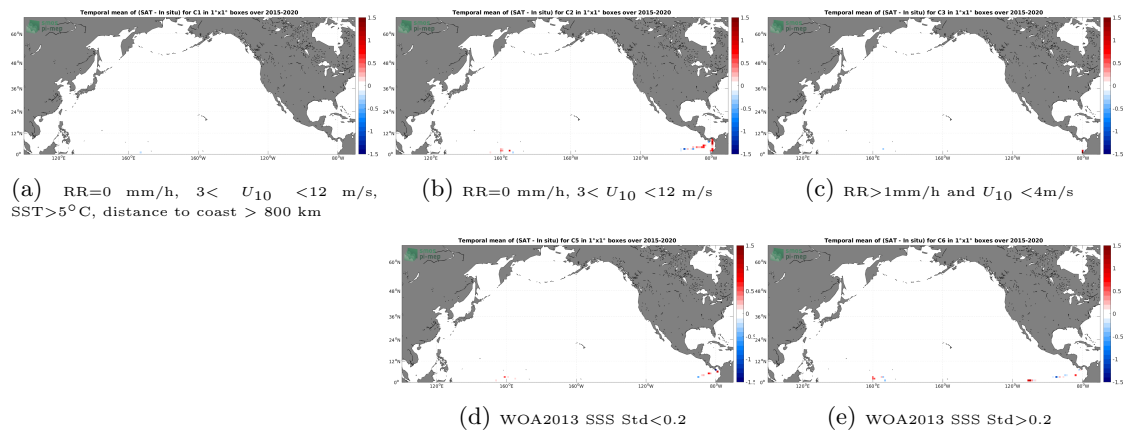
Figure 12: Temporal mean gridded over spatial boxes of size 1^\circ \times 1^\circ of \Delta SSS (SMAP SSS L2 v5 - 40 km (RSS) - TSG (GOSUD-Research-vessel)) for 5 different subdatasets corresponding to: RR=0 mm/h, 3 < U_{10} < 12 m/s, SST > 5°C, distance to coast > 800 km (a), RR=0 mm/h, 3 < U_{10} < 12 m/s (b), RR > 1 mm/h and U_{10} < 4 m/s (c), WOA2013 SSS Std < 0.2 (d), WOA2013 SSS Std > 0.2 (e).
