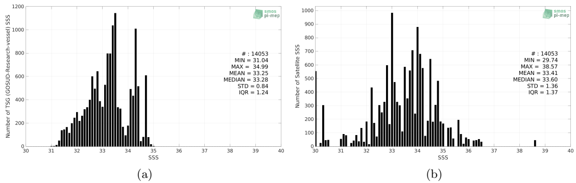
Figure 2: Histograms of SSS from TSG (GOSUD-Research-vessel) (a) and SMAP SSS L2 v5 - 40 km (RSS) (b) considering all match-up pairs per bins of 0.1 over the North Pacific Ocean Pi-MEP region and for the full satellite product period.
