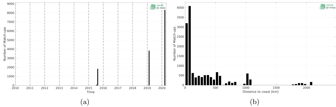
Figure 1: Number of match-ups between TSG (GOSUD-Research-vessel) and SMAP SSS L2 v5 - 40 km (RSS) SSS as a function of time (a) and as function of the distance to coast (b) over the North Pacific Ocean Pi-MEP region and for the full satellite product period.
