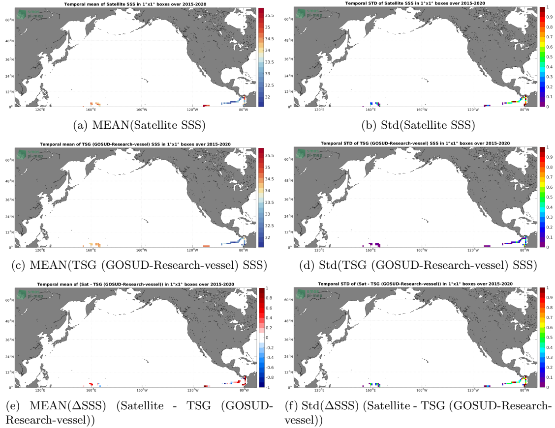
Figure 6: Temporal mean (left) and Std (right) of SSS from SMAP SSS L2 v5 - 40 km (RSS) (top), TSG (GOSUD-Research-vessel) (middle), and of \Delta SSS (Satellite - TSG (GOSUD-Research-vessel)). Only match-up pairs are used to generate these maps.
