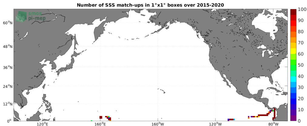
Figure 4: Number of SSS match-ups between TSG (GOSUD-Research-vessel) SSS and the SMAP SSS L2 v5 - 40 km (RSS) SSS product for the North Pacific Ocean Pi-MEP region over 1^\circ \times 1^\circ boxes and for the full satellite product period.
