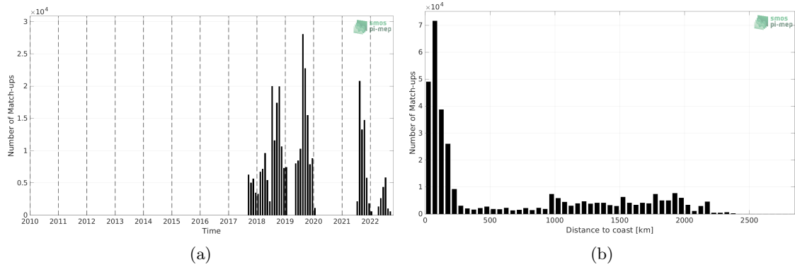
Figure 1: Number of match-ups between Saildrone and SMAP SSS L2 v5 - 40 km (RSS) SSS as a function of time (a) and as function of the distance to coast (b) over the North Pacific Ocean Pi-MEP region and for the full satellite product period.
