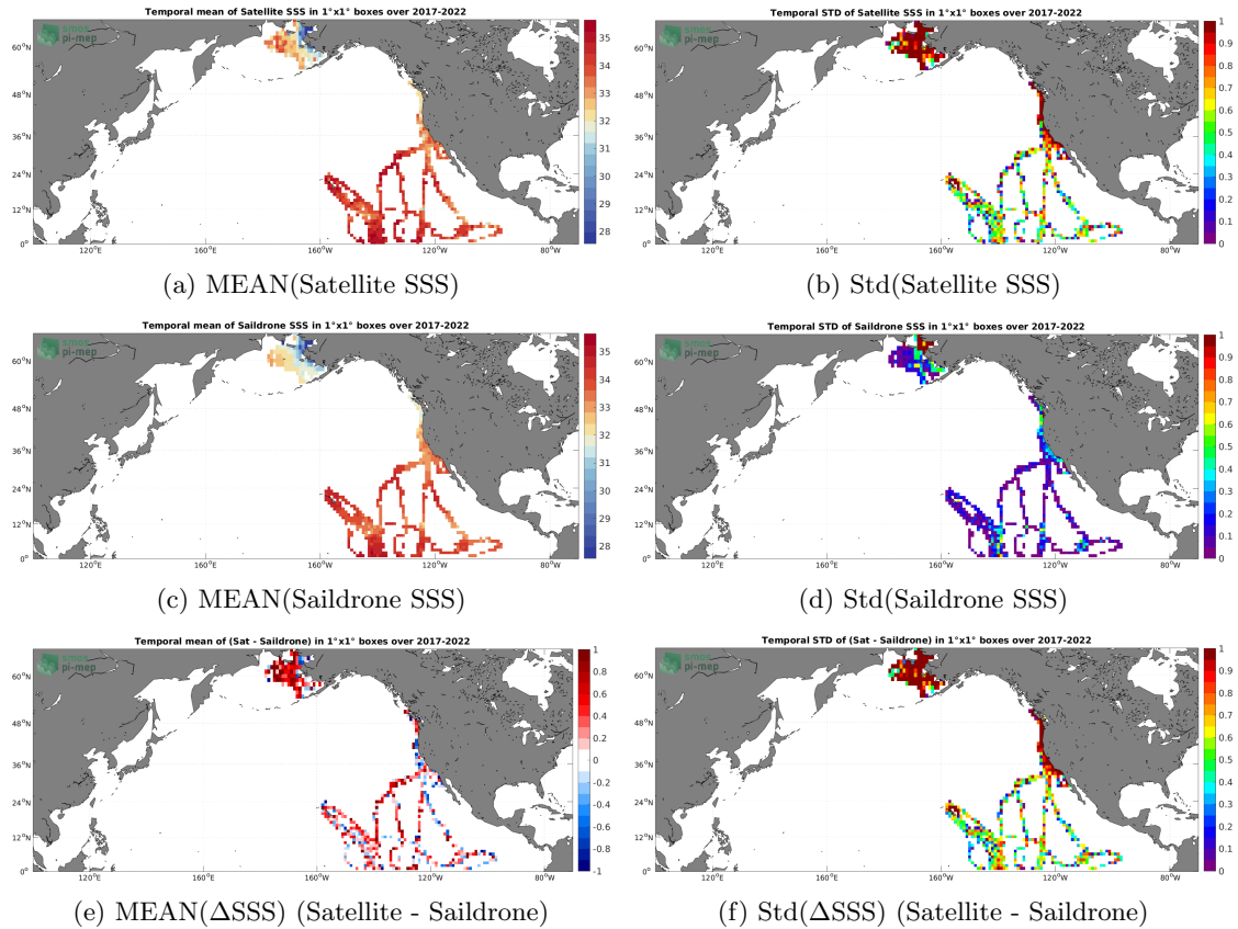
Figure 6: Temporal mean (left) and Std (right) of SSS from SMAP SSS L2 v5 - 40 km (RSS) (top), Saildrone (middle), and of \Delta SSS (Satellite - Saildrone). Only match-up pairs are used to generate these maps.
