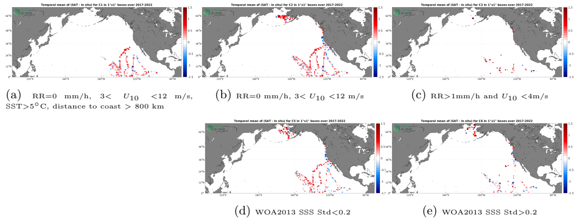
Figure 12: Temporal mean gridded over spatial boxes of size 1^\circ \times 1^\circ of \Delta SSS (SMAP SSS L2 v5 - 40 km (RSS) - Sairdrone) for 5 different subdatasets corresponding to:RR=0 mm/h, 3 < U_{10} < 12 m/s, SST >5^\circ\text{C} , distance to coast > 800 km (a), RR=0 mm/h, 3 < U_{10} < 12 m/s (b), RR >1 mm/h and U_{10} < 4 m/s (c), WOA2013 SSS Std <0.2 (d), WOA2013 SSS Std >0.2 (e).
