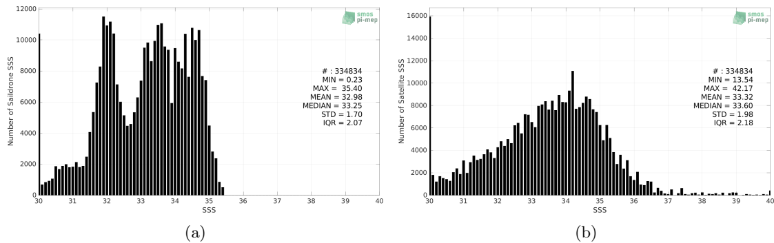
Figure 2: Histograms of SSS from Saildrone (a) and SMAP SSS L2 v5 - 40 km (RSS) (b) considering all match-up pairs per bins of 0.1 over the North Pacific Ocean Pi-MEP region and for the full satellite product period.
