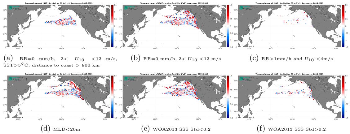
Figure 12: Temporal mean gridded over spatial boxes of size 1^\circ \times 1^\circ of \Delta SSS (SMAP SSS L2 v5 - 40 km (RSS) - Marine mammals) for 6 different subdatasets corresponding to:RR=0 mm/h, 3 < U_{10} < 12 m/s, SST >5^\circ\text{C} , distance to coast > 800 km (a), RR=0 mm/h, 3 < U_{10} < 12 m/s (b), RR >1 mm/h and U_{10} < 4 m/s (c),MLD <20 m (d),WOA2013 SSS Std <0.2 (e),WOA2013 SSS Std >0.2 (f).
