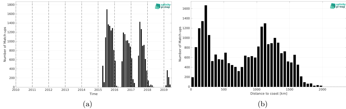
Figure 1: Number of match-ups between Marine mammals and SMAP SSS L2 v5 - 40 km (RSS) SSS as a function of time (a) and as function of the distance to coast (b) over the North Pacific Ocean Pi-MEP region and for the full satellite product period.
