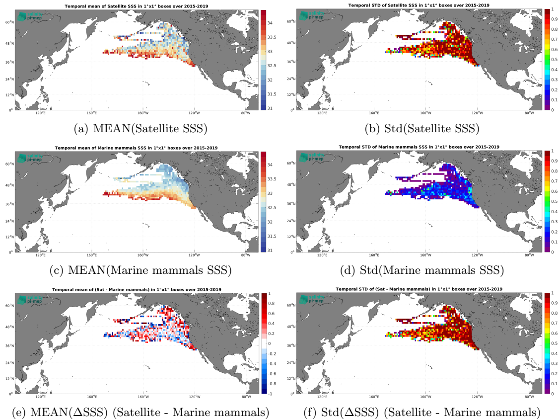
Figure 6: Temporal mean (left) and Std (right) of SSS from SMAP SSS L2 v5 - 40 km (RSS) (top), Marine mammals (middle), and of \Delta SSS (Satellite - Marine mammals). Only match-up pairs are used to generate these maps.
