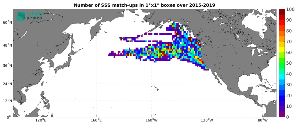
Figure 4: Number of SSS match-ups between Marine mammals SSS and the SMAP SSS L2 v5 - 40 km (RSS) SSS product for the North Pacific Ocean Pi-MEP region over 1^\circ \times 1^\circ boxes and for the full satellite product period.
