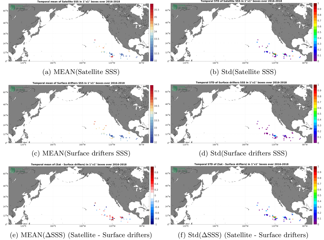
Figure 5: Temporal mean (left) and Std (right) of SSS from SMAP SSS L2 v5 - 40 km (RSS) (top), Surface drifters (middle), and of \Delta SSS (Satellite - Surface drifters). Only match-up pairs are used to generate these maps.
