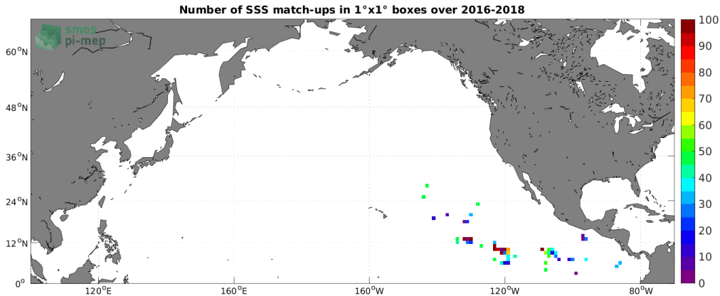
Figure 3: Number of SSS match-ups between Surface drifters SSS and the SMAP SSS L2 v5 - 40 km (RSS) SSS product for the North Pacific Ocean Pi-MEP region over 1^\circ \times 1^\circ boxes and for the full satellite product period.
