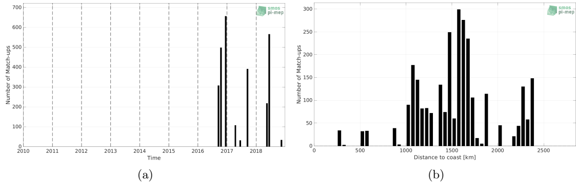
Figure 1: Number of match-ups between Surface drifters and SMAP SSS L2 v5 - 40 km (RSS) SSS as a function of time (a) and as function of the distance to coast (b) over the North Pacific Ocean Pi-MEP region and for the full satellite product period.
