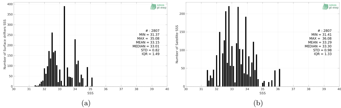
Figure 2: Histograms of SSS from Surface drifters (a) and SMAP SSS L2 v5 - 40 km (RSS) (b) considering all match-up pairs per bins of 0.1 over the North Pacific Ocean Pi-MEP region and for the full satellite product period.
