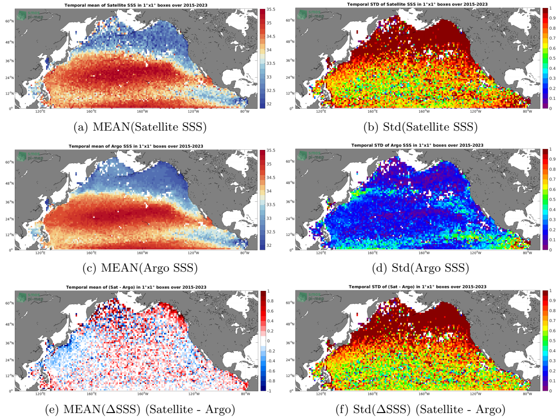
Figure 6: Temporal mean (left) and Std (right) of SSS from SMAP SSS L2 v5 - 40 km (RSS) (top), Argo (middle), and of \Delta SSS (Satellite - Argo). Only match-up pairs are used to generate these maps.
