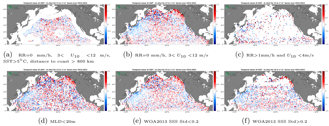
Figure 12: Temporal mean gridded over spatial boxes of size 1^\circ \times 1^\circ of \Delta SSS (SMAP SSS L2 v5 - 40 km (RSS) - Argo) for 6 different subdatasets corresponding to:RR=0 mm/h, 3 < U_{10} < 12 m/s, SST >5^\circ C, distance to coast > 800 km (a), RR=0 mm/h, 3 < U_{10} < 12 m/s (b), RR >1 mm/h and U_{10} < 4 m/s (c),MLD <20 m (d),WOA2013 SSS Std <0.2 (e),WOA2013 SSS Std >0.2 (f).
