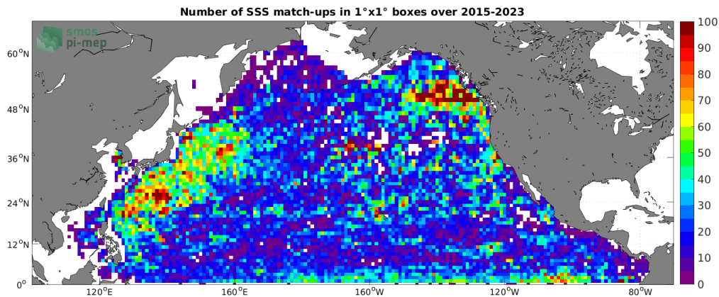
Figure 4: Number of SSS match-ups between Argo SSS and the SMAP SSS L2 v5 - 40 km (RSS) SSS product for the North Pacific Ocean Pi-MEP region over 1^\circ \times 1^\circ boxes and for the full satellite product period.
