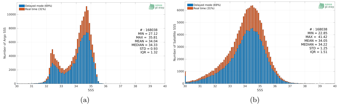
Figure 2: Histograms of SSS from Argo (a) and SMAP SSS L2 v5 - 40 km (RSS) (b) considering all match-up pairs per bins of 0.1 over the North Pacific Ocean Pi-MEP region and for the full satellite product period.
