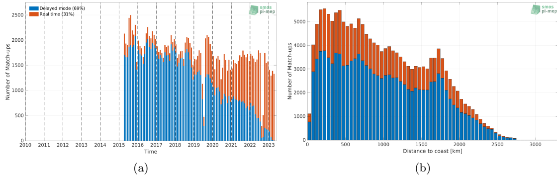
Figure 1: Number of match-ups between Argo and SMAP SSS L2 v5 - 40 km (RSS) SSS as a function of time (a) and as function of the distance to coast (b) over the North Pacific Ocean Pi-MEP region and for the full satellite product period.
