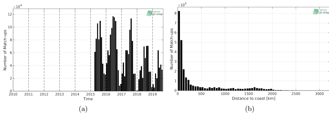
Figure 1: Number of match-ups between TSG-SAMOS and SMAP-L2-RSS-V4 SSS as a function of time (a) and as function of the distance to coast (b) over the North Pacific Ocean Pi-MEP region and for the full satellite product period.
