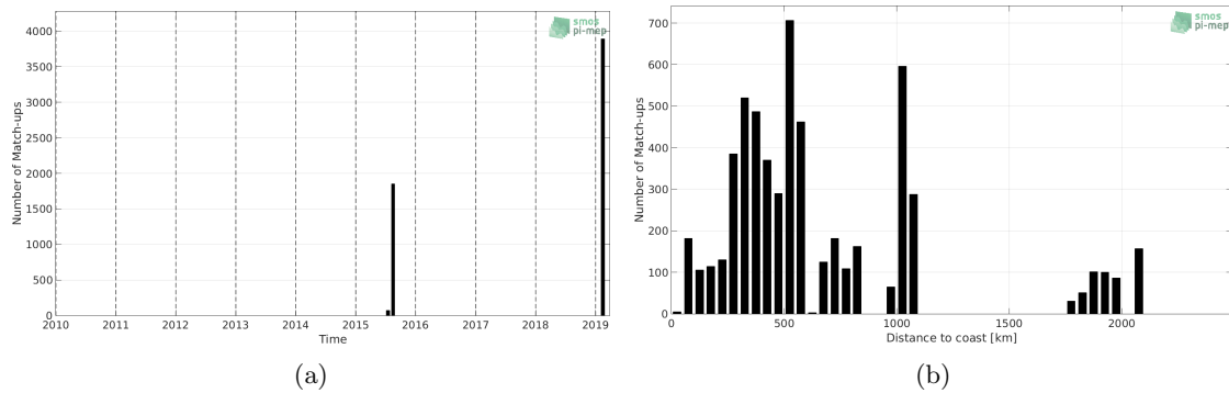
Figure 1: Number of match-ups between TSG (GOSUD-Research-vessel) and SMAP SSS L2 v4 (RSS) SSS as a function of time (a) and as function of the distance to coast (b) over the North Pacific Ocean Pi-MEP region and for the full satellite product period.
