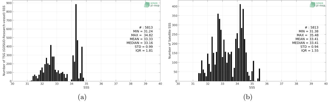
Figure 2: Histograms of SSS from TSG (GOSUD-Research-vessel) (a) and SMAP SSS L2 v4 (RSS) (b) considering all match-up pairs per bins of 0.1 over the North Pacific Ocean Pi-MEP region and for the full satellite product period.
