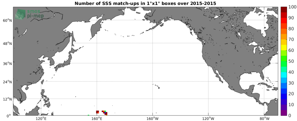
Figure 4: Number of SSS match-ups between TSG-GOSUD-Research-vessel SSS and the SMAP-L2-RSS-V4 SSS product for the North Pacific Ocean Pi-MEP region over 1^\circ \times 1^\circ boxes and for the full satellite product period.
