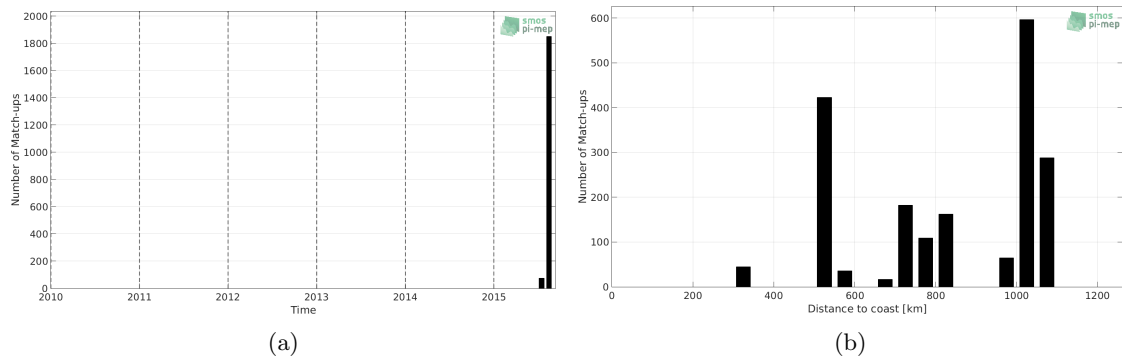
Figure 1: Number of match-ups between TSG-GOSUD-Research-vessel and SMAP-L2-RSS-V4 SSS as a function of time (a) and as function of the distance to coast (b) over the North Pacific Ocean Pi-MEP region and for the full satellite product period.
