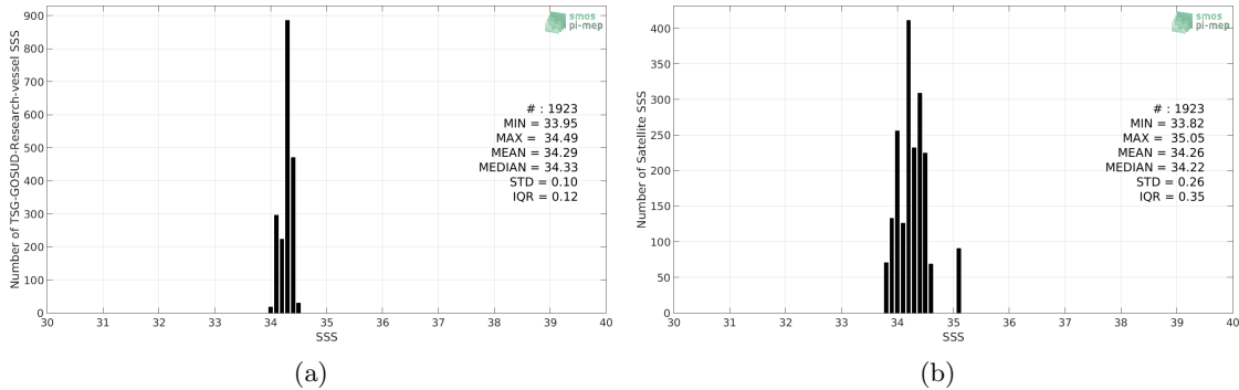
Figure 2: Histograms of SSS from TSG-GOSUD-Research-vessel (a) and SMAP-L2-RSS-V4 (b) considering all match-up pairs per bins of 0.1 over the North Pacific Ocean Pi-MEP region and for the full satellite product period.
