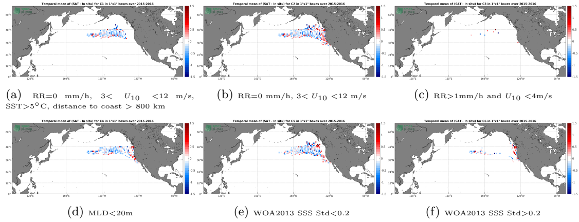
Figure 12: Temporal mean gridded over spatial boxes of size 1^\circ \times 1^\circ of \Delta SSS (SMAP SSS L2 v4 (RSS) - Sea mammals) for 6 different subdatasets corresponding to: RR=0 mm/h, 3 < U_{10} < 12 m/s, SST > 5^\circ C , distance to coast > 800 km (a), RR=0 mm/h, 3 < U_{10} < 12 m/s (b), RR > 1 mm/h and U_{10} < 4 m/s (c), MLD < 20 m (d), WOA2013 SSS Std < 0.2 (e), WOA2013 SSS Std > 0.2 (f).
