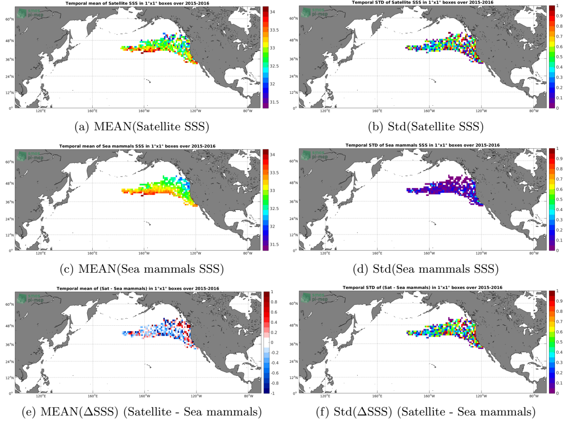
Figure 6: Temporal mean (left) and Std (right) of SSS from SMAP SSS L2 v4 (RSS) (top), Sea mammals (middle), and of \Delta SSS (Satellite - Sea mammals). Only match-up pairs are used to generate these maps.
