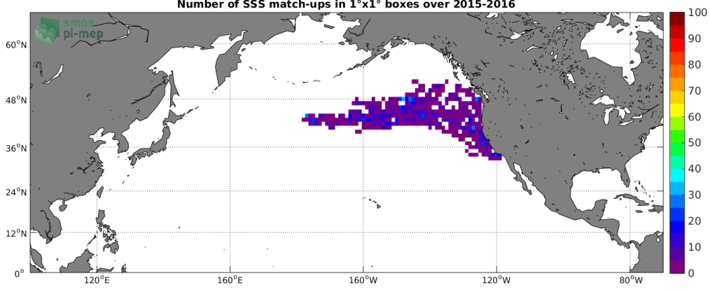
Figure 4: Number of SSS match-ups between Sea mammals SSS and the SMAP SSS L2 v4 (RSS) SSS product for the North Pacific Ocean Pi-MEP region over 1^\circ \times 1^\circ boxes and for the full satellite product period.
