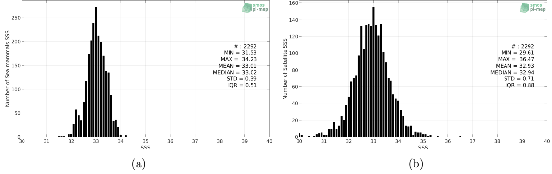
Figure 2: Histograms of SSS from Sea mammals (a) and SMAP SSS L2 v4 (RSS) (b) considering all match-up pairs per bins of 0.1 over the North Pacific Ocean Pi-MEP region and for the full satellite product period.
