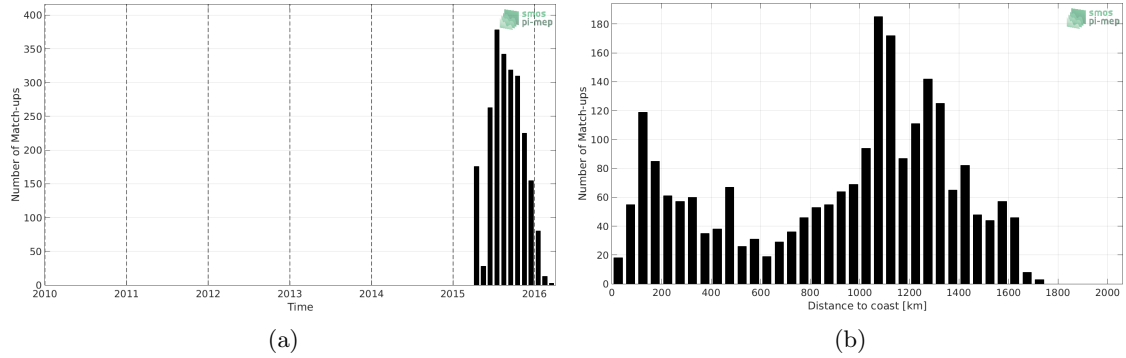
Figure 1: Number of match-ups between Sea mammals and SMAP SSS L2 v4 (RSS) SSS as a function of time (a) and as function of the distance to coast (b) over the North Pacific Ocean Pi-MEP region and for the full satellite product period.
