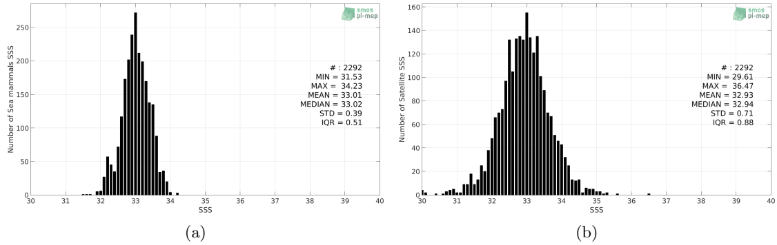
Figure 2: Histograms of SSS from Sea mammals (a) and SMAP-L2-RSS-V4 (b) considering all match-up pairs per bins of 0.1 over the North Pacific Ocean Pi-MEP region and for the full satellite product period.
