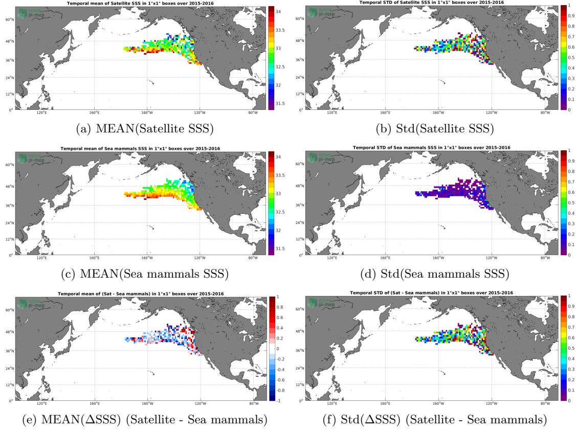
Figure 6: Temporal mean (left) and Std (right) of SSS from SMAP-L2-RSS-V4 (top), Sea mammals (middle), and of \Delta SSS (Satellite - Sea mammals). Only match-up pairs are used to generate these maps.
