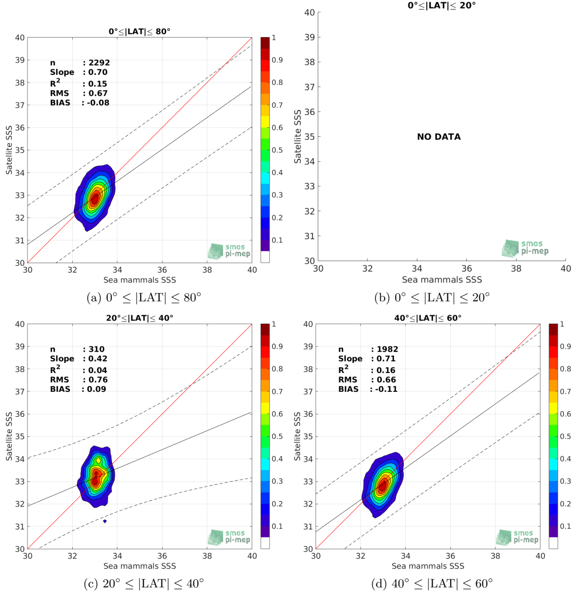
Figure 9: Contour maps of the concentration of SMAP-L2-RSS-V4 SSS (y-axis) versus Sea mammals SSS (x-axis) at match-up pairs for different latitude bands. For each plot, the red line shows x=y . The black thin and dashed lines indicate a linear fit through the data cloud and the \pm 95\% confidence levels, respectively. The number match-up pairs n , the slope and R^2 coefficient of the linear fit, the root mean square (RMS) and the mean bias between satellite and in situ data are indicated for each latitude band in each plots.
