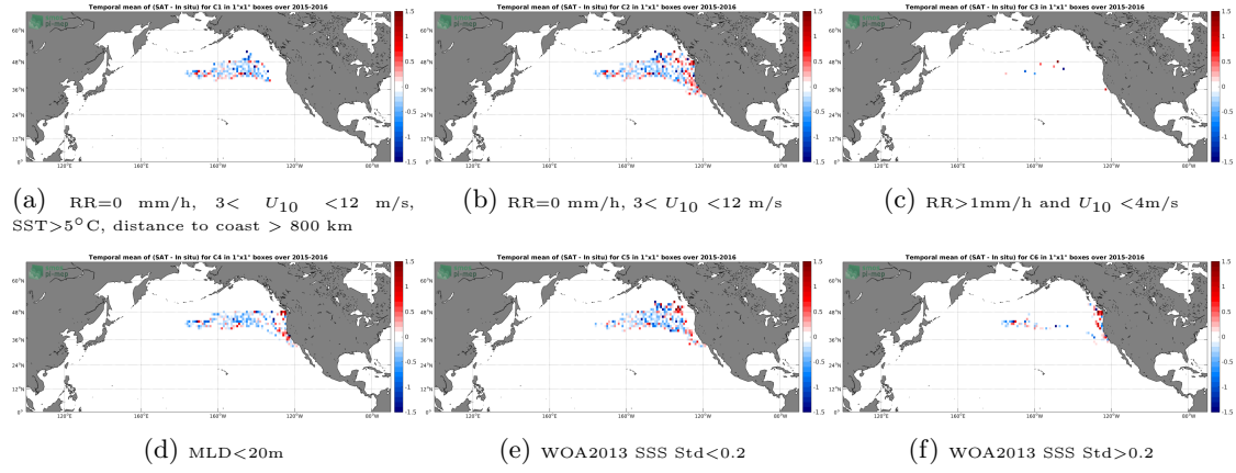
Figure 12: Temporal mean gridded over spatial boxes of size 1^\circ \times 1^\circ of \Delta SSS (SMAP-L2-RSS-V4 - Sea mammals) for 6 different subdatasets corresponding to: RR=0 mm/h, 3 < U_{10} < 12 m/s, SST >5^\circ\text{C} , distance to coast > 800 km (a), RR=0 mm/h, 3 < U_{10} < 12 m/s (b), RR>1\text{mm/h} and U_{10} < 4\text{m/s} (c), MLD <20\text{m} (d), WOA2013 SSS Std <0.2 (e), WOA2013 SSS Std >0.2 (f).
