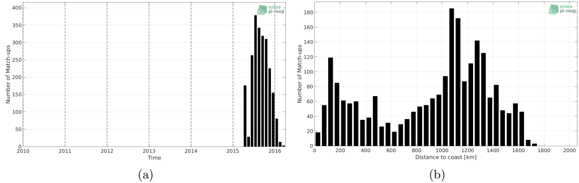
Figure 1: Number of match-ups between Sea mammals and SMAP-L2-RSS-V4 SSS as a function of time (a) and as function of the distance to coast (b) over the North Pacific Ocean Pi-MEP region and for the full satellite product period.
