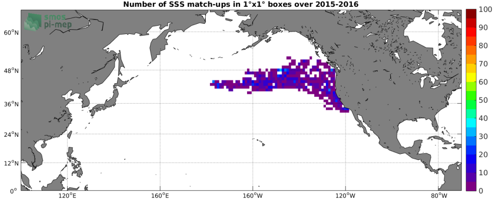
Figure 4: Number of SSS match-ups between Sea mammals SSS and the SMAP-L2-RSS-V4 SSS product for the North Pacific Ocean Pi-MEP region over 1^\circ \times 1^\circ boxes and for the full satellite product period.
