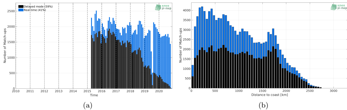
Figure 1: Number of match-ups between Argo and SMAP SSS L2 v4 (RSS) SSS as a function of time (a) and as function of the distance to coast (b) over the North Pacific Ocean Pi-MEP region and for the full satellite product period.
