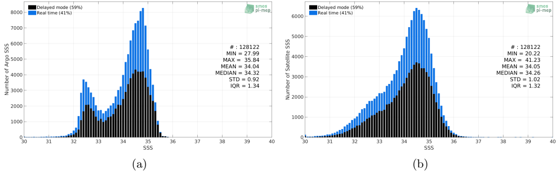
Figure 2: Histograms of SSS from Argo (a) and SMAP SSS L2 v4 (RSS) (b) considering all match-up pairs per bins of 0.1 over the North Pacific Ocean Pi-MEP region and for the full satellite product period.
