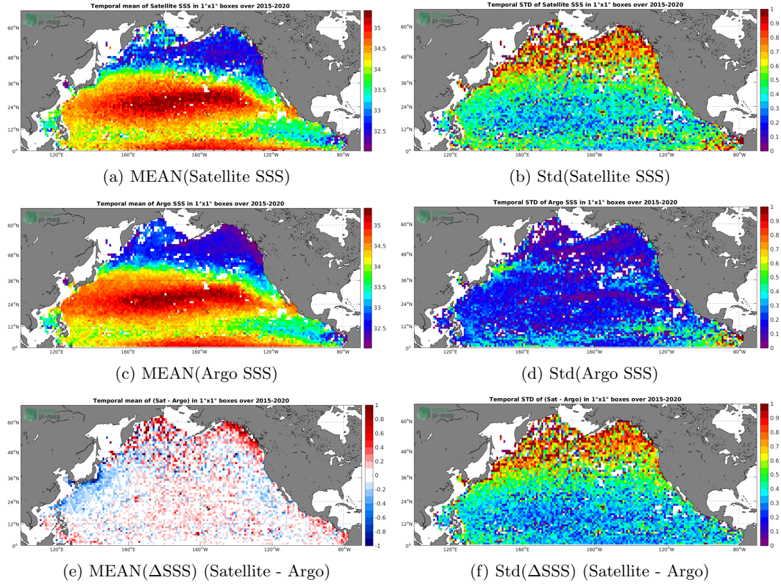
Figure 6: Temporal mean (left) and Std (right) of SSS from SMAP SSS L2 v4 (RSS) (top), Argo (middle), and of \Delta SSS (Satellite - Argo). Only match-up pairs are used to generate these maps.
