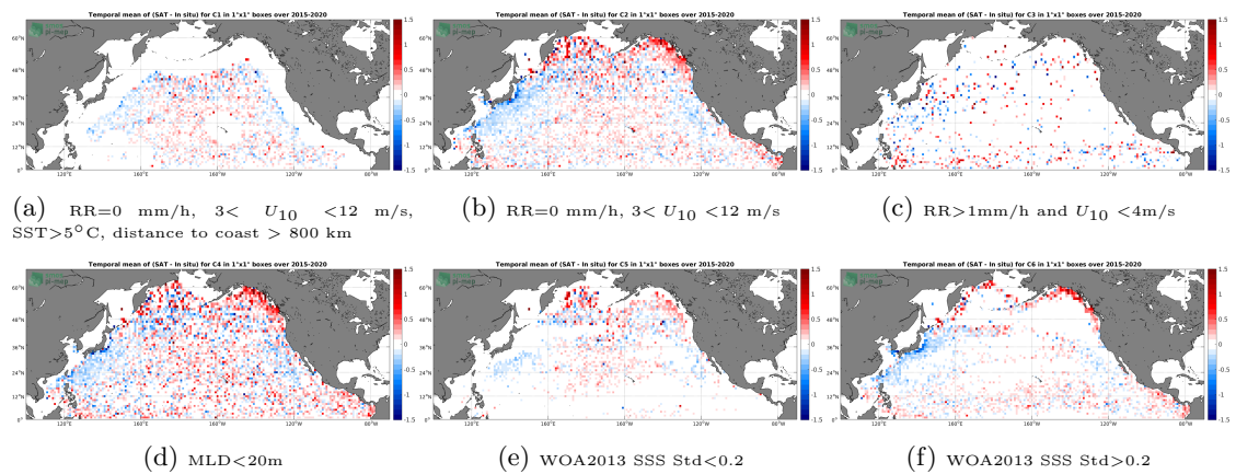
Figure 12: Temporal mean gridded over spatial boxes of size 1^\circ \times 1^\circ of \Delta SSS (SMAP SSS L2 v4 (RSS) - Argo) for 6 different subdatasets corresponding to:RR=0 mm/h, 3 < U_{10} < 12 m/s, SST >5^\circ C, distance to coast > 800 km (a), RR=0 mm/h, 3 < U_{10} < 12 m/s (b), RR >1 mm/h and U_{10} < 4 m/s (c),MLD <20 m (d),WOA2013 SSS Std <0.2 (e),WOA2013 SSS Std >0.2 (f).
