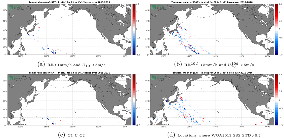
Figure 12: Temporal mean gridded over spatial boxes of size 1^\circ \times 1^\circ of \Delta SSS (SMAP-L2-RSS-V3-70KM - TSG-LEGOS-DM) for 4 different subdatasets corresponding to: RR > 1mm/h and U_{10} < 5\text{m/s} (a), RR^{10d} > 5\text{mm/h} and U_{10}^{10d} < 5\text{m/s} (b), C1 U C2 (c), Locations where WOA2013 SSS STD > 0.2 (d).
