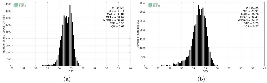
Figure 2: Histograms of SSS from TSG-LEGOS-DM (a) and SMAP-L2-RSS-V3-70KM (b) considering all match-up pairs per bins of 0.1 over the North Pacific Ocean Pi-MEP region and for the full satellite product period.
