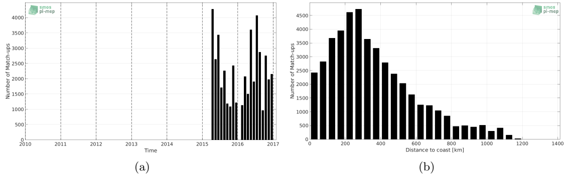
Figure 1: Number of match-ups between TSG-LEGOS-DM and SMAP-L2-RSS-V3-70KM SSS as a function of time (a) and as function of the distance to coast (b) over the North Pacific Ocean Pi-MEP region and for the full satellite product period.
