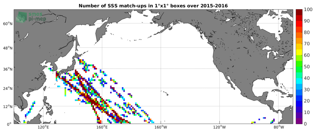
Figure 4: Number of SSS match-ups between TSG-LEGOS-DM SSS and the SMAP-L2-RSS-V3-70KM SSS product for the North Pacific Ocean Pi-MEP region over 1^\circ \times 1^\circ boxes and for the full satellite product period.
