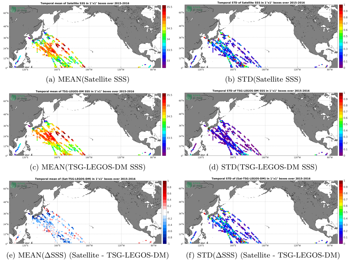
Figure 6: Temporal mean (left) and STD (right) of SSS from SMAP-L2-RSS-V3-70KM (top), TSG-LEGOS-DM (middle), and of \Delta SSS (Satellite - TSG-LEGOS-DM). Only match-up pairs are used to generate these maps.
