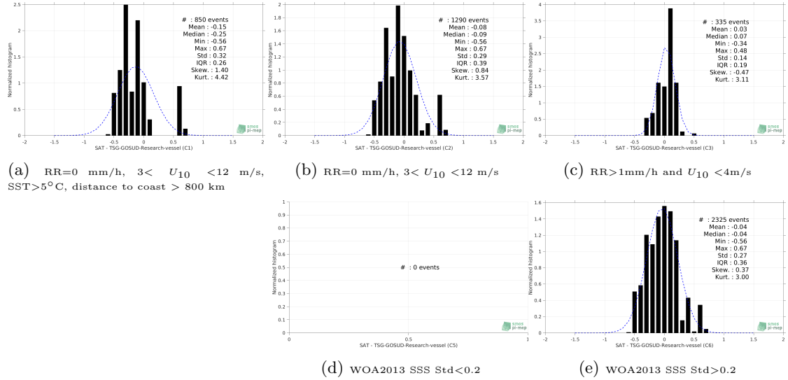
Figure 13: Normalized histogram of \Delta SSS (SMAP-L2-RSS-V3-70KM - TSG-GOSUD-Research-vessel) for 5 different subdatasets corresponding to: RR=0 mm/h, 3 < U_{10} < 12 m/s, SST>5°C, distance to coast > 800 km (a), RR=0 mm/h, 3 < U_{10} < 12 m/s (b), RR>1mm/h and U_{10} < 4 m/s (c), WOA2013 SSS Std<0.2 (d), WOA2013 SSS Std>0.2 (e).
