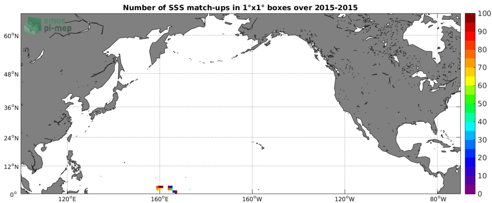
Figure 4: Number of SSS match-ups between TSG-GOSUD-Research-vessel SSS and the SMAP-L2-RSS-V3-70KM SSS product for the North Pacific Ocean Pi-MEP region over 1^\circ \times 1^\circ boxes and for the full satellite product period.
