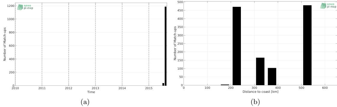
Figure 1: Number of match-ups between TSG-GOSUD-Research-vessel and SMAP-L2-RSS-V3-70KM SSS as a function of time (a) and as function of the distance to coast (b) over the North Pacific Ocean Pi-MEP region and for the full satellite product period.
