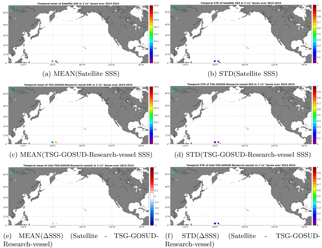
Figure 6: Temporal mean (left) and STD (right) of SSS from SMAP-L2-RSS-V3-70KM (top), TSG-GOSUD-Research-vessel (middle), and of \Delta SSS (Satellite - TSG-GOSUD-Research-vessel). Only match-up pairs are used to generate these maps.
