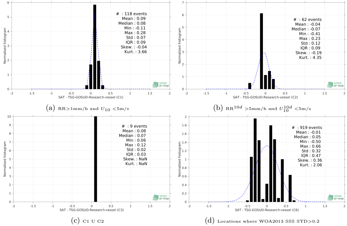
Figure 13: Normalized histogram of \Delta\text{SSS} (SMAP-L2-RSS-V3-70KM - TSG-GOSUD-Research-vessel) for 6 different subdatasets corresponding to: RR > 1mm/h and U_{10} < 5\text{m/s} (a), RR^{10d} > 5\text{mm/h} and U_{10}^{10d} < 5\text{m/s} (b), C1 U C2 (c), Locations where WOA2013 SSS STD > 0.2 (d).
