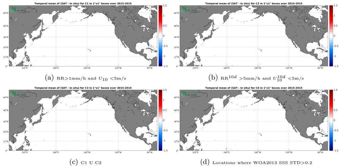
Figure 12: Temporal mean gridded over spatial boxes of size 1^\circ \times 1^\circ of \Delta SSS (SMAP-L2-RSS-V3-70KM - TSG-GOSUD-Research-vessel) for 4 different subdatasets corresponding to: RR > 1\text{mm/h} and U_{10} < 5\text{m/s} (a), RR^{10d} > 5\text{mm/h} and U_{10}^{10d} < 5\text{m/s} (b), C1 U C2 (c), Locations where WOA2013 SSS STD > 0.2 (d).
