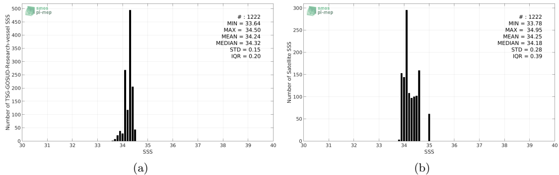
Figure 2: Histograms of SSS from TSG-GOSUD-Research-vessel (a) and SMAP-L2-RSS-V3-70KM (b) considering all match-up pairs per bins of 0.1 over the North Pacific Ocean Pi-MEP region and for the full satellite product period.
